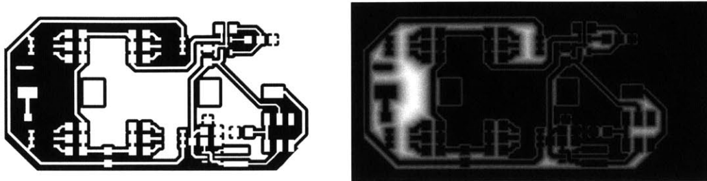
Figure 6-6: Original model and distance transform
