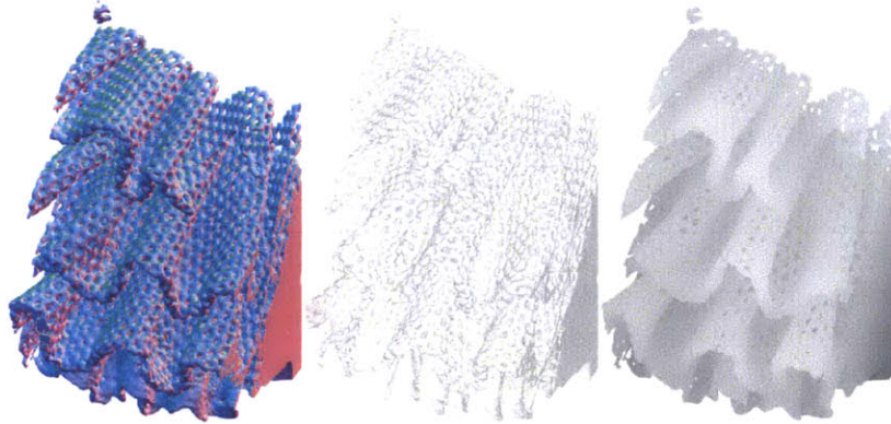
Figure 5-1: CT scanned lace (normals, shaded, and height-map)
