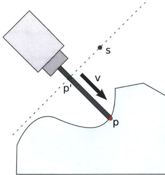
Figure 6-20: Safe plane for angled cuts
