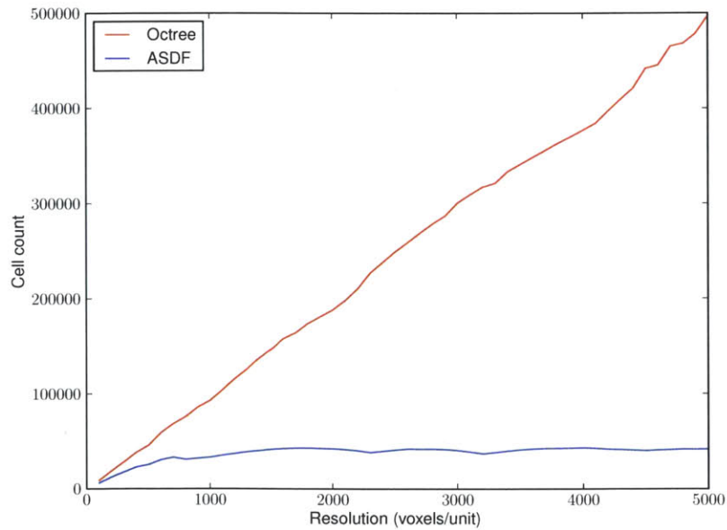
Figure 2-4: Cell count in octree and ASDF
