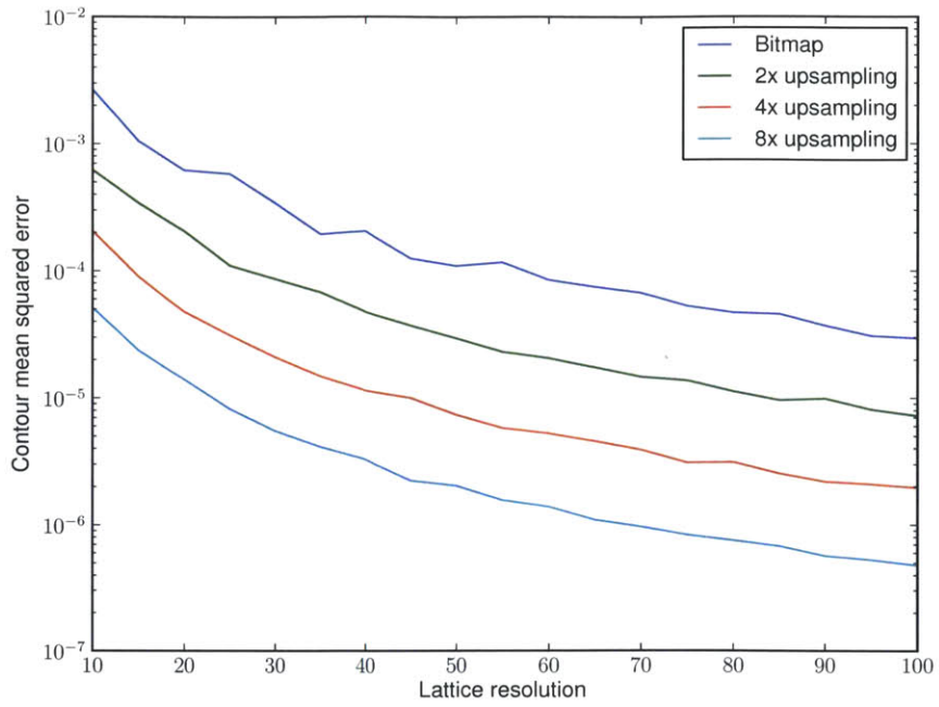
Figure 6-4: Mean squared errors in circle contours
