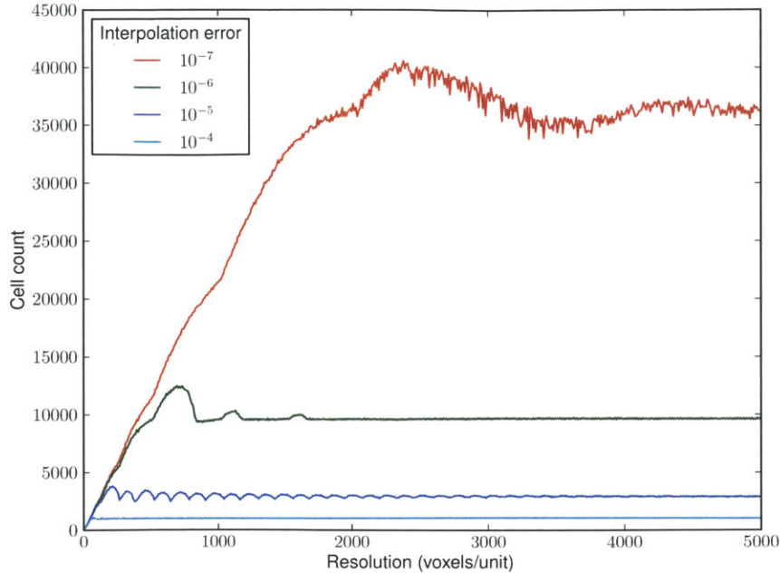
Figure 2-5: Number of cells defining circle
