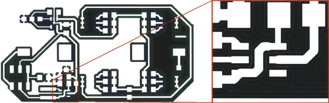
Figure 6-13: Contour cuts on a PCB bitmap
