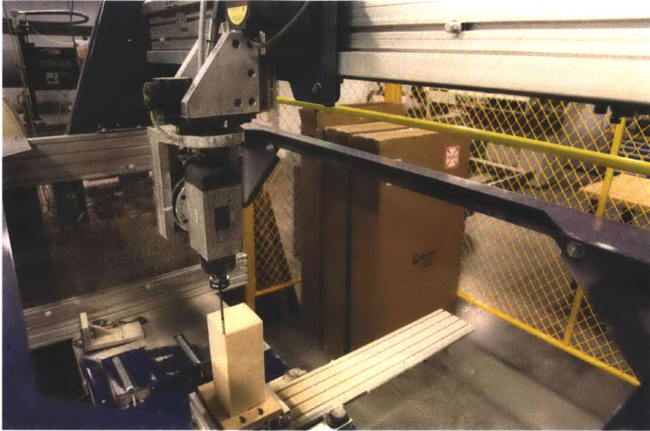
Figure 6-19: Shopbot 5-axis
