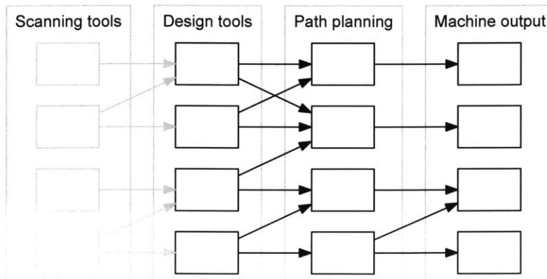
Figure 1-1: Combinatorial explosion
