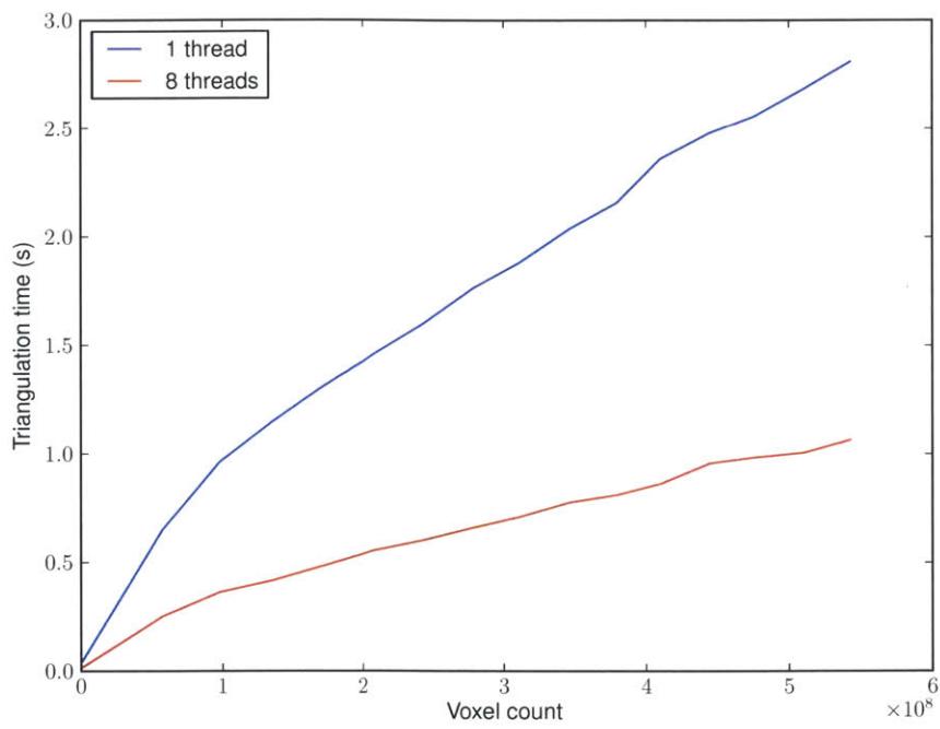
Figure 2-15: Triangulation time
