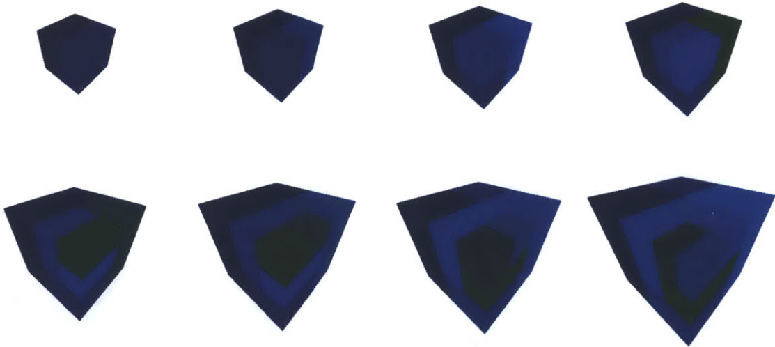
Figure 4-4: Subdivision meshes
