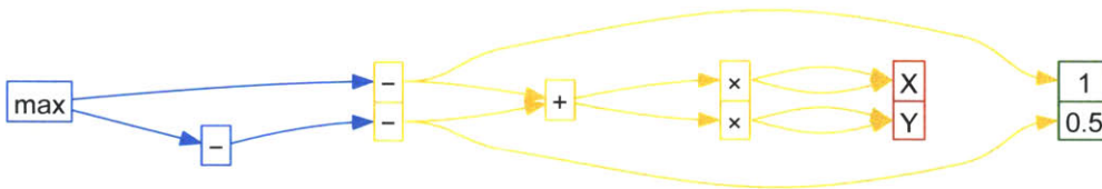
Figure 3-3: Packed tree
