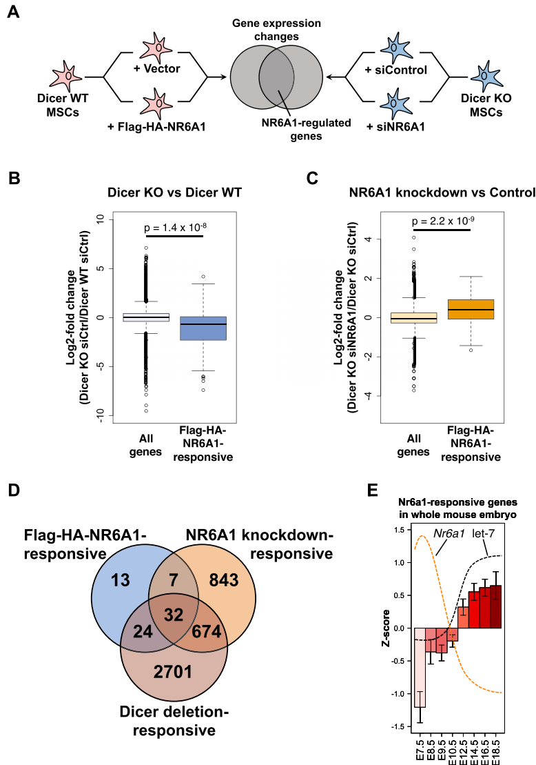
Figure 5. Gain-of-function and loss-of-function approaches identify genes regulated by let-7 target NR6A1. (A) Schematic of experimental design. (From left) Dicer wild-type (WT) MSCs (“NR6A1-low”) were infected with pMMP-puro retrovirus encoding vector control or Flag-HA-NR6A1, selected with puromycin, and passaged for several weeks prior to isolation of total RNA for polyA-selected mRNA-seq. (From right) Dicer knockout (KO) MSCs (“NR6A1-high”) were transfected with control nontargeting siRNA (siCtrl) or siRNA against Nr6a1 (siNR6A1) 48 h prior to isolation of total RNA for polyA-selected mRNA-seq. (B) Box plot of gene expression changes in siCtrl-transfected Dicer knockout versus siCtrl-transfected Dicer wild-type MSCs for all genes (“All genes”) or genes differentially expressed upon overexpression of Flag-HA-NR6A1 (“Flag-HA-NR6A1-responsive”). An FPKM cutoff \geq 0.1 was used for all compared data sets. P -value was calculated by Wilcoxon rank-sum test. (C) Box plot of gene expression changes in siNR6A1-transfected Dicer knockout versus siCtrl-transfected Dicer knockout MSCs for all genes (“All genes”) or genes differentially expressed upon overexpression of Flag-HA-NR6A1 (“Flag-HA-NR6A1-responsive”). An FPKM cutoff \geq 0.1 was used for all compared data sets. P -value was calculated by Wilcoxon rank-sum test. (D) Triple overlap of Flag-HA-NR6A1-responsive, NR6A1 knockdown-responsive, and Dicer deletion-responsive gene sets. (E) Average Z-score in the whole mouse embryo time course for 32 NR6A1-responsive genes defined in D. The orange dashed line shows Nr6a1 expression, and the black dashed line shows let-7 expression. Error bars indicate the SEM. See also Supplemental Figure S6 and Supplemental Table S4.
