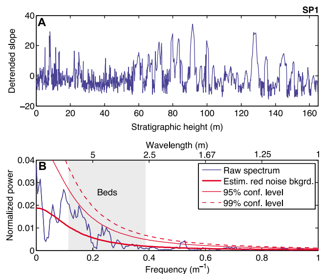
Figure 10. (a) Detrended slope for the stratigraphic transect at site SP1. (b) Power spectrum of data in Figure 10a. Shaded portion corresponds to 1\text{-}\sigma range of bed thickness measurements at same site.
