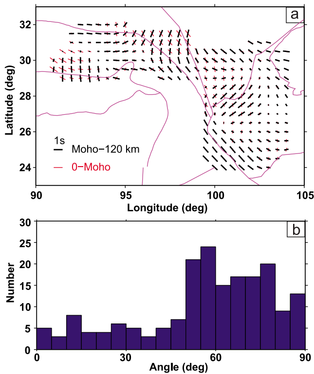
Figure 14. Comparison of the predicted shear wave splitting in the crust (red bars in Figure 14a) with that in the uppermost mantle (Moho–120 km) (black thick bars in Figure 14a). The histogram of the angle differences between red and black bars in Figure 14a, both with splitting time larger than 0.2 s is shown as Figure 14b, with the vertical axis the number of grid points in the study region for comparison and the horizontal axis the angle difference (in degree).
