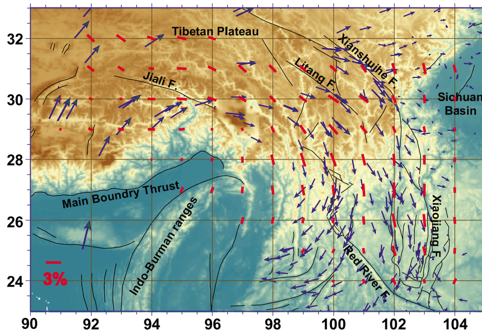
Figure 11. Observed azimuthal anisotropy at 10 km (red bars), local fault systems (black lines), and GPS velocity field (blue arrows) with respect to the South China Block. The sources of GPS measurements are from Chen et al. [2000], Zhang et al. [2004], and Sol et al. [2007].
