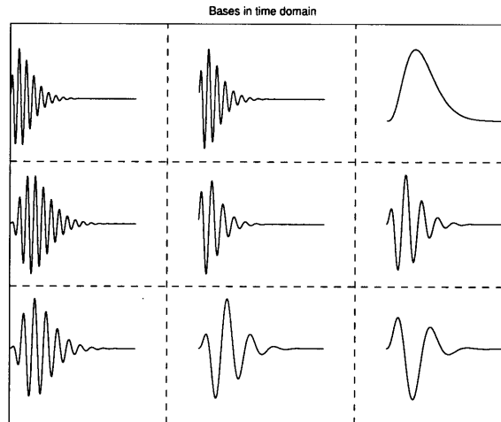
Gammatone examples for various values of f , \alpha and \beta .
