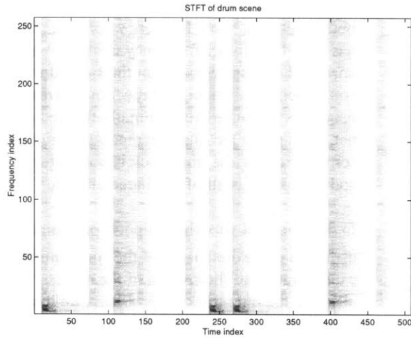
Figure 8 The STFT of the drum loop scene. The individual components are easily identified by eye from their temporal and spectral characteristics.
