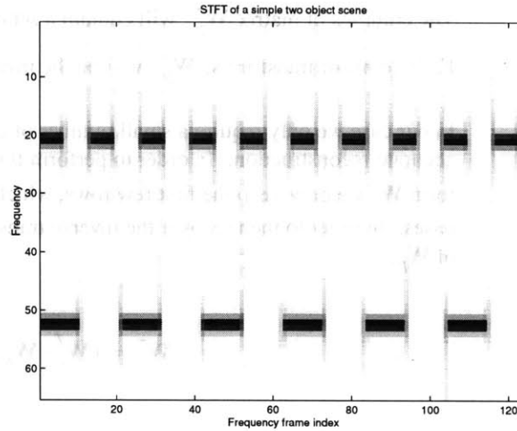
Figure 2 The magnitude STFT of a simple two object scene. Note that the two objects feature different frequency and time characteristics
