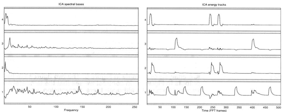
Figure 9 Analysis of the data in Figure 8. The left figure displays the estimated resynthesis spectral bases, and the right figure their energy through time. In contrast to the original objects we have a fair decomposition of the scene to its original comprising elements
