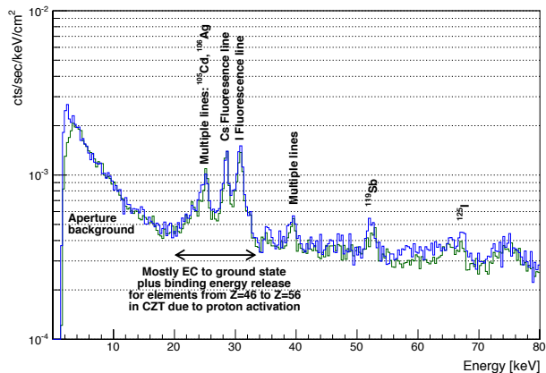
FIG. 11.— Background spectrum from observations of the Extended Chandra Deep Field South (ECDFS). At low energies the background is dominated by leakage through the aperture stop, while at high energies ( E \gtrsim 10 keV) atmospheric albedo and activation components dominate. Several prominent lines can be seen in the 20–40 keV band, which are a combination of fluorescence from the CsI shield and electron capture to the ground state plus binding energy release from elements with Z = 46 - 56 .
