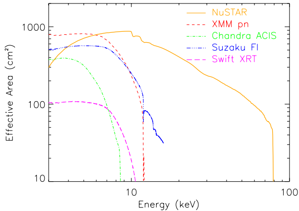
FIG. 2.— Effective collecting area of NuSTAR compared to selected operating focusing telescopes. NuSTAR provides good overlap with these soft X-ray observatories, and extends focusing capability up to 79 keV.
