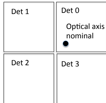
FIG. 5.— Photo of a NuSTAR focal plane (top). The focal plane consists of a 2 \times 2 array of CdZnTe pixel detectors, each with 32 \times 32 pixels 0.6 mm in size. The detectors are referred to as Det 0 – 3. The optical axis nominal location is approximately 1' from the chip gaps on Det 0 (bottom).
