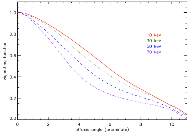
FIG. 4.— The reduction in effective area as a function of off-axis angle resulting from vignetting in the optics. The curves show the vignetting function for different incident energies. Due to the tightly nested low-graze-angle design and the change in reflectance of the shells as a function of energy, the vignetting is strongly energy dependent above 15 keV.
