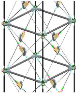
FIG. 3.— Close up including one full bay of the NuSTAR mast. Diagonal cables tension and latch during deployment, locking the carbon fiber elements into a stiff structure.
