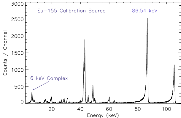
FIG. 9.— Spectrum of the ^{155}\text{Eu} flight calibration source for focal plane module A taken during on-orbit commissioning. At energies below 50 keV the resolution is 400 eV FWHM and is constant with energy, being determined by the electronic noise. Above this the energy resolution broadens due to charge trapping effects in the detector, reaching 1.0 keV FWHM at 86 keV.
