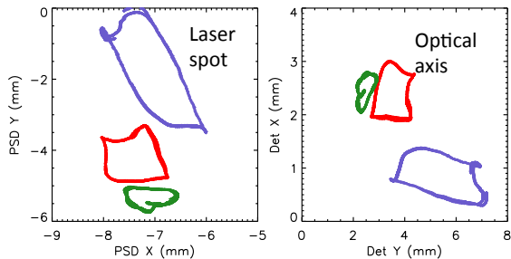
FIG. 6.— Left: Measured location of the laser beam on the metrology system position sensitive detector (PSD) for module A. The three sets of tracks show 5-6 orbits each for three different celestial targets differing in pointing direction relative to the Sun. The character of the motion changes with thermal conditions, with the maximum amplitude being \sim 3 mm. Right: Motion of the Optical Axis (OA) of the X-ray optic on the focal plane detector resulting from the mast motion for module A. The optical axis moves by about 3 mm, or 1' over the course of an orbit
