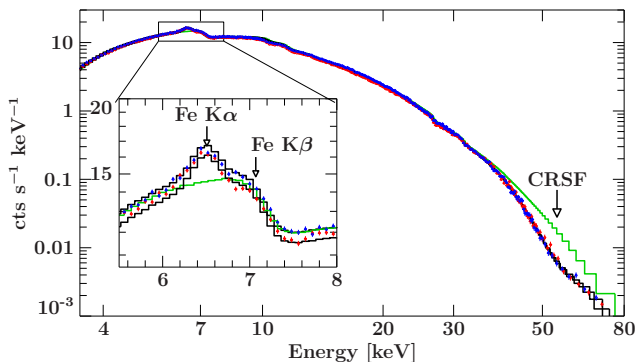
FIG. 10.— Spectrum with 15 ks exposure of Vela X-1 taken by NuSTAR . The red curve shows focal plane module A and the blue curve is from B. The inset shows the Fe-line region. The good broad band response enables NuSTAR to measure both Fe-line fluxes and high energy continuum. A Cyclotron Resonance Scattering Feature (CRSF) is seen with high significance at 55 keV.
