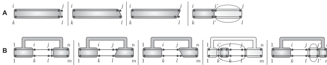
FIGURE 4. Inside and outside decomposition by the recursions. (A) Inside. The gray inside regions correspond to the matrix Z^M and the white inside region to Z^D . (B) Outside. The gray outside regions correspond to entries in Z^M ; the white outside region represents an entry of Z^D .
