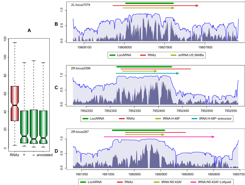
FIGURE 2. Accurate ncRNA boundaries for Drosophilids RNAz screen. (A) Deviation from annotated boundaries. We compare the deviation of RNAz (red) with the deviation of the boundaries as determined with our method (green). When the notches around the medians do not overlap, there is strong evidence that the medians differ. We show results of our method in three variants, since the alignment quality could be expected to depend on the sequence orientation: first, always aligning the sequences in forward orientation (+); second, in reverse orientation (-); third, in the orientation of the ncRNA annotation (annotated). (B–D) STAR plots with LocARNA-P predictions (thick green lines on top), RNAz predictions (red lines below), and annotated regions, RNAz predictions (red), and LocARNA-P predictions (green). (B) LocARNA-P precisely locates the snoRNA:U5:38ABa annotated in FlyBase. (C) For tRNA:H:48F, our prediction is well correlated with the precursor (cyan line) as described by Frendewey et al. (1985) (FlyBase annotation). (D) In the case of tRNA:N5:42Af, the magenta line shows the tRNA precursor, including the flanking region given by Lofquist and Sharp (1986). Here, RNAz indicates a 3' extension, whereas LocARNA-P indicates the structure in the 5' part of the precursor. As shown by Lofquist and Sharp (1986), the 5'-flanking regions of the tRNA5Asn genes differentially arrest RNA polymerase III.
