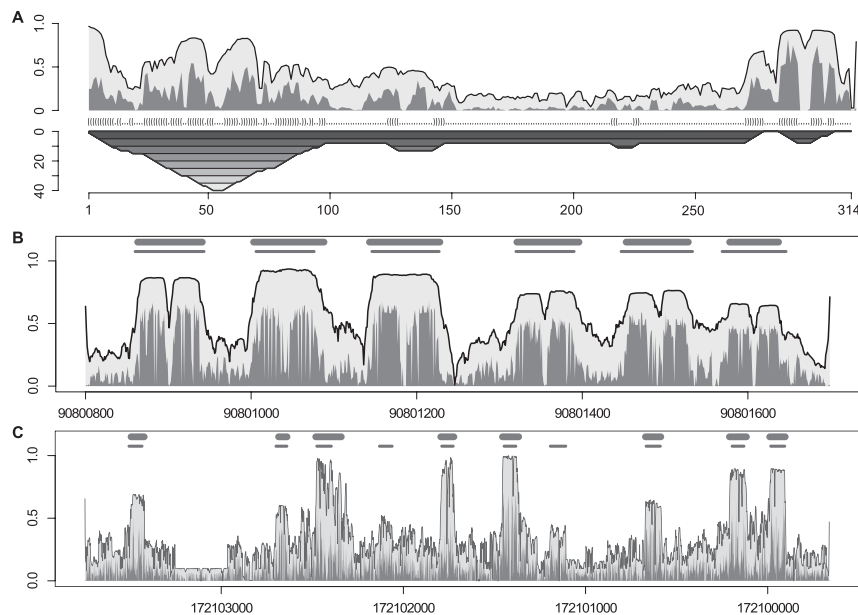
FIGURE 1. STAR profile plots with annotations. In each profile plot, the dark regions indicate structure reliability, the light regions represent sequence reliability, and the thin line shows the combined column-reliability. The thick lines on top of B and C show the automatic prediction based on the STAR profile; below we indicate the known annotation by thinner lines. (A) STAR plot of an alignment of nine ncRNAs from the 7SK ncRNA family projected to the X. laevis sequence. The profile is annotated with a mountain plot of the consensus structure. (B) STAR plot for the LocARNA-P alignment of the miRNA cluster hg18, chr13, positions 90800800–90801699, projected to the human sequence; the known microRNAs are easily detected using our method. (C) STAR plot for the LocARNA-P alignment of the human gene gas5 (hg18, chr1, 172,099,662–172,103,748); the gene is aligned with four other mammalian sequences; the introns of human gas5 host 10 C/D-box snoRNAs.
