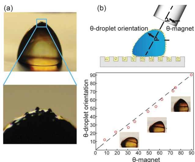
FIG. 2. (a) Symmetric magnet configuration. Magnetic particles cluster over the cloaked water droplet and orient themselves to be directly underneath the region of highest magnetic field intensity. (b) Asymmetric magnet configuration. Magnet approaching angle versus droplet orientation angle which shows that the clumped particles act to deform the droplet directly in the direction of highest field intensity, or directly at the angle the magnet is being approached.
