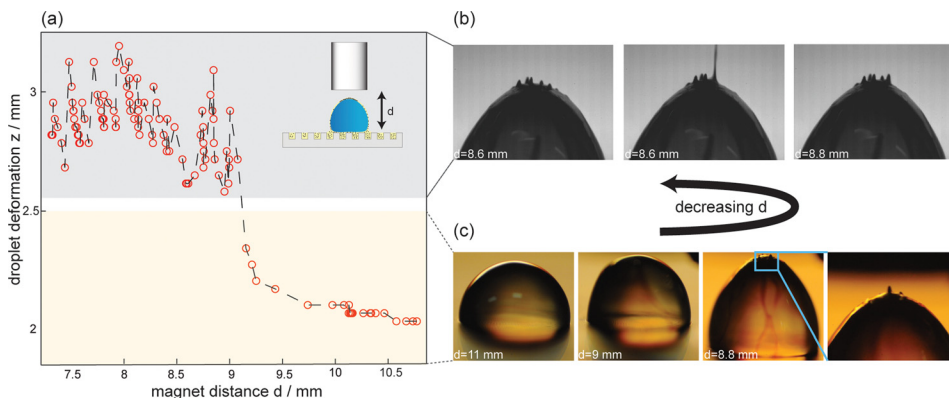
FIG. 3. Jetting transition of ferrofluid-cloaked droplet. (a) Droplet deformation versus magnet distance. Droplet height continuously increases until critical jetting transition distance is reached. Droplet height then begins to fluctuate as fluid jets grow and detach repeatedly from cloak/air interface. (b) High-Speed images of fluid jet detaching from cloak/air interface in the jetting regime. 59 (c) Snapshots of droplet deformation as the magnet is slowly approached to the surface (Multimedia view). [URL: http://dx.doi.org/10.1063/1.4891439.2 ]
