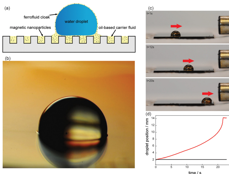
FIG. 1. Ferrofluid-impregnated textured surface. (a) Schematic of surface with water droplet resting on top. The ferrofluid can cloak the water droplet if the spreading coefficient ( S_{ow(v)} \geq 0 ) is greater than 0. (b) Photograph of water droplet resting on the surface with the ferrofluid cloak. (c) Snapshots of droplet mobility experiment as water droplet is accelerated towards the magnet. 59 (d) Water droplet position versus time in mobility experiment (Multimedia view). [URL: http://dx.doi.org/10.1063/1.4891439.1 ]
