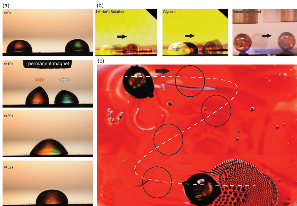
FIG. 4. (a) Two water droplets (dye used to color droplets) are placed on ferrofluid-infused surface. A magnet is lowered vertically directly between droplets and causes them to move toward one another. Coalescence of droplets occurs and is captured just before droplets fully mix. (b) Droplets of various fluids and one solid are actuated and displaced when a permanent magnet is approached to the surface. (c) Water droplet being dragged along an s-curve as the magnet is held beneath the surface.
