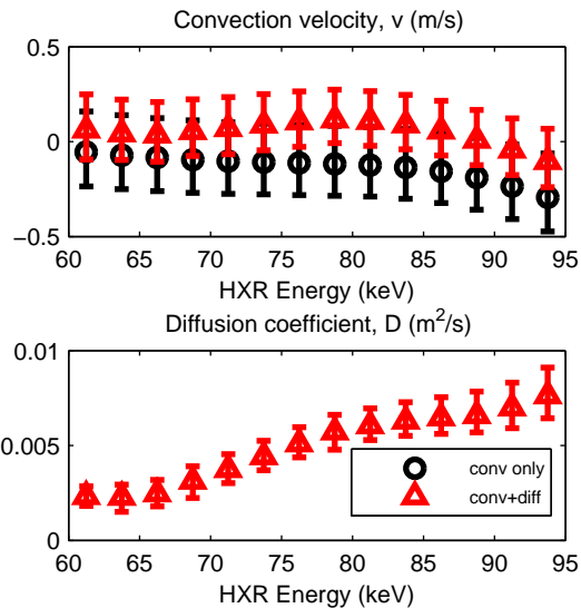
FIG. 11. (Color online) Inferred fast electron convection velocities and diffusivities for the I_p=800 kA case discussed in section III B. In this case, the launched n_{\parallel}=3.1 . Plasma parameters were B=5.4 T, T_{e0}=2.3 keV, and \bar{n}_e = 9 \times 10^{19} \text{ m}^{-3} .
