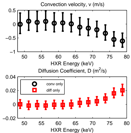
FIG. 12. (Color online) Inferred fast electron convection velocities and diffusivities for the I_p=600 kA case discussed in section III B. In this case, the launched n_{\parallel}=3.1 . Plasma parameters were B=5.4 T, T_{e0}=1.9 keV, and \bar{n}_e = 9 \times 10^{19} \text{ m}^{-3} . In this case, convection and diffusion were included in the model one at a time.
