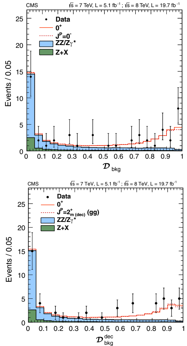
FIG. 23 (color online). Distribution of \mathcal{D}_{bkg} (top) and \mathcal{D}_{bkg}^{dec} (bottom) in data and MC expectations for the background and for a signal resonance consistent with the SM Higgs boson with m_{0^+} = 125.6 GeV.
