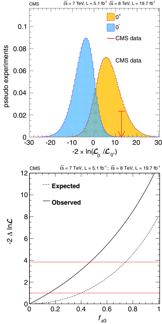
FIG. 26 (color online). (top) Distribution of the test statistic q = -2\ln(\mathcal{L}_0^-/\mathcal{L}_0^+) of the pseudoscalar boson hypothesis tested against the SM Higgs boson hypothesis. Distributions for the SM Higgs boson are represented by the yellow histogram, and those for the alternative J^P hypotheses are represented by the blue histogram. The arrow indicates the observed value. (bottom) Average expected and observed distribution of -2\Delta\ln\mathcal{L} as a function of f_{a3} . The horizontal lines at -2\Delta\ln\mathcal{L} = 1 and 3.84 represent the 68% and 95% C.L.'s, respectively.
