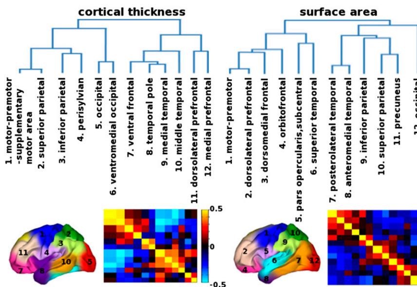
Fig. 3. Organization among genetic clusters. ( Upper ) The dendrograms derived from hierarchical clustering based on genetic correlations among clusters. ( Lower ) The genetic clustering maps show anatomical locations of the clusters, and the heatmaps represent the weighted mean genetic correlations within and between clusters.
