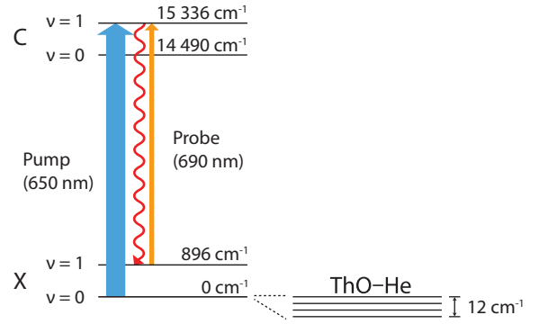
FIG. 2. (Color online) Relevant energy levels of the ThO molecule. Letters refer to the electronic states, X ( ^1\Sigma^+ ) and C (77% ^1\Pi , 20% ^3\Pi ), respectively. All measurements were performed in the ground rotational levels, J = 0 for the X state and J = 1 for the C state. Optical pumping via the X ( v = 0 ) \rightarrow C ( v = 1 ) R(0) transition at 650 nm is used to transfer the population to the X ( v = 1 ) state, which is probed using the X ( v = 1 ) \rightarrow C ( v = 1 ) R(0) transition at 690 nm. The relative scale of ThO-He bound-state energies is also shown.
