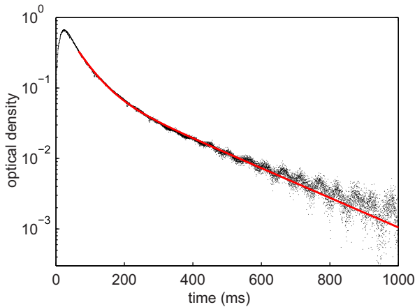
FIG. 1. (Color online) Optical density (OD) decay of ThO in its X ( v = 0 , J = 0 ) state at a high helium density ( n_{\text{He}} = 3 \times 10^{16} \text{ cm}^{-3} ) and 2.4 K (single shot). The solid (red) line is fit to a sum of two exponentials corresponding to ThO loss to diffusion and to vdW molecule formation. We verify that both diffusion modes and temperature stabilize within the first 50 ms by observing decay of atomic chromium produced simultaneously (not shown). The apparent oscillation visible at late times (small OD) is caused by mechanical vibration of the apparatus, and it has no significant effect on the early-time (large-OD) fitted lifetime.
