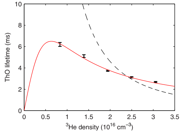
FIG. 5. (Color online) Observed vibrational quenching of the X ( v=1 , J=0 ) state of ThO at 1.2 K. Error bars are statistical uncertainties. The ^3\text{He} density is determined from the diffusive decay of Cr produced simultaneously [23]. The solid (red) line is a combined diffusion, two-body, and three-body fit to the data [Eq. (7)]. The dashed black line is a three-body fit. The effect of diffusion is insignificant for n_{\text{He}} \gtrsim 1.2 \times 10^{16} \text{ cm}^{-3} .
