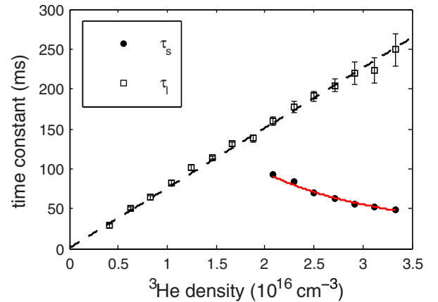
FIG. 3. (Color online) Fits to early- and late-time decay-time constants \tau_s and \tau_l in Eq. (4) and Eq. (5) at various helium densities at 2.4 K. Open squares (filled circles) denote fitted values for \tau_l ( \tau_s ). The dashed black line and solid (red) line are fits to Eq. (5) and Eq. (4), respectively, where the diffusive rate constants in Eq. (2) are extracted.
