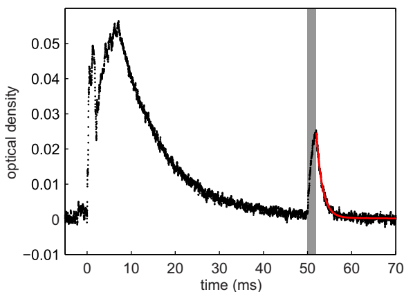
FIG. 4. (Color online) Optical density (OD) of ThO in its X ( v=1 , J=0 ) state at 1.2 K (single shot). The initial OD, produced by molecule production via laser ablation, varies in both magnitude and duration and therefore it is unsuitable for the study of vibrational quenching. Instead, at 50 ms, a short optical pumping pulse [shaded (gray) area] transfers the population from the X ( v=0 , J=0 ) state. This method removes noise from shot-to-shot fluctuation. The solid (red) line at the right is a fit to a single-exponential decay.
