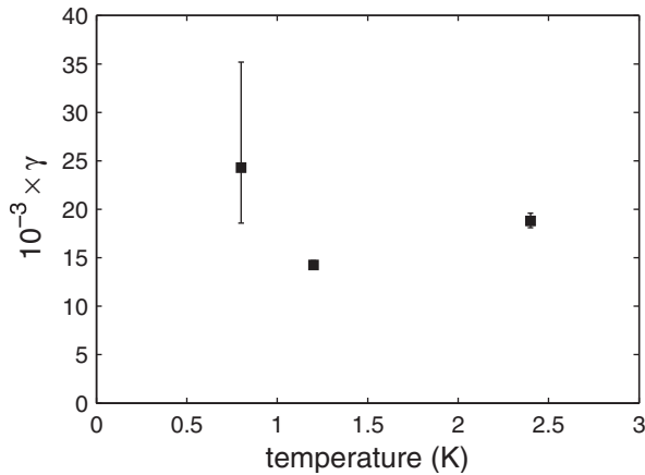
FIG. 6. Collisional quenching of the first vibrationally excited state of ThO in collisions with ^3\text{He} . Shown is the ratio \gamma of the momentum transfer to the vibrational quenching cross section for the X ( ^1\Sigma^+ ), v = 1 , J = 0 state versus the temperature.
