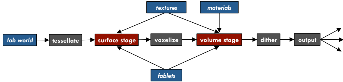
Figure 4-1: The OpenFab pipeline defines a programming model for synthesizing continuous volumetric material mixtures for 3D printing. As an input (blue) it takes a scene graph describing a set of object boundary representations, textures, printer materials, and user-programmable fablets —similar to shaders. From this input, it generates a discrete volumetric material definition that is device specific. Some stages are fixed-function (grey), controlled by high-level parameters and printer characteristics, while fablet stages (red) are programmable by the user.
