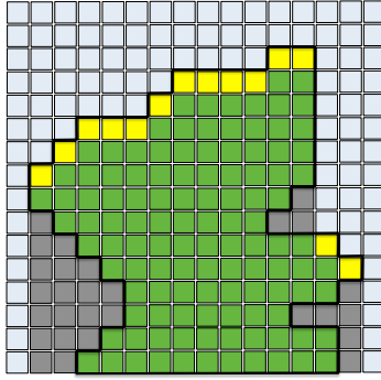
Figure 6-2: A 2D representation of the OpenFab support generation approach. Voxels in green and yellow are part of the object being printed. Voxels in grey are support voxels. Voxels in yellow are part of the depth map that is generated with a high-resolution, fixed-point rasterizer. Support voxels are generated for empty voxels iff there is a voxel in the depth map above them.
