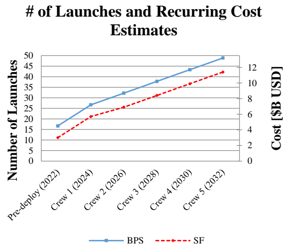
Fig. 26: Number of launches required and resulting estimated launch vehicle production and launch cost for the first ten years of Mars One operation for both the BPS and SF cases.
