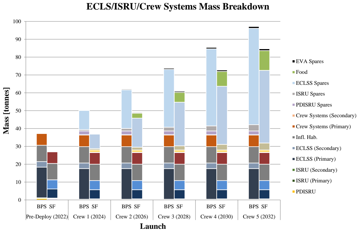
Fig. 24: Mass breakdown of the cargo missions for the first 5 crews, including the pre-deploy mission. The mass for each mission is shown for both the architecture utilizing a BPS and the architecture using stored food (SF). The total mission mass is shown as a stacked bar of the primary and secondary systems, inflatable habitat (infl. hab.), spare parts, and resupply food.
