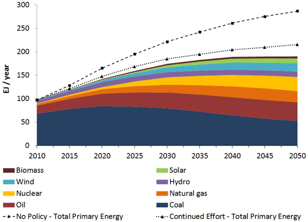
Figure 1. Energy demand in the No Policy , Continued Effort , and Accelerated Effort scenarios, with the primary energy mix shown for the Accelerated Effort scenario.
