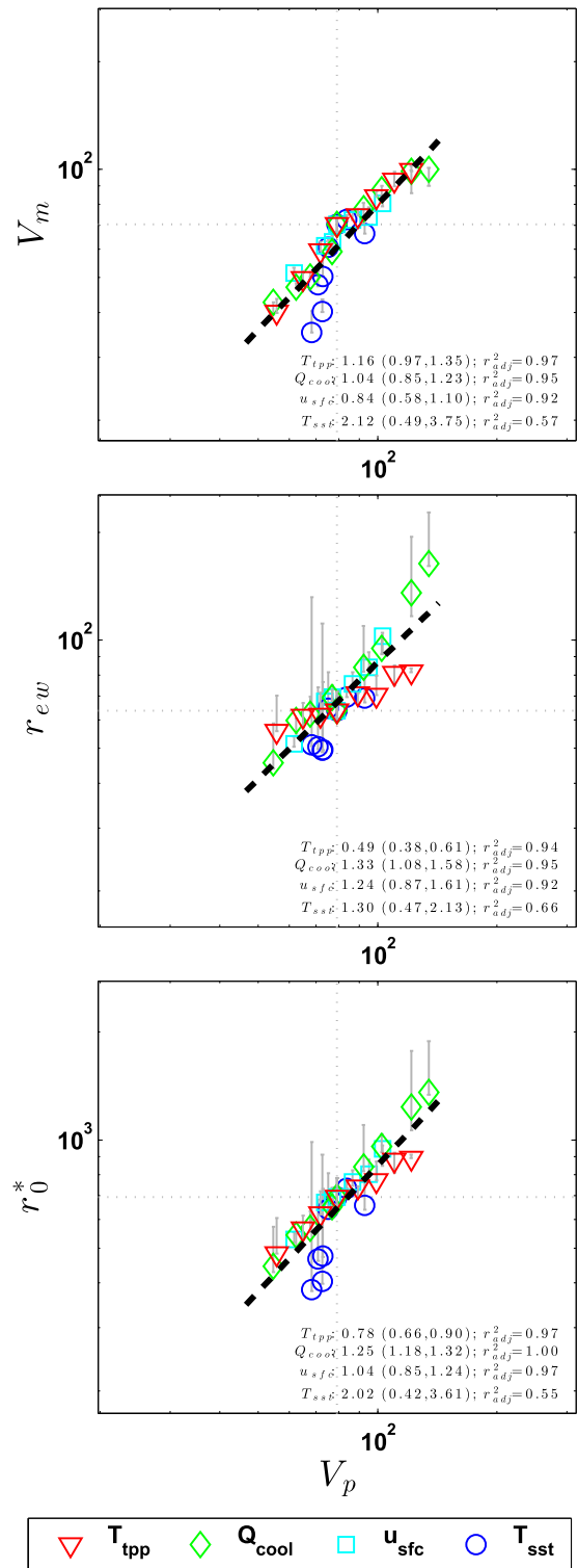
FIG. 11. Scaling of the respective equilibrium values of V_m , r_{\text{ew}} , and r_0^* (ordinate) with V_p (abscissa) for the four thermodynamic parameters. Dashed line indicates best fit to all data. For each individual parameter, best-fit linear slope (95% confidence interval) and corresponding adjusted r -squared statistic listed in lower-right corner. Gray bars indicate full range of variability of the 30-day running mean after day 60.
