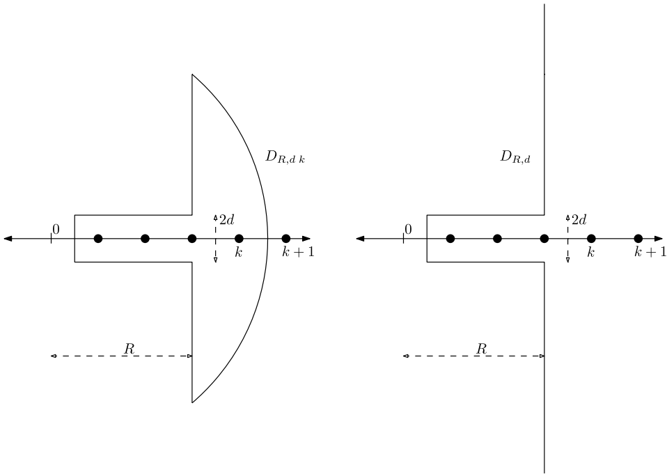
FIG. 3. Left: The contour D_{R,d;k} ; Right: The contour D_{R,d} .
