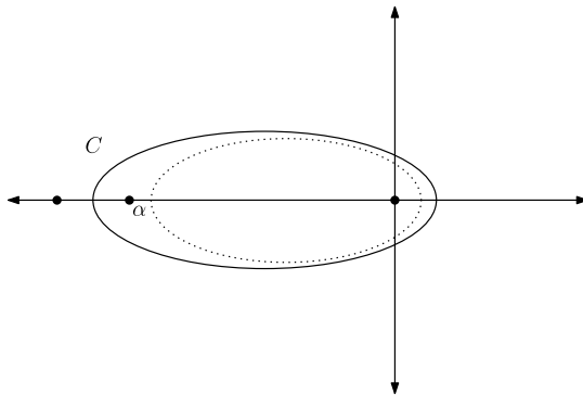
FIG. 6. The contour C is chosen so as to contain 0, \alpha and no other poles of f (such as the one indicated with a black dot to the left of \alpha ).
