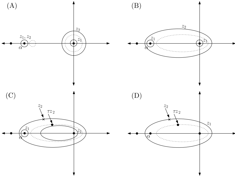
FIG. 7. (A): Both contours contain 0 and \alpha , but the z_1 contour must not contain \tau z_2 (and neither contour may contain any other poles such as the one indicated by the black dot to the right of \alpha ). (B) The z_2 contour may freely (without crossing poles) be deformed to a single circle containing 0 and \alpha . (C) For z_2 fixed along that circle, the z_1 contour can be deformed and only picks a pole when crossing the point \tau z_2 . (D) After crossing that pole, the z_1 contour can be freely deformed to the same contour on which z_2 is integrated.
