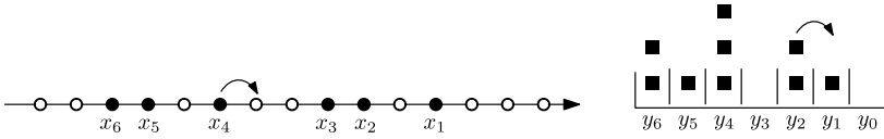
FIG. 1. Left: q -TASEP with six particles. The indicated jump of x_4 occurs at rate a_4(1 - q^2) since the gap x_3 - x_4 - 1 = 2 . Right: The dual TAZRP with sites \{0, 1, \dots, 6\} . The indicated jump occurs at rate a_2(1 - q^2) since y_2 = 2 .
