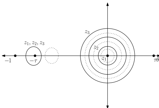
FIG. 5. The contour for z_A includes 0, -\tau but does not include -1, \tau\theta or \{\tau z_B\}_{B>A} . The dotted lines represent the images of the contours under multiplication by \tau . For instance, observe that the z_1 contour does not include the image under multiplication by \tau of z_2 or z_3 .
