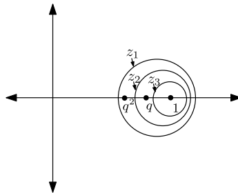
FIG. 2. Possible contours when k = 3 for the z_j contour integrals in Proposition 3.2.
