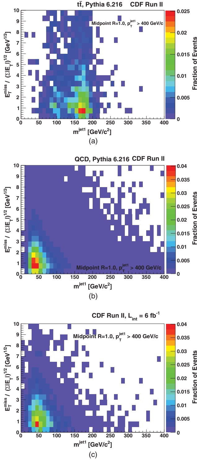
FIG. 19 (color). The S_{\text{MET}} versus m^{\text{jet}1} distribution for simulated t\bar{t} events (a), simulated QCD events (b), and all data events (c) with at least one jet with p_T > 400 \text{ GeV}/c and |\eta| < 0.7 using R = 1.0 MIDPOINT cones.
