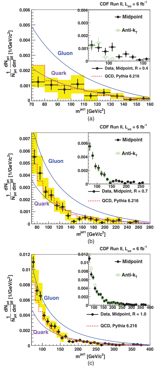
FIG. 13 (color). Multiple-interaction-corrected jet-mass distributions for jets with p_T > 400 GeV/ c and |\eta| \in (0.1, 0.7) reconstructed with an R = 0.4 (a), R = 0.7 (a reproduction of Fig. 1 of [15]), and R = 1.0 (c) MIDPOINT cone algorithm after rejection of t\bar{t} events. Comparisons with the analytic expression for the jet function for quarks and gluons are shown. The inset compares the results with the anti- k_T jet algorithm.
