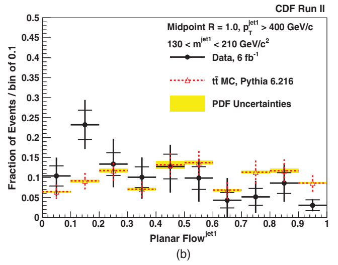
FIG. 16 (color). The normalized planar flow distribution for jets with p_T > 400 \text{ GeV}/c and |\eta| \in (0.1, 0.7) reconstructed with the R = 1.0 MIDPOINT cone algorithm. We have rejected t\bar{t} events and have required that m^{\text{jet}1} \in (130, 210) \text{ GeV}/c^2 . Data points are shown with statistical and systematic uncertainties. Overlaid in (a) are results from the PYTHIA QCD prediction (red triangles) with the PDF uncertainties (yellow bars). Overlaid in (b) are results from the PYTHIA MC prediction for the leading jet in t\bar{t} MC events (red triangles) with the PDF uncertainties (yellow bars).
