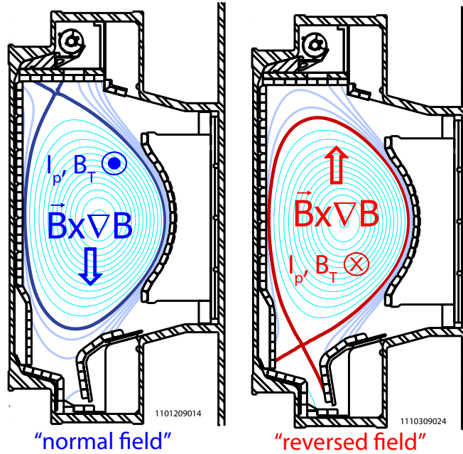
Figure 2.5: C-Mod cross-sections illustrating magnetic configurations suitable for I-mode access. Either upper-null operation in the normal field direction, or lower-null with field and current reversed provides ion \nabla B drift away from the X-point. This configuration is unfavorable for the H-mode threshold, but allows for easier access to I-mode.
