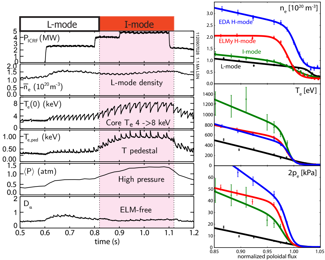
Figure 2.7: (left) Characteristic traces for a typical I-mode. At the L-I transition, the core and edge temperature rise over several sawtooth cycles (visible in the oscillations in T_e(0) ) before reaching a steady level; global confinement and pressure rise accordingly. However, the density remains at L-mode levels, and no ELMs are exhibited. (right) Edge profiles for density, temperature, and pressure in L-, I-, and H-mode. The I-mode (green) retains an density profile comparable to the L-mode (black), unlike the ELMy (red) and EDA (blue) H-modes which form a strong density pedestal. However, the I-mode forms a higher temperature pedestal than either H-mode. As a result, the I-mode reaches comparable pedestal pressures to the H-modes while retaining L-mode particle transport.
