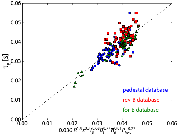
Figure 5.27: Power-law fit to I-mode energy confinement time \tau_E , with the ansatz of an L-mode-like R^{1.5}\epsilon^{0.3} size scaling fixed (fit #5 in table 5.1). Both the high-resolution pedestal database and older reversed-field LSN and forward-field USN I-mode databases are used. Note the expected weak degradation of \tau_E with heating power.
