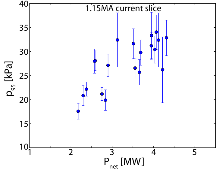
Figure 5.9: Pedestal pressure ( 2 \times p_{e,95} ) versus net heating power for the 1.15 MA current slice, illustrating the trend p_{95} \sim P_{net} at fixed current. This is consistent with the power trend in the I-mode temperature pedestal, T_{e,95} \sim P_{net}/\bar{n}_e .
