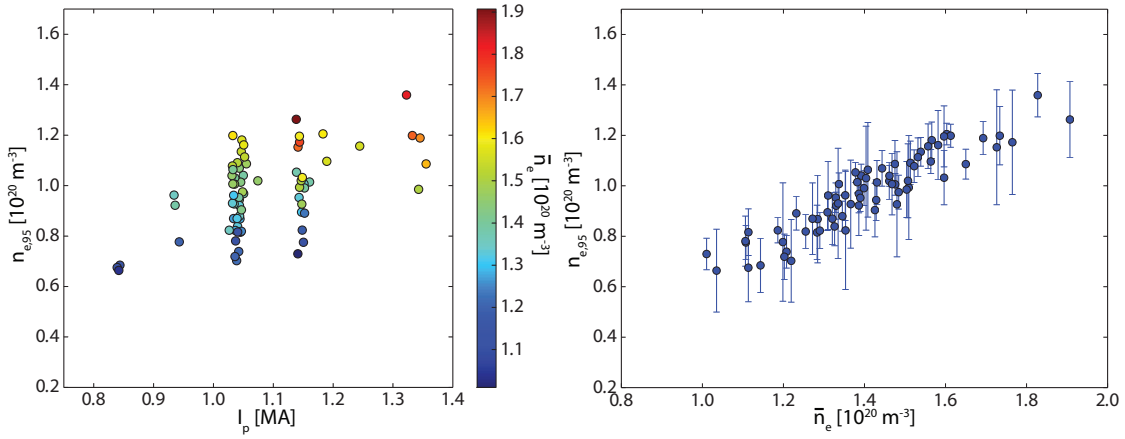
Figure 5.6: Pedestal density as a function of current (left, colored by \bar{n}_e ) and line-averaged density (right). The pedestal density is set solely by operator fueling; in contrast the transport-limited pedestals in EDA H-mode, plasma current is a poor predictor of the pedestal density, with the trend due only to the co-variance between I_p and \bar{n}_e .
