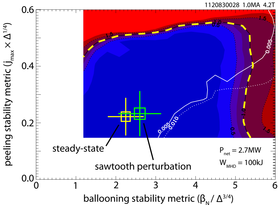
Figure 6.9: Peeling-ballooning MHD stability calculated by ELITE and KBM thresholds calculated by BALOO for an I-mode case, comparing the time-averaged data against pedestal profiles prepared with data masking to the first 25% of the sawtooth cycle following the heat pulse reaching the edge (see fig. 6.8). Note that, to directly compare two separately-calculated equilibria, we replace the \alpha_{\text{MHD}} and j_{\parallel} axes with stability metrics arising from peeling and ballooning MHD. While the sawtooth heat pulse does measurably perturb the pedestal in stability space, it is insufficient to reach either the peeling-ballooning or KBM threshold.
