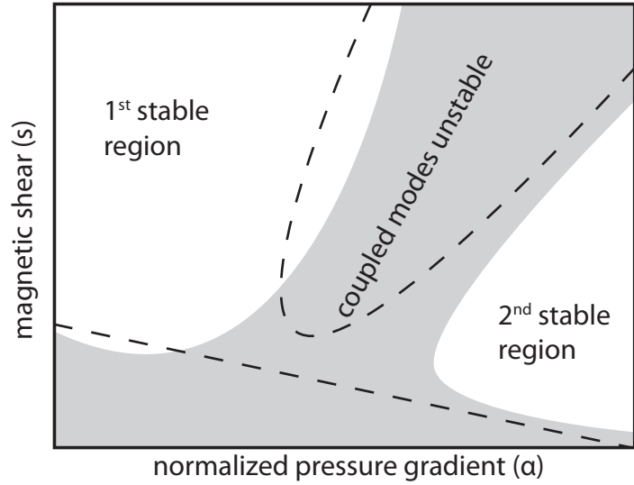
Figure 3.2: Schematic in s - \alpha_{\text{MHD}} space of finite- n coupled peeling-ballooning instabilities, with the infinite- n decoupled results (see fig. 3.1) shown by the dashed lines. Mode coupling tends to stabilize finite- n ballooning modes. However, the coupled modes can close off access to the second-stable regime; only in cases with very strong “magnetic wells” (typically achieved with extreme plasma shaping) does this access reopen.
