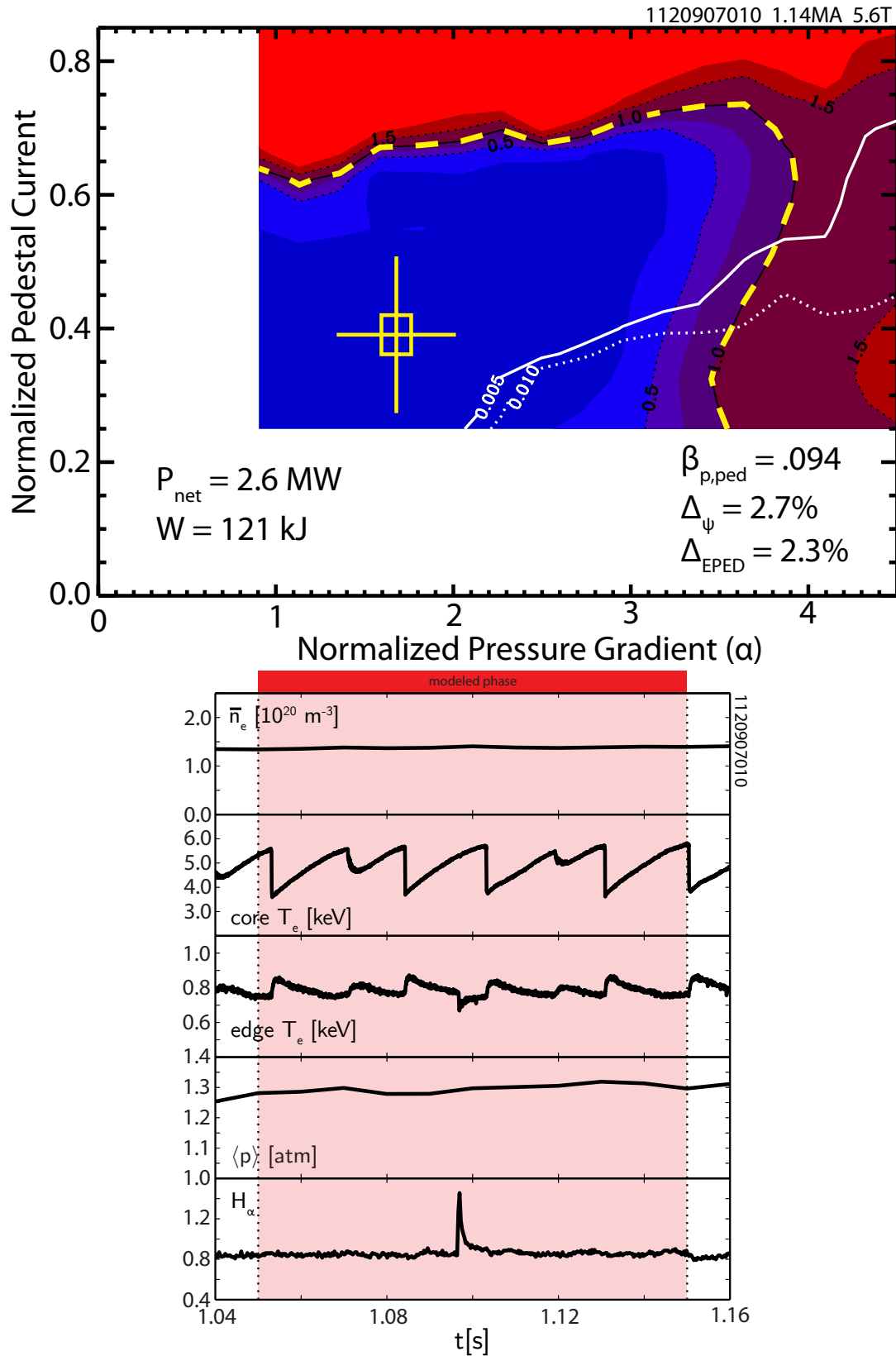
Figure 6.12: MHD stability contour for I-mode generated by the ELITE code, with results from the infinite-n BALOO calculation overlaid. The experimental measurement is shown by the crosshair, with the stability boundary indicated by the yellow dashed line. Parameters for the modeled phase of the discharge are shown below. This case exhibited a solitary ELM not triggered by the sawtooth heat pulse, with the characteristic edge temperature crash of a canonical ELM. However, the I-mode phase around the ELM is calculated to be peeling-ballooning stable and below the KBM threshold.
