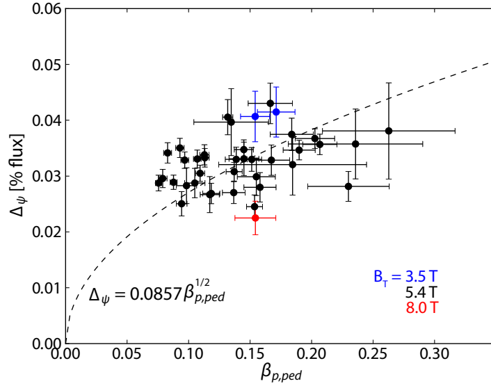
Figure 4.16: Ensemble-averaged EPED width \Delta\psi (eq. (4.3)) versus \beta_{p,ped} , color-coded by field set. The expected scaling from the KBM limit, \Delta\psi = c\beta_{p,ped}^{1/2} , is shown with a scale factor of 0.0857, consistent with observations in other experiments.
