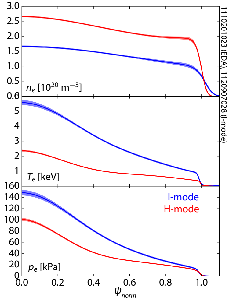
Figure 5.19: Profiles in density, temperature, and pressure for I-mode and EDA H-mode, with the \pm\sigma errorbars indicated by the shaded region. The H-mode case exhibits a very strong density pedestal, with a somewhat reduced temperature pedestal; the I-mode, in contrast, has a significant temperature pedestal with a relaxed density profile. While this typically results in a reduced pedestal pressure in I-mode compared to H-mode, core profile stiffness supports very high central temperatures, such that I-mode exhibits comparable or greater core and average pressure despite the relaxed pedestal.
