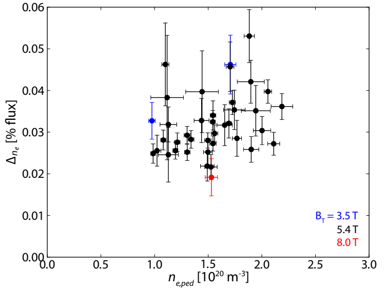
Figure 4.22: Density pedestal width versus pedestal density. Contrary to expectations from neutral-penetration models (see section 3.1.2), there is little systematic variation of the density pedestal width and height. This is consistent with the highly opaque SOL typical on C-Mod.
