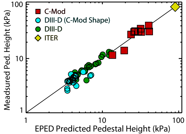
Figure 4.28: EPED predictions versus measured pressure pedestal heights from DIII-D and C-Mod, spanning a significant range of pedestal pressures. Notably, C-Mod pressure pedestals reach within a factor of \sim 2 of the predicted ITER pedestal height. Reproduced from [19]
