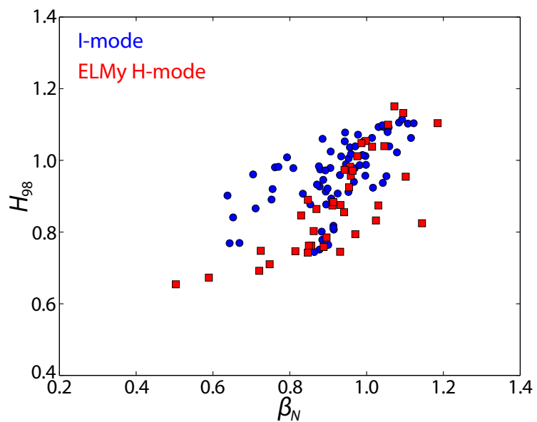
Figure 5.20: Global normalized \beta_N versus confinement factor H_{98} for I-mode and ELMy H-mode. Despite the relaxed pedestal pressure, I-modes reach comparable average pressures, while maintaining H-mode-like energy confinement.
