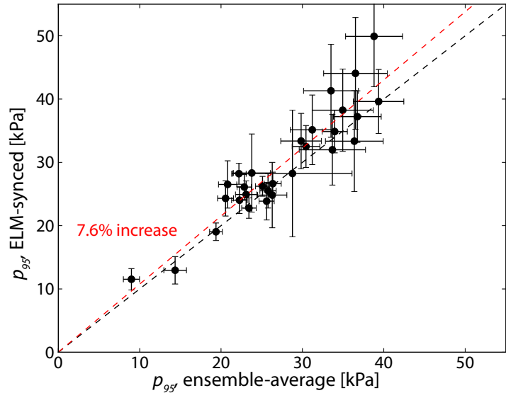
Figure 4.8: Comparison of the pressure at the 95% flux surface, p_{95} , between the ensemble-averaged and ELM-synchronized profiles. On average, ELM synchronization results in a 7.6% increase in the measured pressure. This is consistent with the ELM perturbation to the pedestal being largely restricted to the pedestal just within the steep-gradient region, with decreasing perturbation further into the plasma from the pedestal.
