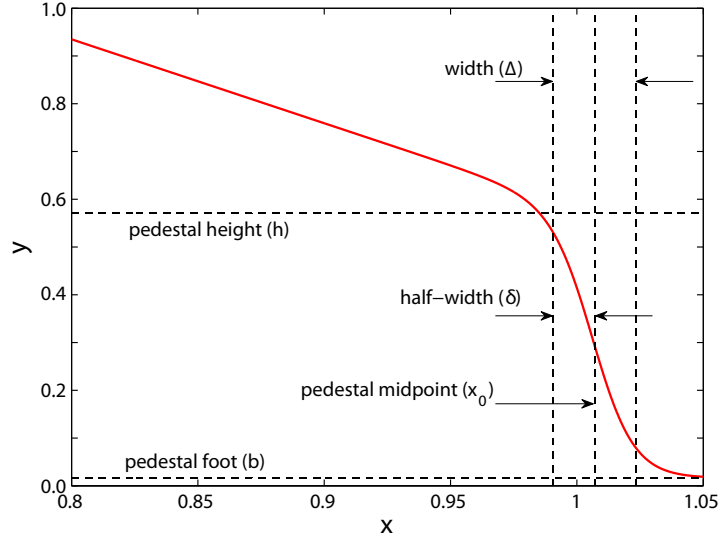
Figure 4.4: Example pedestal illustrating the mtanh function used for pedestal fitting (eq. (4.1)), defining the parameters: height h , baseline b , midpoint x_0 , half-width \delta /full width \Delta . The inboard slope is characterized by the parameter \alpha .
