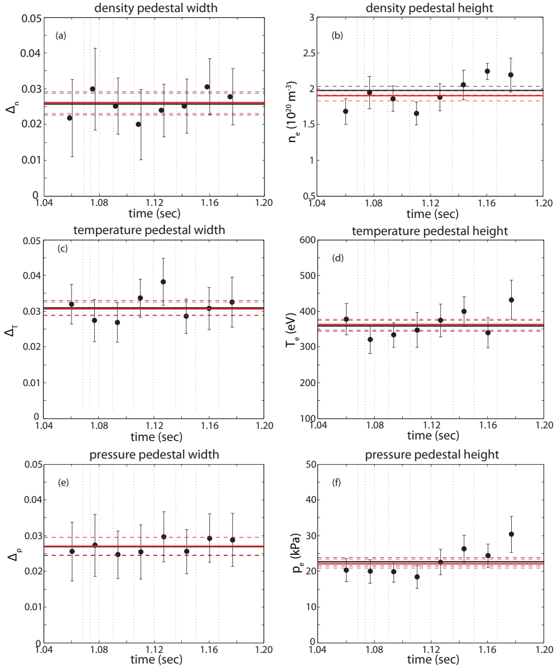
Figure 4.3: Comparison of fits for the n_e , T_e , and p_e pedestal width and height from Thomson scattering. Individual frames of data are shown as black points, with their average shown by the black line (errorbars indicated by the dashes). The ensemble-averaged fit is shown in red. The ensemble fit captures the average behavior in a steady ELMing phase well, while suppressing the random scatter found in individual frames of TS data. For comparison, ELM crash times in the window are indicated by vertical dashed lines.
