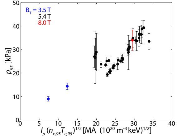
Figure 4.11: Pedestal pressure versus I_p \sqrt{n_{e,95} T_{e,95}} – effectively, the p_{ped} \sim I_p^2 \sqrt{\beta_{p,ped}} scaling predicted for a KBM-limited pedestal.
