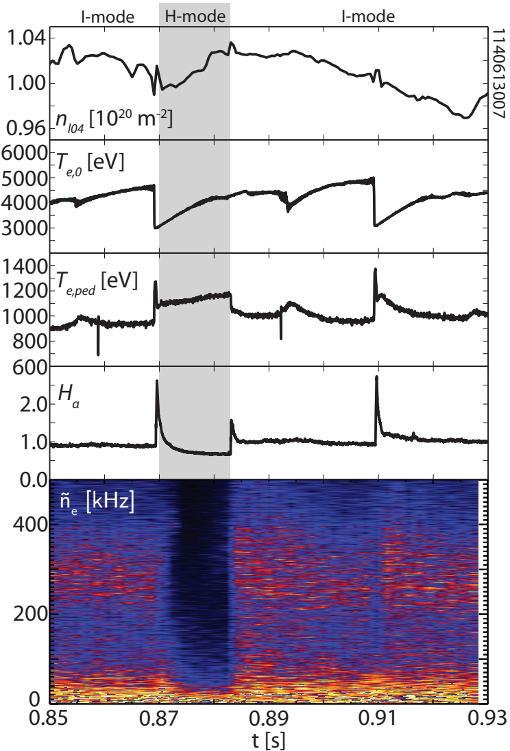
Figure 6.11: Traces of n_{104} , core and edge T_e , and H_\alpha for an I-mode exhibiting ELM-like events. The sawtooth heat pulse at \sim 0.87 s triggers an I-H transition, indicated by the drop in H_\alpha and suppression of turbulence visible on the \tilde{n}_e plot. This H-mode terminates with a non-sawtooth-triggered ELM with visible edge temperature crash and density perturbation, dropping back into I-mode. The I-mode phase also exhibits sawtooth-triggered ELM-like events with minimal density perturbation or temperature crash.
