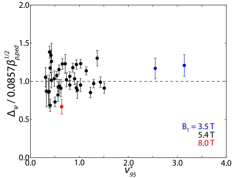
Figure 4.26: Scaling of the normalized pedestal width \Delta_\psi/0.0857\beta_{p,ped}^{1/2} versus pedestal collisionality \nu_{95}^* . Low, standard, and high-field sets are indicated in blue, black, and red respectively. No systematic variation is observed.
