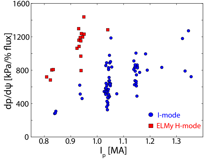
Figure 5.11: Peak pressure gradient (measured at the pedestal midpoint) versus plasma current for I-mode and ELMy H-mode. I-mode consistently exhibits a weaker pressure gradient at a given current, as well as scaling more weakly than the \nabla p \sim I_p^2 expected from the ballooning MHD stability limits associated with ELMy H-mode.
