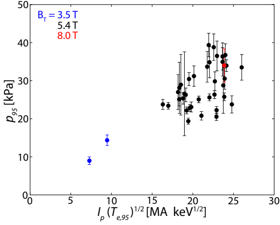
Figure 4.10: Pedestal pressure versus I_p \sqrt{T_{e,95}} – effectively, the p_{ped} \sim I_p^2 \rho_{i,pol} scaling predicted in [28].
