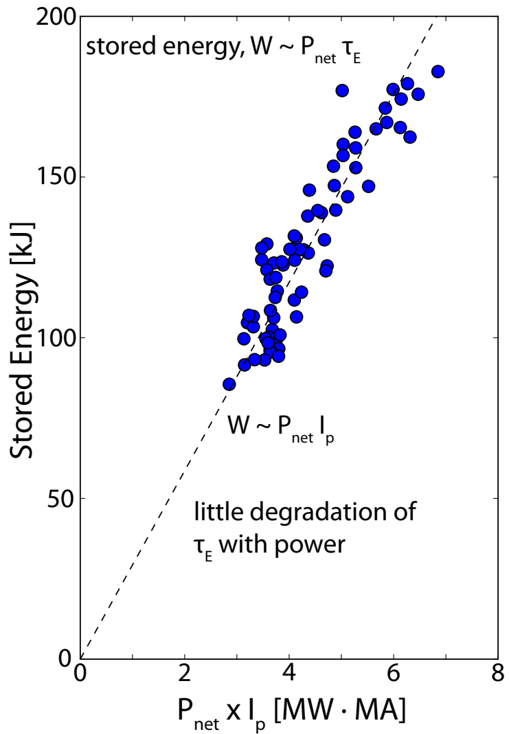
Figure 5.21: I-mode stored energy versus the product of net heating power P_{net} and plasma current I_p . Based on the H-mode confinement scaling, \tau_E is expected to scale linearly with I_p , and to show a strong degradation with heating power: \tau_E \sim I_p \times P_{net}^{-0.7} . As the stored energy is given by W \sim P_{net} \tau_E , W \sim I_p P_{net}^{0.3} is expected. The observed linear trend indicates little-to-no degradation of \tau_E in I-mode with heating power.
