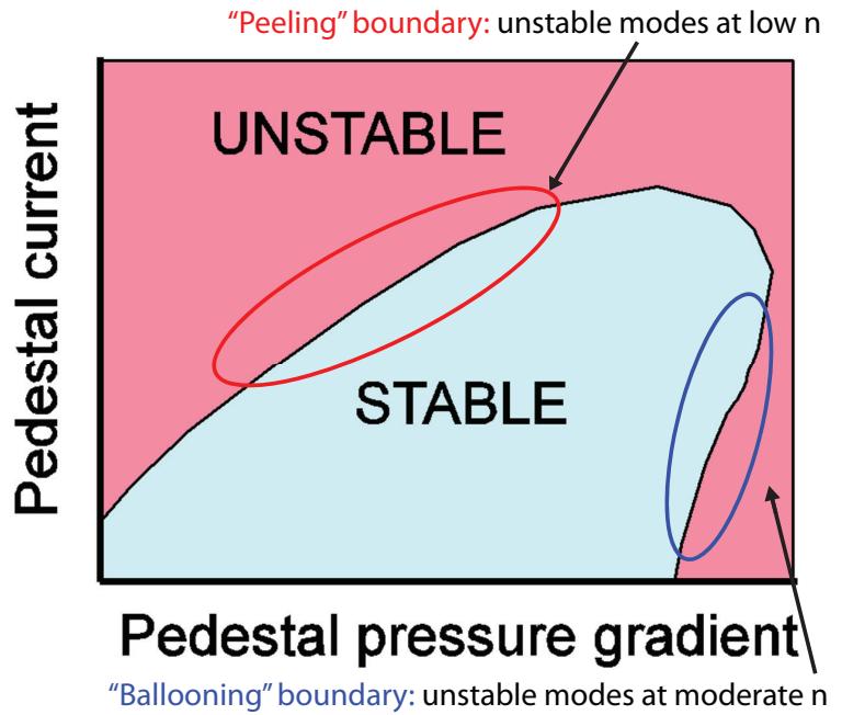
Figure 3.4: Schematic of the stability space to coupled peeling-ballooning MHD modes, set by the edge pressure gradient and current density. Ballooning modes are driven by pressure gradient, while kink/peeling modes are current-driven but stabilized by pressure gradients.
