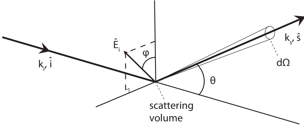
Figure A.2: Definitions of the angular dependences in the Thomson scattering geometry: namely, the angle \theta between the incident wave direction \hat{i} and scattering direction \hat{s} , and the polarization angle \phi of the incident electric field \hat{E}_i with respect to the projection of \hat{s} into the polarization plane.
