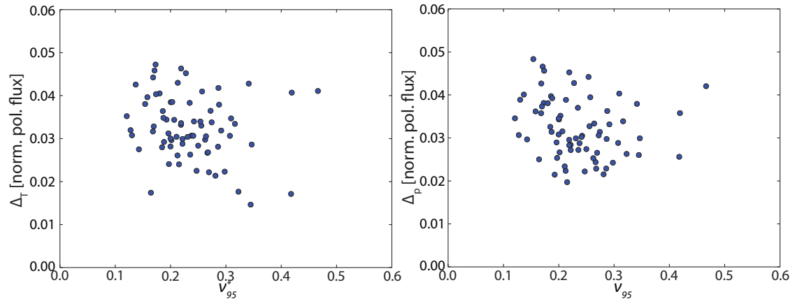
Figure 5.14: Temperature (left) and pressure (right) pedestal widths versus pedestal collisionality \nu_{95}^* . No correlation is seen.
