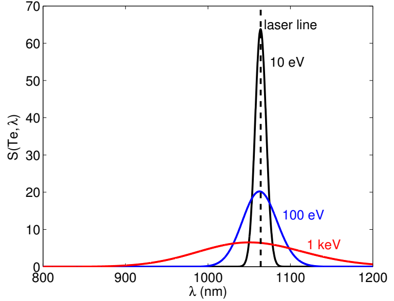
Figure A.3: Spectral functions normalized to density and laser power, evaluated at \theta = \phi = \pi/2 . The spectrum spreads farther from the laser line at higher temperature, as well as blue-shifting due to relativistic effects.
