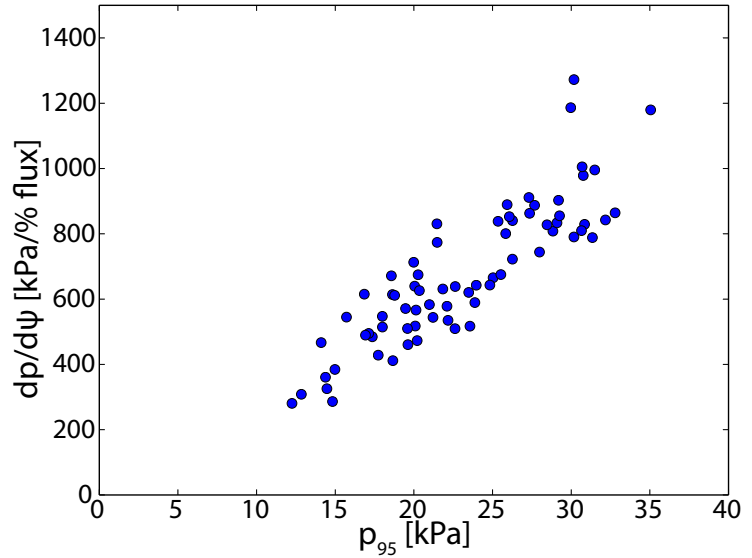
Figure 5.18: Peak \nabla p in the I-mode pedestal versus p_{95} . There is a robust linear dependence between the pedestal gradient and height, consistent with a robust pedestal width.
