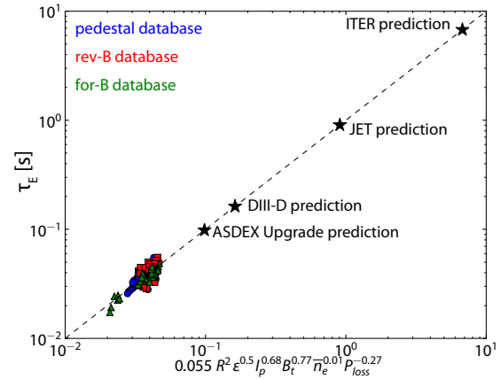
Figure 5.26: Modeled energy confinement time \tau_E with the fixed H-mode-like R^2\sqrt{\varepsilon} size scaling (fit #4 in table 5.1), extrapolated to DIII-D, ASDEX Upgrade, JET, and ITER. Modeled energy confinement times are competitive with H-modes, both the measured \tau_E for existing machines and the expected ITER98y2 prediction for ITER H-modes.
