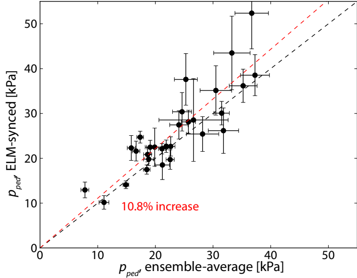
Figure 4.7: Comparison of the pressure pedestal height p_{ped} between the ensemble-averaged and ELM-synchronized profiles. On average, ELM synchronization results in a 10.8% increase in measured pedestal pressure, consistent with ELM losses observed on other machines. At lower pressures, ELMs are typically small enough that the perturbation is minimal; however, the distinction becomes important for the highest-pressure ELMy H-modes on C-Mod.
