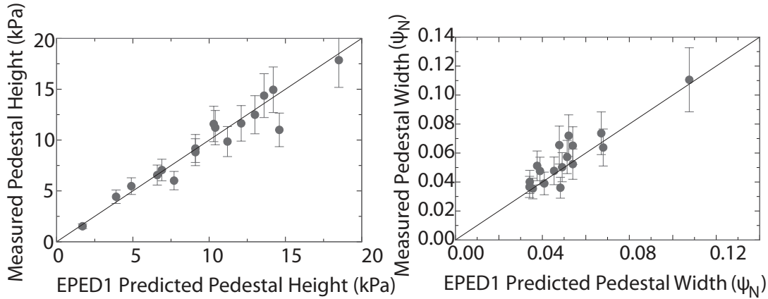
Figure 3.6: EPED 1 predictions versus measured pressure pedestal height and width on a range of DIII-D discharges [57].
