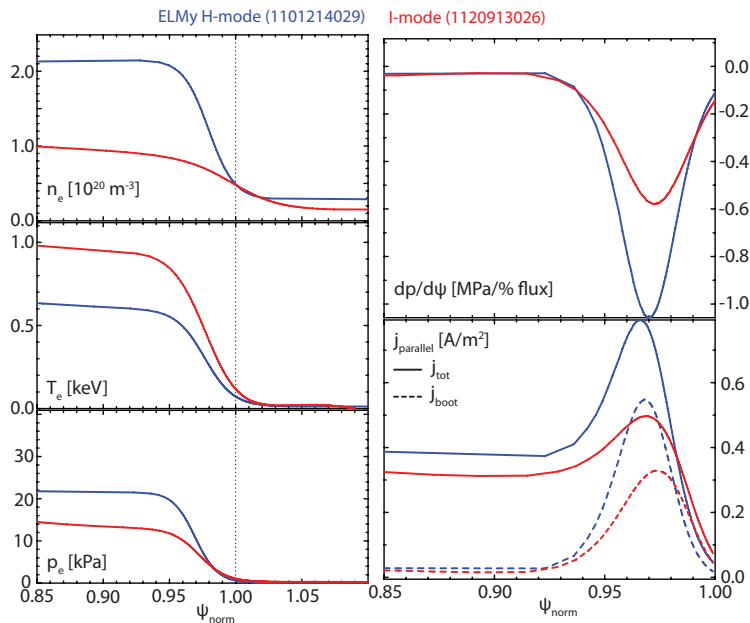
Figure 6.2: Pedestal profiles in I-mode and ELMy H-mode. Due to the steep density gradient in the pedestal, the H-mode exhibits significant pressure gradient and edge current density, which drive the peeling-ballooning MHD instability associated with the ELM trigger. Despite this, the high edge temperature in I-mode allows it to reach an appreciable pedestal pressure.
