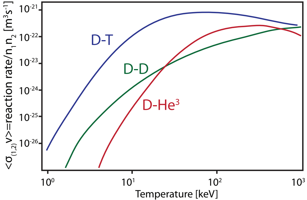
Figure 1.2: Reaction rate normalized to fuel density, expressed as the rate coefficient \langle \sigma v \rangle , for fusion fuels as a function of temperature. Notably, deuterium-tritium fusion exhibits a higher peak reaction rate, as well as reaching that peak at a lower temperature, than other fuels.
