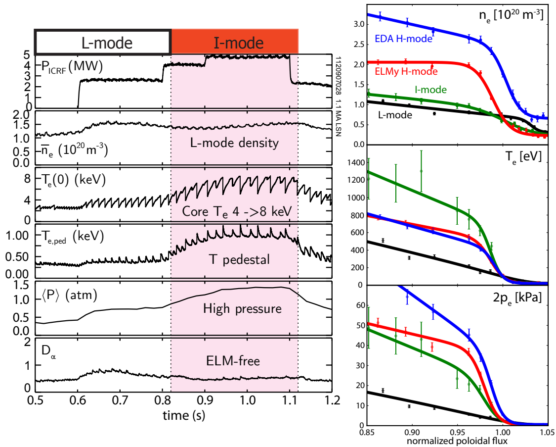
Figure 5.1: (left) Characteristic traces for a typical I-mode. At the L-I transition, the core and edge temperature rise over several sawtooth cycles before reaching a steady level; global confinement and pressure rise accordingly. However, the density remains at L-mode levels, and no ELMs are exhibited. (right) Edge profiles for density, temperature, and pressure in L-, I-, and H-mode. The I-mode (green) retains an density profile comparable to the L-mode (black), unlike the ELMy (red) and EDA (blue) H-modes which form a strong density pedestal. However, the I-mode forms a higher temperature pedestal than either H-mode. As a result, the I-mode reaches comparable pedestal pressures to the H-modes while retaining L-mode particle transport. (repeated from fig. 2.7)
