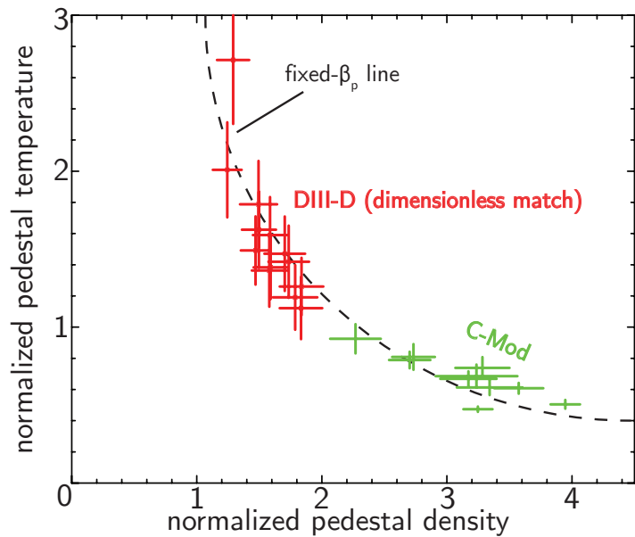
Figure 2.2: ELMy H-mode pedestals from pedestal similarity experiments on Alcator C-Mod and DIII-D. Pedestal densities and temperatures are shown normalized to poloidal field (which accounts for differences in plasma current) such that hyperbolae in the parameter space are curves of constant poloidal beta. ELMy H-mode pedestals are, to lowest order, constrained to a curve of fixed \beta_{p,ped} .
