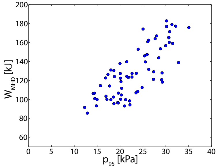
Figure 5.10: I-mode stored energy versus pedestal pressure, confirming the strong dependence of global performance on the pedestal height.
