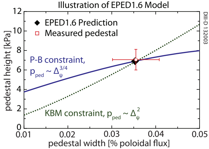
Figure 3.5: Illustration of the peeling-ballooning MHD and kinetic-ballooning turbulent constraints used in the EPED model. The peeling-ballooning constraint, calculated by ELITE, results in a trend roughly of p_{\text{ped}} \sim \Delta_{\psi}^{3/4} , while the KBM width constraint calculated via the ballooning-critical pedestal (BCP) technique sets p_{\text{ped}} \sim \Delta_{\psi}^2 . The unique solution to these constraints is the EPED prediction for the pedestal width and height. The prediction is here shown compared to the measured pedestal from DIII-D shot 132003 (reproduced from [81])
