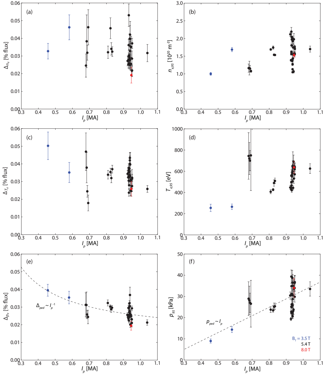
Figure 4.9: Plasma current scalings of the density, temperature, and pressure pedestal widths and heights. Magnetic-field sets are differentiated by color. While the density and temperature pedestals independently show little systematic dependence of their widths on plasma current, the pressure pedestal width shows a exhibits a \Delta_{ped} \sim I_p^{-1} trend. The n_e and T_e pedestal heights both positively trend with current, although with significant scatter – inverse trends between the two are consistent with the zero-th-order approximation of MHD-limited ELMy pedestals lying on a curve of fixed \beta_{p,ped} for a given shaping/field configuration. The pressure pedestal height shows a trend of p_{ped} \sim I_p , such that the pressure pedestal is consistent with the expected \nabla p \sim I_p^2 scaling.
