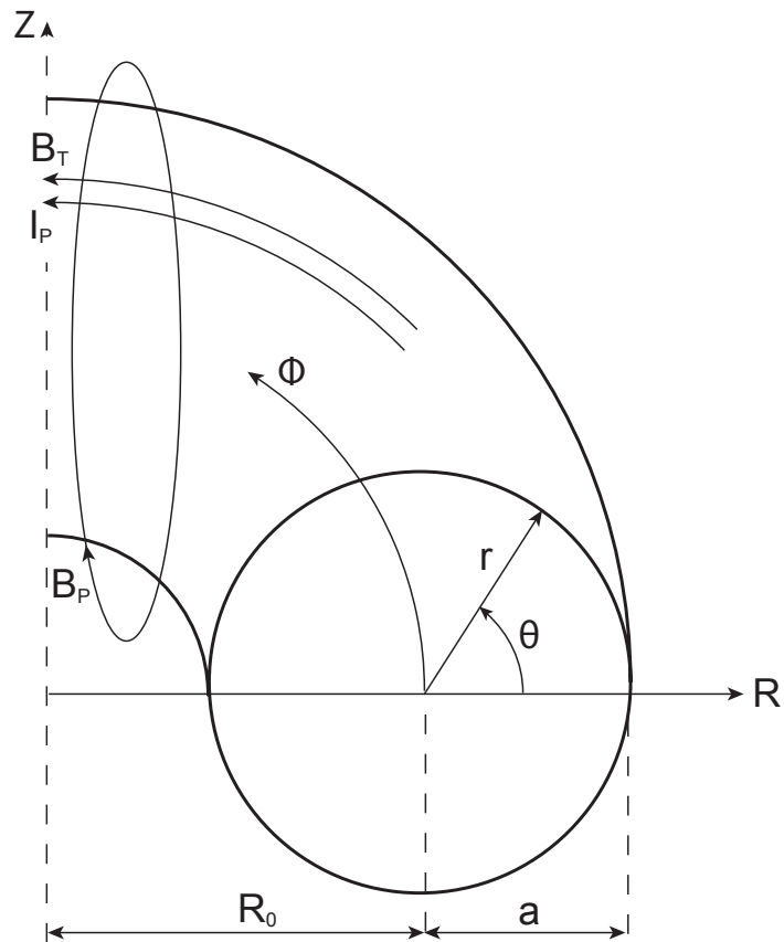
Figure 1.4: Example geometry of a circular-cross-section tokamak plasma, describing a torus of major radius R_0 and minor radius a , with poloidal coordinate \theta and toroidal coordinate \Phi . Tokamak configurations are characterized by an applied toroidal field B_T with a toroidal plasma current I_P , which in turn generates a poloidal magnetic field B_P .
