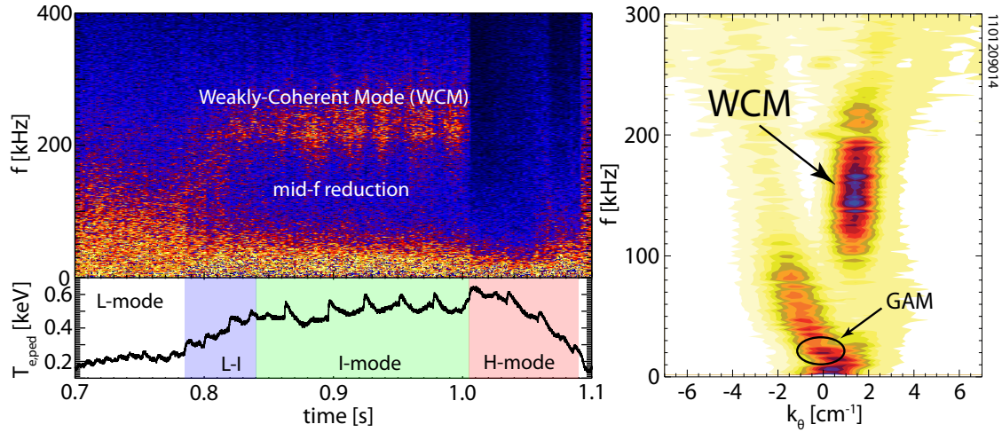
Figure 2.9: Measurements of \tilde{n}_e fluctuations from the WCM in I-mode. (left) Reflectometer measurements in the pedestal region, showing the transition from broadband L-mode turbulence to the WCM, and subsequent fluctuation suppression as the plasma transitions into an ELM-free H-mode. Edge T_e measurements are also shown, tracking the formation of the characteristic I-mode temperature pedestal. Note the dynamics of the L-I transition – while the edge temperature increases steadily over several sawtooth periods, the turbulence suppression and formation of the WCM is more rapid, with the mode spinning up in frequency as the I-mode is established. (right) Gas-puff imaging measurements of the WCM, averaged over the I-mode. The mode is restricted in k -space to k_\theta \sim 1.5 \text{ cm}^{-1} , but is broad in frequency. Also shown is the k_\theta = 0 , f \sim 10 \text{ kHz} signal of the GAM coupled to the WCM [130].
