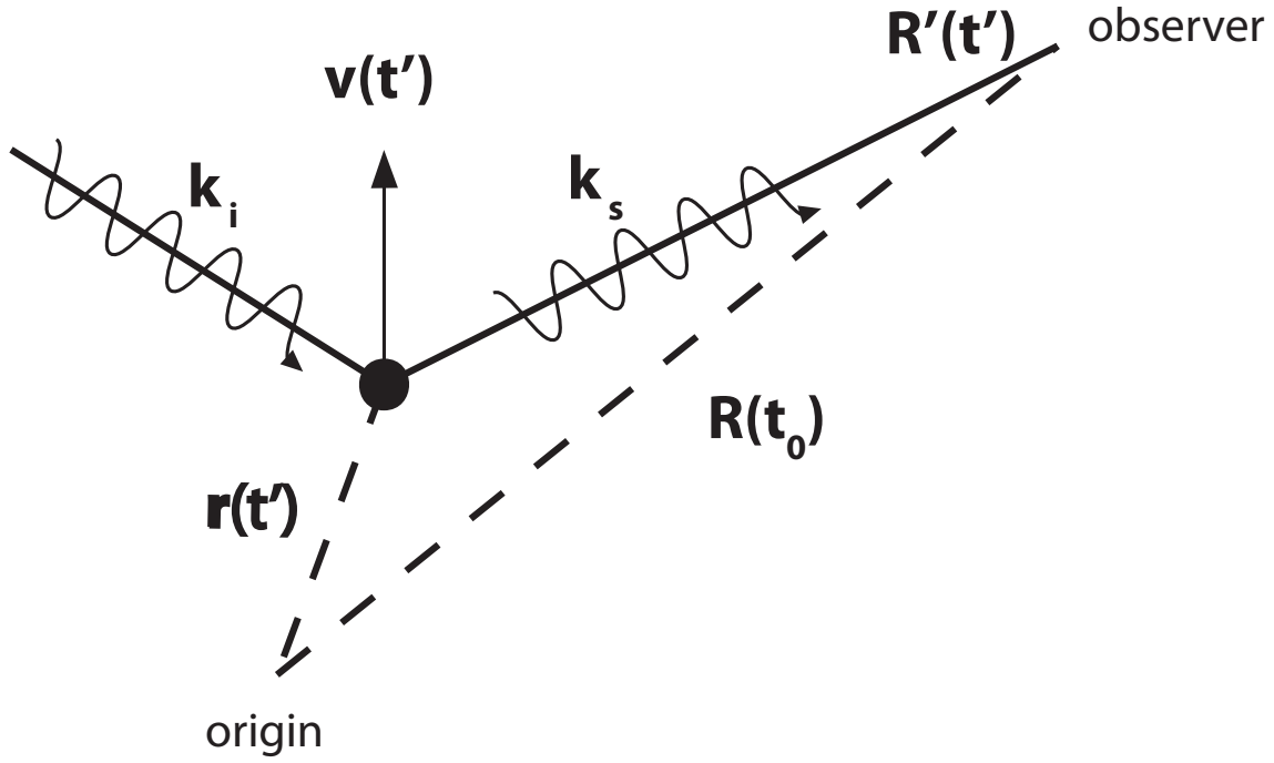
Figure A.1: Coordinate system considered for Thomson scattering, with the incident wave of wavenumber \vec{k}_i incident on a particle at \vec{r}(t') for retarded time t' . The scattered wave \vec{k}_s is drawn to an observer at \vec{R}'(t') .
