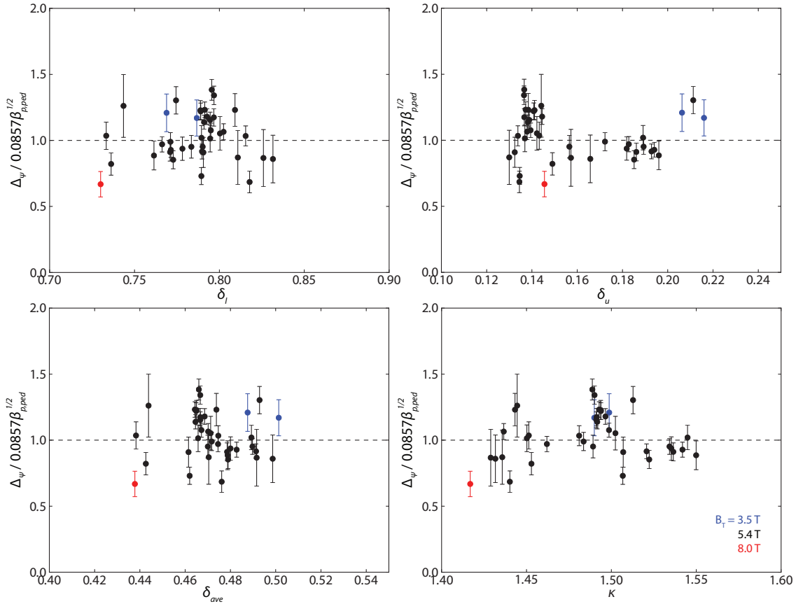
Figure 4.25: Scalings of the pedestal width \Delta_\psi normalized to the dominant scaling \Delta_\psi = 0.0857\beta_{p,ped}^{1/2} with plasma shaping: upper, lower, and average triangularity ( \delta_l, \delta_u, \delta_{ave} = (\delta_u + \delta_l)/2 ), and elongation \kappa . No strong trend with shaping parameters is seen – rather, the influence of plasma shaping arises in the improved MHD stability, such that both \beta_{p,ped} and \Delta_\psi increase with stronger shaping along the KBM-limited curve.
