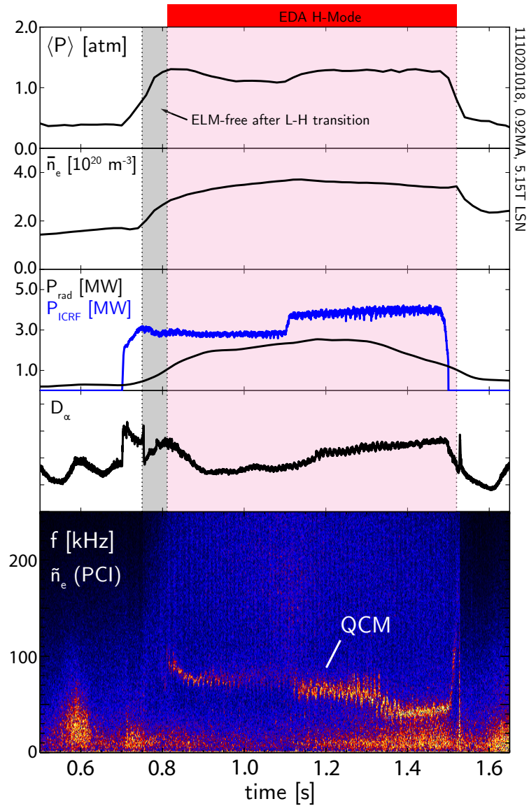
Figure 2.4: Characteristic traces of an EDA H-mode on C-Mod (section 2.3.2). Following a brief ELM-free phase, the plasma density and radiated power stabilizes at a sustainable level. The edge transport barrier is regulated by the continuous QCM fluctuation at \sim 60 - 70 kHz (shown in density fluctuations in the bottom panel) rather than bursty ELM transport.
