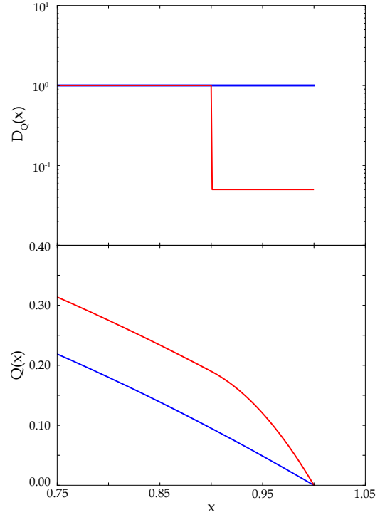
Figure 1.9: Diffusion coefficients and plasma profiles for a “toy model” 1D diffusion equation with a general parameter Q(x) and accompanying diffusion coefficient D_Q(x) , with constant D_Q shown in blue and D_Q reduced by a transport barrier shown in red.
