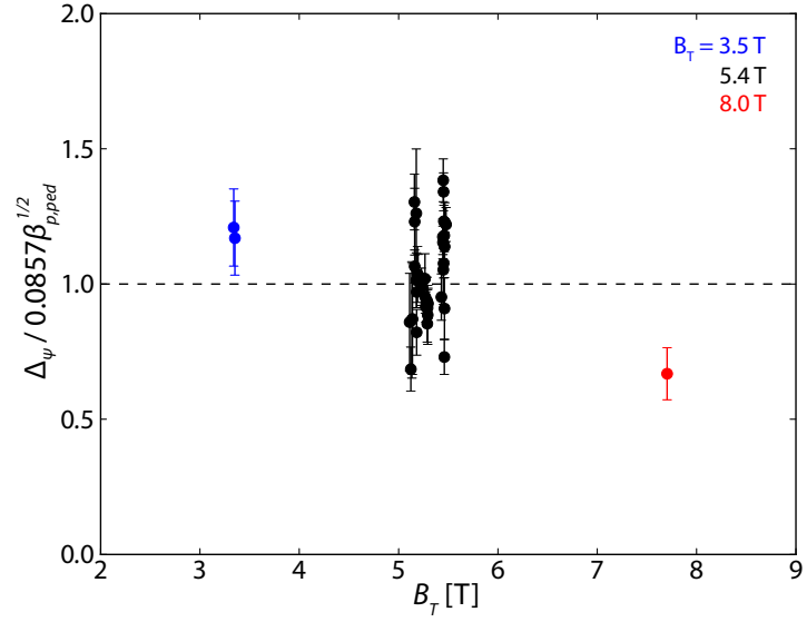
Figure 4.24: Scalings of the pedestal width \Delta_\psi , normalized to the dominant scaling \Delta_\psi = 0.0857\beta_{p,ped}^{1/2} with the applied toroidal field B_T . Although the high scatter at standard B_T and the sparsity of data at low and high field makes a conclusive scaling difficult, there is some indication of an inverse relation of pedestal width with toroidal field.
