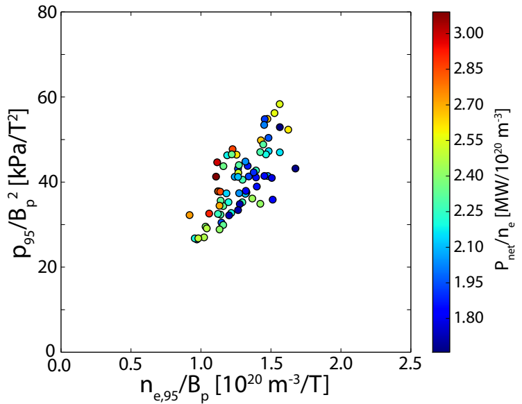
Figure 6.5: Pedestal pressure normalized to poloidal field pressure versus normalized density in I-mode (cf. fig. 6.4(b)). Points are color-coded by power-per-particle, which sets the pedestal temperature – differing values of P_{net}/\bar{n}_e set the slope of the fixed T_e/B_p line. The increase in normalized pressure, then, is not solely due to increased power, but rather indicates a positive response with fueling.
