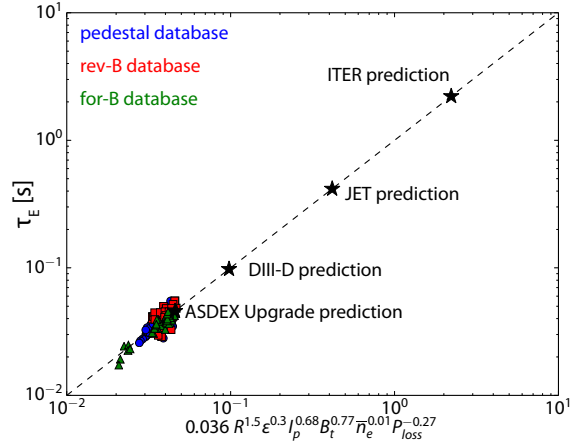
Figure 5.28: Modeled energy confinement time \tau_E with the fixed L-mode-like R^{1.5}\epsilon^{0.3} size scaling (fit #5 in table 5.1), extrapolated to DIII-D, ASDEX Upgrade, JET, and ITER. Modeled energy confinement times are competitive with H-modes, both the measured \tau_E for existing machines and the expected ITER98y2 prediction for ITER H-modes.
