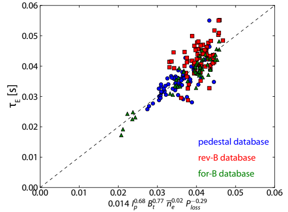
Figure 5.24: Power-law fit for I-mode energy confinement time \tau_E , fitted with the size parameters R and \varepsilon , and elongation \kappa excluded due to the lack of variation in these variables in the available data (fit #3 in table 5.1). Both the high-resolution pedestal database and older reversed-field LSN and forward-field USN I-mode databases are used. This represents the minimum-complexity fit for I-modes on C-Mod, capturing the essential dependences on current, field, and fueling, and notably the weak degradation of confinement with heating power.
