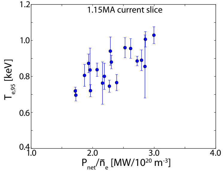
Figure 5.5: Pedestal temperature T_{e,95} vs. heating power per particle ( P_{net}/\bar{n}_e ) for the 1.15 MA current slice, illustrating the approximately-linear trend in temperature at fixed current. This behavior is highly beneficial as an external control for the pedestal temperature.
