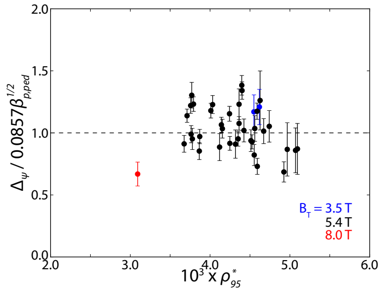
Figure 4.27: Scaling of the normalized pedestal width \Delta_\psi/0.0857\beta_{p,ped}^{1/2} with normalized pedestal gyroradius \rho_{95}^* . Low, standard, and high-field sets are indicated in blue, black, and red respectively. No systematic variation is seen.
