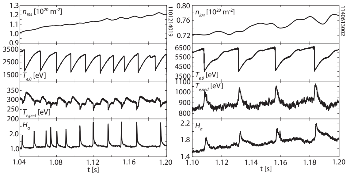
Figure 6.10: Traces of n_{104} , core and edge ( r/a \sim 0.98 ) T_e , and H_\alpha for ELMy H-mode (left) and I-mode (right). ELMs in H-mode (visible on the H_\alpha trace) are independent of the sawtooth cycle, and drive perturbations to the edge temperature and line-integrated density, as both energy and particles are expelled from the plasma by the ELM crash. This is particularly clear on the edge temperature, which exhibits a clear increase with the sawtooth heat pulse and a separate crash with the ELM. I-mode, in contrast, exhibits ELMs (or ELM-like events) that are tied to sawtooth heat pulses reaching the edge, as visible on the ECE T_e signal. No visible crash in edge temperature is visible following the ELM, nor is there a significant perturbation to the density.
