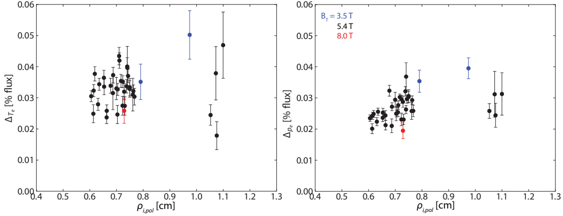
Figure 4.23: Temperature and pressure pedestal widths versus poloidal gyroradius. The temperature pedestal width shows no systematic variation with \rho_{i,pol} . A weak trend is possible in the pressure pedestal width, comparable to the trend of \Delta_p \sim \beta_{p,ped}^{1/2} (due to the strong covariance between \rho_{i,pol} and \beta_{p,ped} ). However, this trend is overruled in favor of a poloidal beta scaling by other observations.
