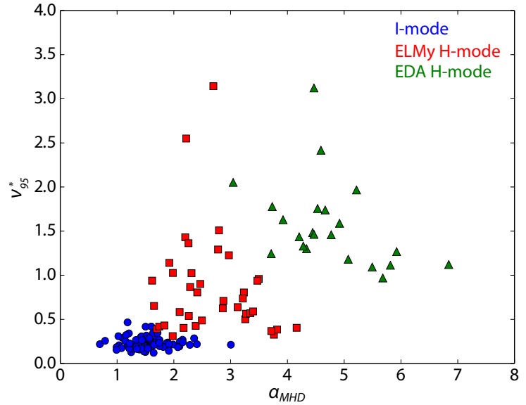
Figure 2.6: Customary parameter range in pedestal collisionality and normalized pressure gradient for I-mode, ELMy H-mode, and EDA H-mode. I-mode is favored by low collisionality, and exhibits the reduces \alpha_{\text{MHD}} associated with stability against ELMs.
