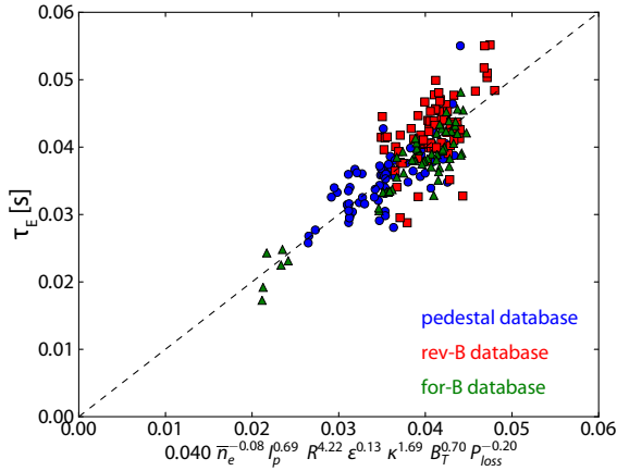
Figure 5.23: Power-law fit for I-mode energy confinement time \tau_E , fitted using the full ITER98y2 parameter set (fit #1 in table 5.1). Both the high-resolution pedestal database and older reversed-field LSN and forward-field USN I-mode databases are used. While the fit is generally good, lack of variation in certain parameters – particularly the size parameters R and \varepsilon (as expected for a single-machine scaling), and elongation \kappa mean that the true variation with these parameters is not accurately captured. However, the expected weak degradation of \tau_E with heating power is captured.
