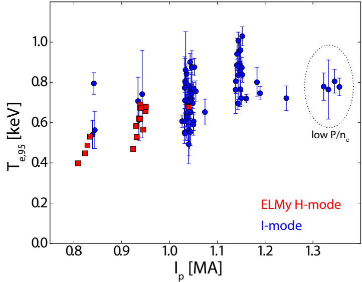
Figure 5.4: Pedestal temperature versus plasma current for I-mode and ELMy H-mode. I-mode temperature pedestals meet or exceed H-mode levels, and trend positively with current. The spread in T_{e,95} at a given current point is due to varying power per particle (see fig. 5.5). The highest-current I-modes exhibit temperatures below the bulk trend due to low values of P_{net}/\bar{n}_e , as these I-modes were fueled to relatively high densities.
