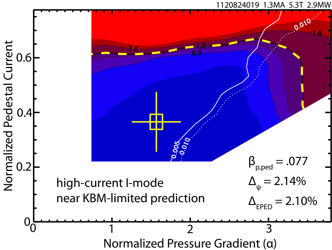
Figure 6.6: Infinite- n ballooning MHD results calculated by BALOO, overlaid on the ELITE results for the same case (see fig. 6.1). The Infinite- n ballooning threshold is taken as a surrogate for the onset of KBM turbulence. Due to the local nature of the infinite- n constraint, BALOO calculates the width in flux space that is locally ballooning-critical – when this reaches half of the pedestal width, the KBM is assumed to be triggered. This case is near the KBM-predicted pedestal width \Delta_{\text{EPED}} , but is nevertheless modeled to be KBM-stable (for \Delta_{\psi} \sim 0.02 , the half-width threshold is the white dotted contour labeled 0.01).
