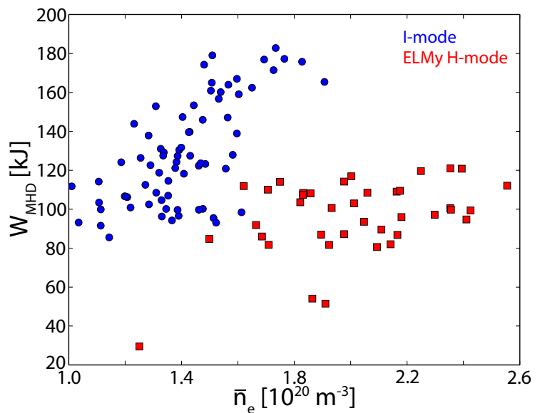
Figure 5.22: Plasma stored energy versus fueling, indicated by \bar{n}_e in I-mode and ELMy H-mode. I-mode stored energy increases strongly with fueling (provided sufficient power to maintain the temperature pedestal), while ELMy H-mode exhibits little trend with density – the global stored energy and average pressure is set by the pedestal beta, which is strongly limited in ELMy H-mode.
