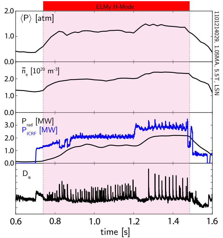
Figure 2.1: Characteristic traces of a steady ELMy H-mode on Alcator C-Mod (section 2.1). Density and radiated power rise after the L-H transition, but stabilize as the periodic relaxation of the pedestal regulates and flushes impurities from the plasma. ELM bursts are visible as spikes on the edge D_\alpha signal.
