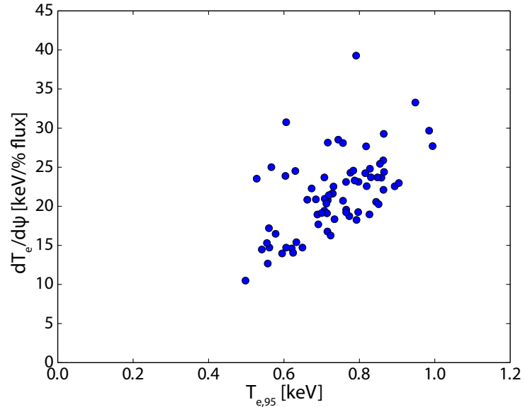
Figure 5.17: Peak \nabla T_e in the I-mode pedestal versus T_{e,95} . Hotter pedestals support a steeper gradient in temperature (albeit with significant scatter), consistent with a robust temperature pedestal width.
