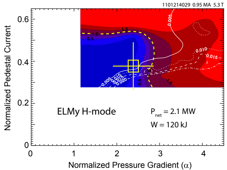
Figure 4.13: Calculation of the peeling-ballooning MHD stability contour from ELITE for an ELMy H-mode pedestal on C-Mod. The red-blue contours show the peeling-ballooning growth rate with diamagnetic stabilization, \gamma/(\omega_{*eff}/2) , while white contours show the width in flux space that is unstable to the KBM. To within error bars, the pedestal lies on the peeling-ballooning boundary. The comparatively higher collisionality typical of C-Mod H-mode pedestals pushes the MHD behavior of the pedestal towards higher-n, pure-ballooning modes, although moderate-n coupled modes in the “nose” of the stability contour are also common.
