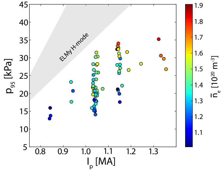
Figure 5.8: Pedestal thermal pressure ( 2 \times p_{e,95} ) versus plasma current, colored by fueling level indicated by line-averaged density \bar{n}_e . The shaded region indicates the typical range of pedestal pressures in C-Mod ELMy H-modes. A strong, roughly p_{95} \sim I_p trend in pedestal pressure is observed. At a given current, a strong increase in pedestal pressure with fueling is also observed (note: heating power also varied in these discharges).
