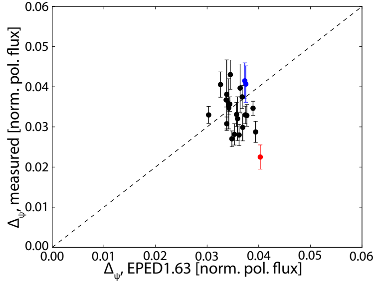
Figure 4.20: Measured EPED pedestal width \Delta_\psi = (\Delta_{n_e} + \Delta_{T_e})/2 in ensemble-averaged pedestals versus EPED1.63-predicted pedestal widths. Magnetic-field groups are indicated by color. The dashed line indicates perfect agreement with EPED prediction. Pedestal widths are robust on C-Mod, restricted to \sim 2 - 5\% of poloidal flux. The EPED model reproduces this trait within expected prediction error.
