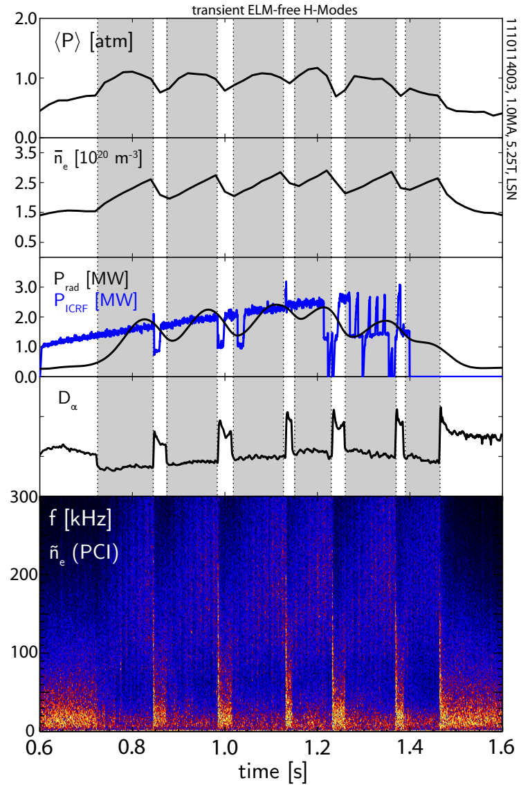
Figure 2.3: Characteristic traces of transient ELM-free H-modes, highlighted on the traces (section 2.2). After the L-H transition, density and thermal pressure (and therefore fusion reaction rate and stored energy) rise, while turbulent particle transport is reduced, as seen by the drop in edge D_\alpha light and suppression of turbulence (shown in the density fluctuations). However, radiated power rises due to impurity accumulation – when radiated power reaches a level comparable to total heating power, the plasma drops back into L-mode.
