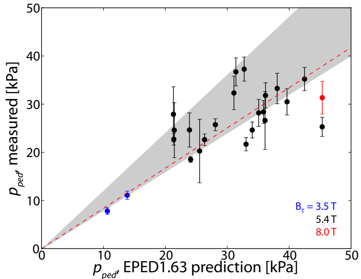
Figure 4.14: Pressure pedestal height predicted by EPED1.63 versus the measured (ensemble-averaged) pedestal height, color-coded by magnetic field set. The grey band indicates agreement within the \pm 20\% typical prediction accuracy for EPED. The EPED model systematically over-predicts the pedestal pressure, with an average ratio of measured to predicted pedestal heights of 0.835 \pm 0.036 (indicated by the red line).
