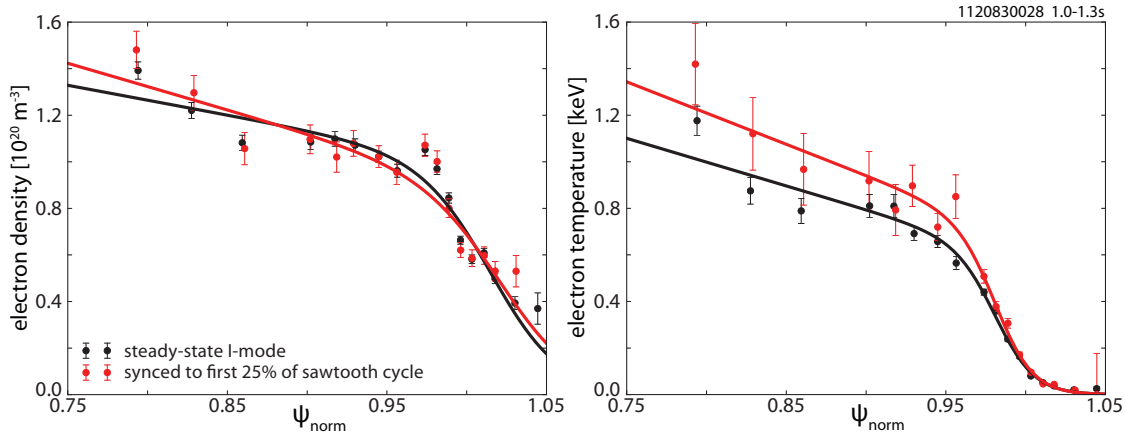
Figure 6.8: Profiles of n_e and T_e in the I-mode pedestal, with the full ensemble-averaged data (black) compared to data masked to the first 25% of the sawtooth cycle following the heat pulse reaching the edge. The sawtooth does not meaningfully perturb the density profile, but triggers a measurable transient increase in the temperature pedestal.
