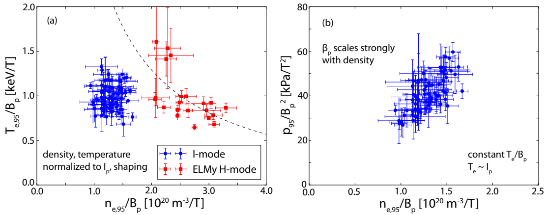
Figure 6.4: Pedestal temperature (left) and pressure (right) versus pedestal density. Parameters are normalized to the edge poloidal field – this accounts for plasma-current variation in the datapoints, as well as allowing a natural representation of MHD boundaries. (a) Pedestal temperature vs. density for I-mode and ELMy H-mode. Due to the poloidal-field normalization, hyperbolae in the parameter space are curves of constant \beta_{p,ped} . ELMy H-modes lie, to lowest-order approximation, on a \beta_{p,ped} -limited curve (indicated by the dashed line) with the expected inverse relationship between density and temperature; I-mode n_e and T_e , however, are uncorrelated. (b) Pedestal pressure normalized to poloidal field pressure versus normalized density in I-mode. Pedestal poloidal beta trends linearly with (normalized) density, rather than lying on the \beta_{p,ped} -limited line expected for MHD-limited pedestals, consistent with the strong response of the I-mode pedestal to fueling (see section 5.2.2). I-mode data lie on a line of constant T_e/B_p , consistent with the observed T_{e,ped} \sim I_p seen in section 5.2.1.
