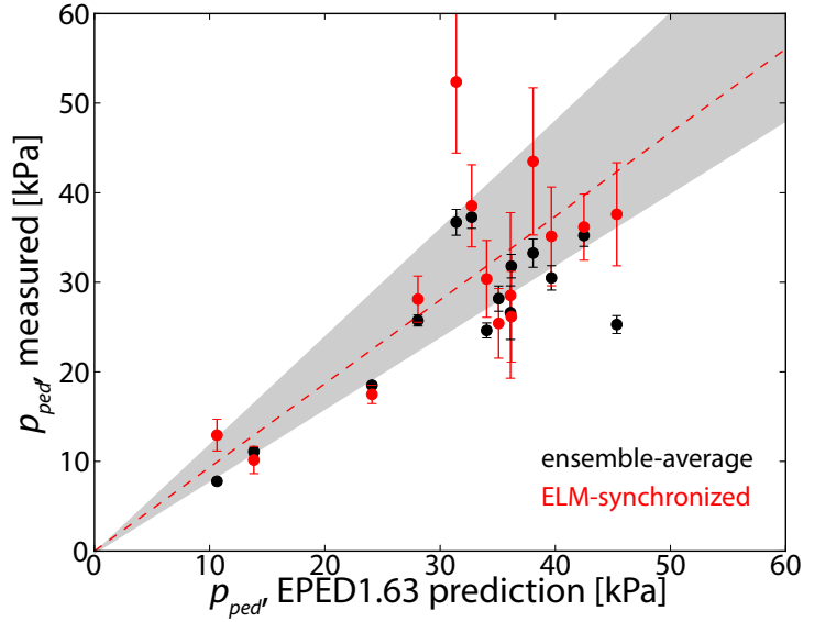
Figure 4.15: Pressure pedestal height predicted by EPED1.63 versus measured, ELM-synchronized pedestal height (red, with corresponding ensemble-average points shown in black). The grey band indicates agreement within the \pm 20\% typical prediction accuracy for EPED. ELM synchronization brings the measured pedestal height into better agreement with EPED predictions, with a correspondence of 0.934 \pm 0.066 (indicated by the red dash).
