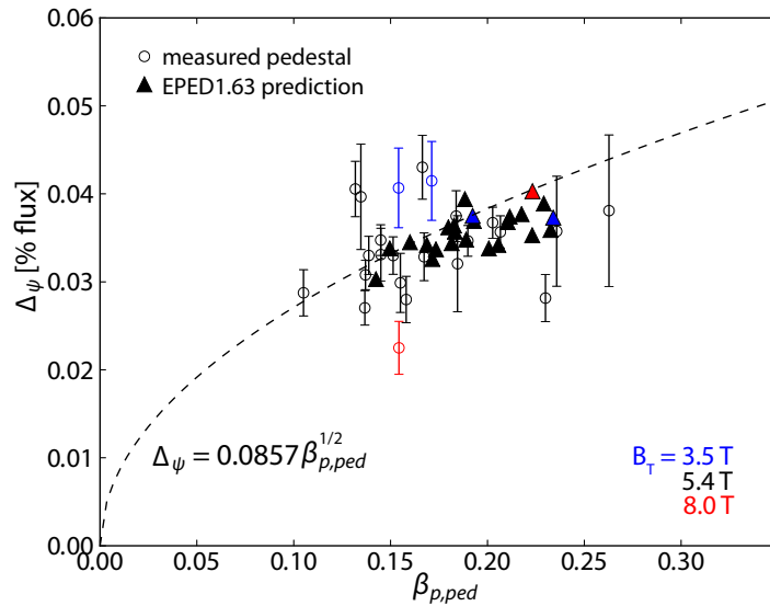
Figure 4.17: Comparison of EPED1.63-predicted pedestal width \Delta\psi and height \beta_{p,ped} with the corresponding ensemble-averaged experimental points, with the KBM scaling \Delta\psi = c\beta_{p,ped}^{1/2} . Though the EPED predictions were calculated with a self-consistent treatment of the scale factor c as a weakly-varying function of plasma parameters, the result is quantitatively similar to the simple fixed scale factor.
