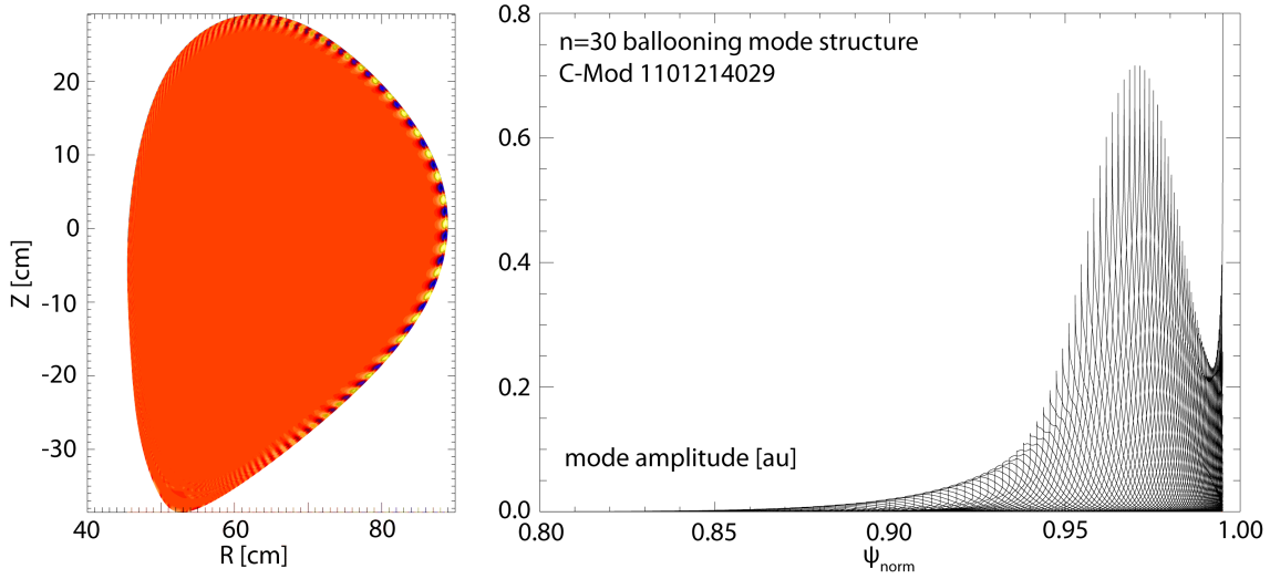
Figure 3.3: Mode structure for an n = 30 ballooning mode calculated by ELITE. (left) Contour plot of radial perturbations from the mode. The mode is edge-localized and strongest at the outboard midplane, consistent with an edge ballooning mode. (right) Eigenmode structure of the n = 30 mode. Each peak is a poloidal harmonic localized around the rational flux surface determined by the corresponding poloidal mode number m for n = 30 . The mode is strongest in the steep gradient region, but extends inward due to the comparatively high mode number (eigenmode envelope encompasses O(n^{1/3}) flux surfaces). Note that, as ELITE cannot treat the separatrix, the mode calculation truncates at \psi_{\text{norm}} = 0.995 .
