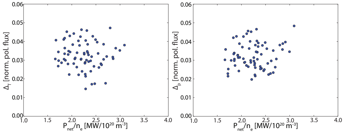
Figure 5.16: Temperature (left) and pressure (right) pedestal widths versus power-per-particle, P_{\text{net}}/\bar{n}_e , i. e., the heat flux through the pedestal. No correlation is seen.
