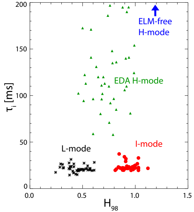
Figure 2.8: Impurity confinement time \tau_I measured by laser blow-off [126] versus normalized confinement H_{98} for L-mode, I-mode, and H-mode. I-mode exhibits H-mode-like energy confinement, increased by roughly a factor of two over L-mode. However, I-mode retains L-mode levels of particle and impurity transport, readily flushing heavy impurities from the plasma. EDA H-mode exhibits strongly increased particle confinement, while transient ELM-free H-modes increase their particle confinement to the point of radiative collapse (see section 2.2)
