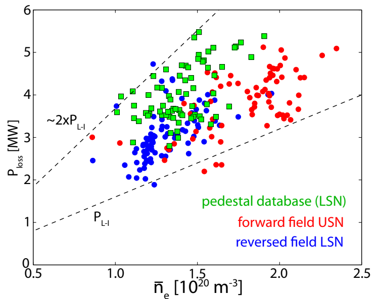
Figure 5.3: Line-averaged density and loss power range for USN and LSN I-modes, illustrating \sim 2 \times P_{L-I} range for I-mode access. USN shapes are forward-field and LSN-shapes are reversed field, such that all I-modes shown are in the unfavorable drift configuration. Data from the high-resolution pedestal database (all are LSN reversed-field) are highlighted.
