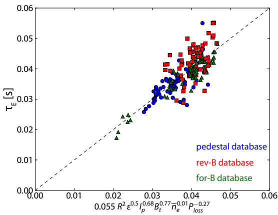
Figure 5.25: Power-law fit to I-mode energy confinement time \tau_E , with the ansatz of an H-mode-like R^2\sqrt{\varepsilon} size scaling fixed (fit #4 in table 5.1). Both the high-resolution pedestal database and older reversed-field LSN and forward-field USN I-mode databases are used. Note the expected weak degradation of \tau_E with heating power.
