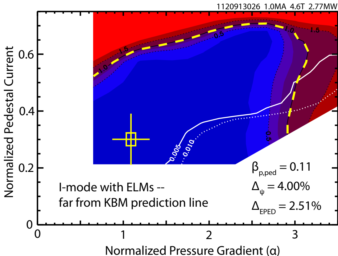
Figure 6.7: Infinite- n ballooning MHD results calculated by BALOO, overlaid on the ELITE results for the same case (see fig. 6.3). This case exhibited sawtooth-triggered ELM-like events. This case is substantially wider than the KBM-predicted pedestal width \Delta_{EPED} , and is modeled to be strongly KBM-stable – in fact, the BALOO assay could not calculate enough ballooning-unstable rational surfaces to draw the contour for the BCP-predicted threshold of 0.02.
