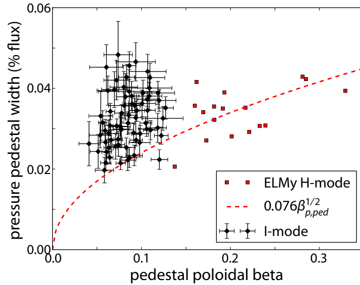
Figure 5.12: Pedestal width versus poloidal beta in I-mode and ELMy H-mode. ELMy H-modes lie on the \Delta\psi \sim \beta_{p,ped}^{1/2} line predicted for KBM-limited pedestals (see section 4.4.2). I-mode shows no scaling of the pedestal width with \beta_p , and exhibits pedestals consistently wider than predicted for comparable ELM-limited pedestals.
