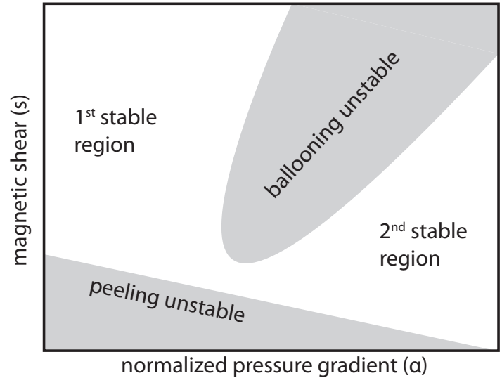
Figure 3.1: Schematic in s - \alpha_{\text{MHD}} space of the infinite- n peeling and ballooning instabilities. The ballooning instability (see section 3.2.1) is destabilized by increasing pressure gradient and stabilized by magnetic shear. A second-stable region for the ballooning mode is found at very high pressure gradient, which can be accessed by increasing the pressure gradient at low magnetic shear. The peeling instability is driven by large edge current density (equivalently, low magnetic shear), and is stabilized by increased pressure gradient.
