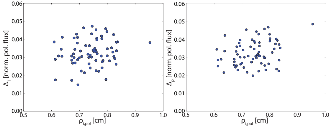
Figure 5.13: Temperature (left) and pressure (right) pedestal widths versus poloidal gyroradius \rho_{i,pol} . No correlation in the pedestal width is seen, contrary to models suggesting a scaling of the sheared-flow layer and pedestal with the gyroradius.
