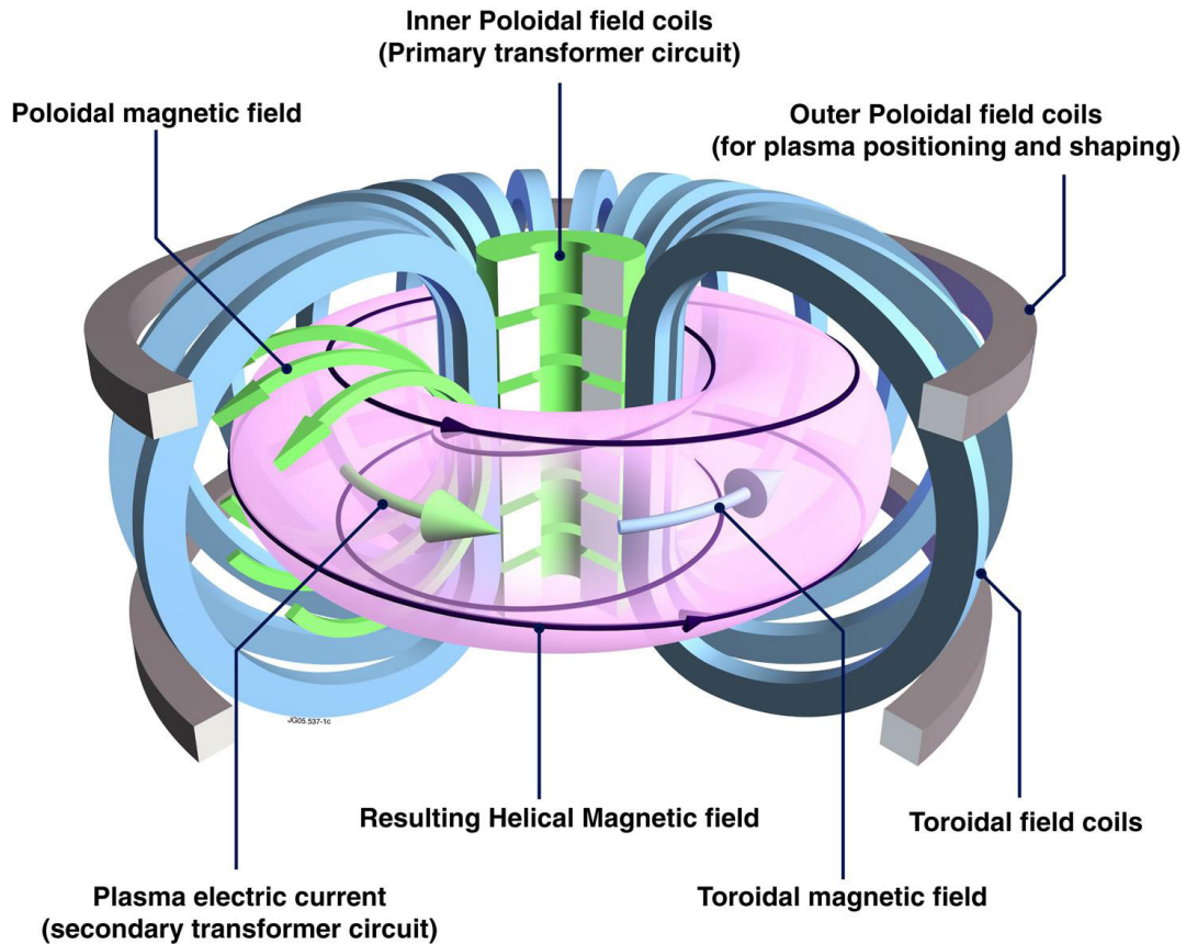
Figure 1.5: Schematic of a tokamak configuration, showing the plasma and magnetic coils. The applied toroidal magnetic field is generated by the toroidal field coils (shown in blue). A toroidal plasma current is generated by the center transformer, in turn generating a poloidal magnetic field (shown in green). These combine to form the helical magnetic field. The plasma shape and equilibrium is adjusted with the outer poloidal field coils (gray).
