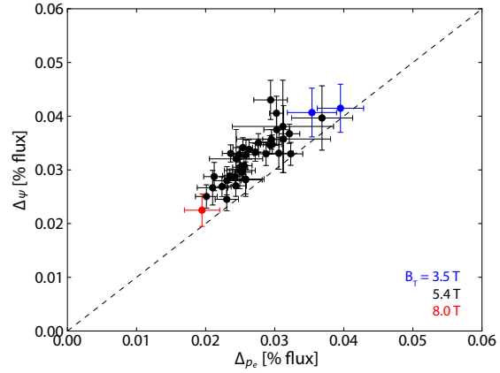
Figure 4.6: Comparison of the directly-measured pressure pedestal width and the EPED width \Delta_\psi defined as the average of \Delta_{n_e} and \Delta_{T_e} . The widths trend quite closely to one another, although \Delta_\psi is systematically somewhat wider.
