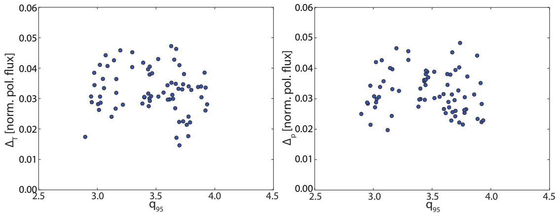
Figure 5.15: Temperature (left) and pressure (right) pedestal widths versus edge safety factor q_{95} . No correlation is seen.
