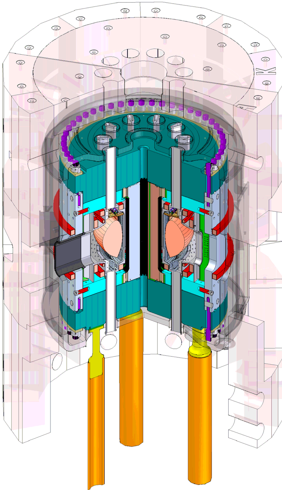
Figure 1.7: Cutaway view of the Alcator C-Mod tokamak, including cryostat and ancillary structures, illustrating the extensive support structures necessary for compact, high-field operation.
