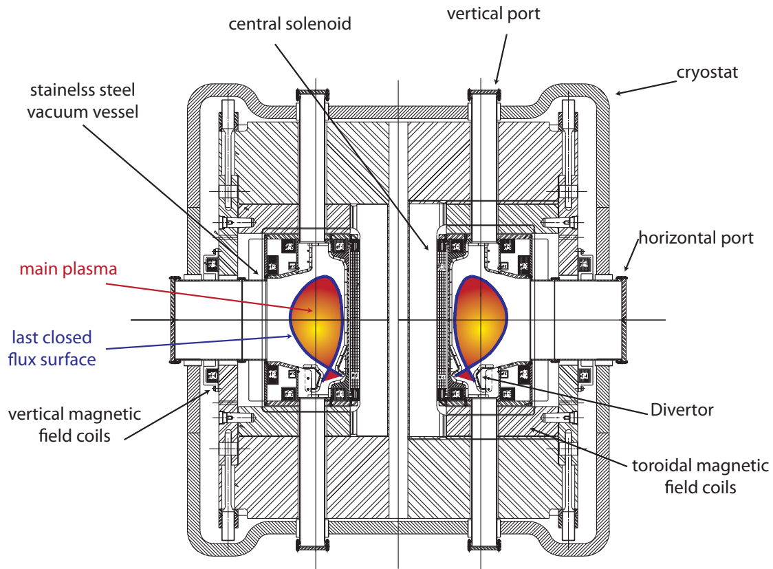
Figure 1.8: Cross-section of the C-Mod vacuum vessel, cryostat and diagnostic access ports, with toroidal-field and equilibrium-field magnetic coils labeled. Also shown is the plasma position in a typical LSN shape, with strike points in the lower divertor shown.
