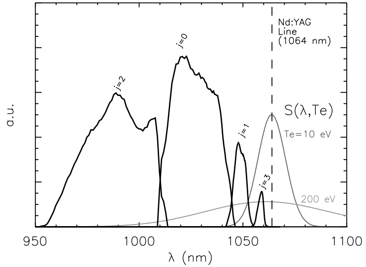
Figure A.5: Normalized spectral response functions of the edge TS polychromator bandpasses, compared to characteristic scattered spectra at 10 eV and 200 eV.
