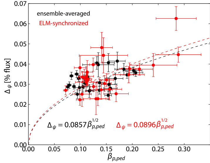
Figure 4.18: Comparison of ensemble-averaged (black) and ELM-synchronized (Red) pedestal width and height, compared to the KBM constraint. The \Delta\psi = 0.0857\beta_{p,ped}^{1/2} scaling found in the ensemble-averaged case is shown in black, while the minor modification of \Delta\psi = 0.0896\beta_{p,ped}^{1/2} for the ELM-synced cases is shown in red.
