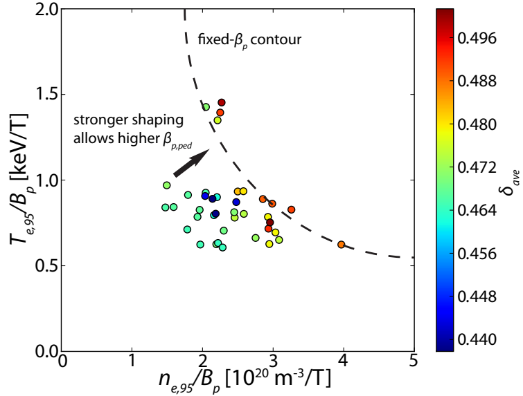
Figure 4.12: Pedestal density vs. temperature normalized to poloidal field (accounting for variation in plasma current) such that hyperbolae in the parameter space are curves of fixed \beta_{p,ped} . At a given shaping, ELMy H-mode pedestals are to lowest order constrained to fixed \beta_{p,ped} , with stronger shaping allowing greater attainable \beta_p .
