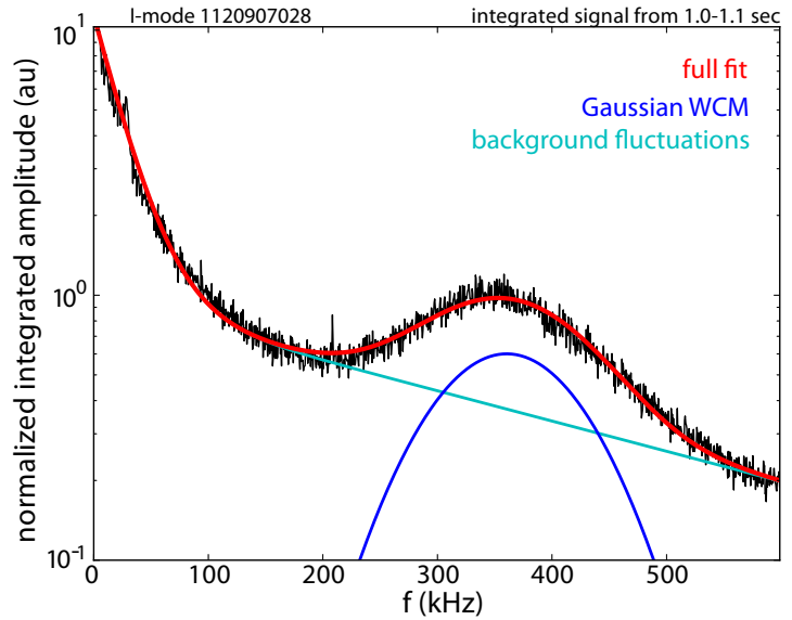
Figure A.6: Time-integrated fluctuation intensity for a steady I-mode phase, fitted as a function of frequency to the form in eq. (A.48). The Gaussian fit to the WCM is shown in blue, with the exponentially dropoff in background fluctuations is shown in teal. The full fit is shown in red.
