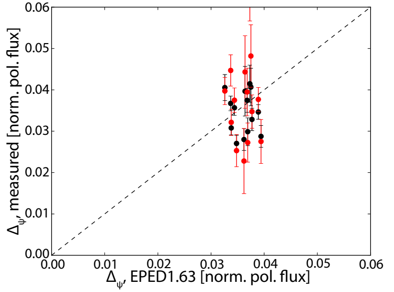
Figure 4.21: Measured pedestal width \Delta_\psi versus EPED1.63 predicted width. Ensemble-averaged points are shown in black, while corresponding ELM-synchronized points are shown in red. ELM-synced pedestals are typically somewhat wider, although still lie within the \pm 20\% expected error for EPED.
