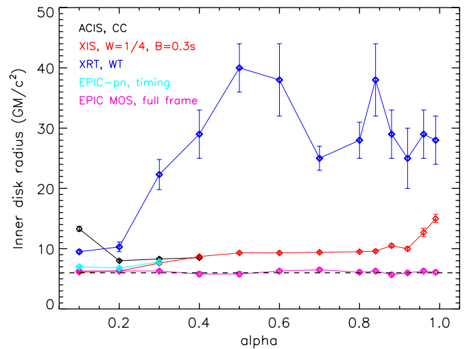
Figure 1. Plot above depicts the evolution of the inner disk radius measured via a relativistic iron emission line (in units of GM/c^2 ) vs. the severity of photon pile-up (governed by the grade migration parameter \alpha ), for simulated spectra assuming a form typical of the “very high” state in accreting black holes (see Section 5 and Table 1). The dashed horizontal line at 6GM/c^2 denotes the input radius used in all simulated spectra. An iron line could not be required in fits to simulated Chandra /ACIS “continuous clocking” mode spectra past \alpha = 0.92 , nor above \alpha > 0.3 for fits to simulated EPIC-pn spectra. Fits to simulated EPIC MOS spectra do not show an evolution in radius because pile-up is so severe that event loss dominates over grade migration distortions; this is a limitation of our simulations and it does not suggest that the MOS should be operated in “full frame” to observe a source this bright. The results above suggest that the Suzaku /XIS (with a 1/4 window and 0.3 s burst option) and Swift /XRT (in windowed timing mode) are capable of dealing with flux levels this high but would give falsely large disk radii unless pile-up distortions were mitigated (e.g., by extracting counts in annuli).
