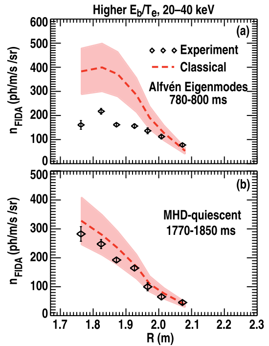
FIG. 16. FIDA density profiles from the higher E_b/T_e cases for (a) an early time during which Alfvén eigenmodes are present, and (b) during the MHD-quietest period. The red dashed lines represent the classically expected FIDA density as computed by the synthetic diagnostic FIDASIM. The uncertainty ribbon about the simulation trace represents a 25% range.
