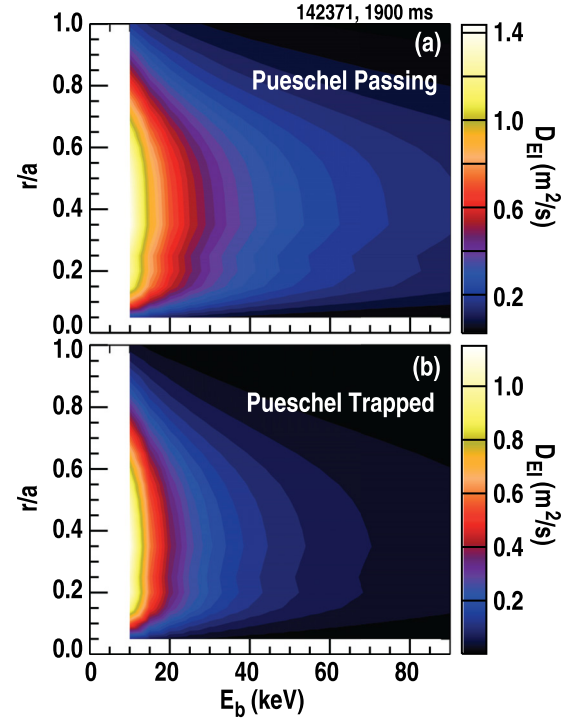
FIG. 18. Values of D_{EI} calculated using the Pueschel formulation for the lower E_b/T_e case of shot 142371.
