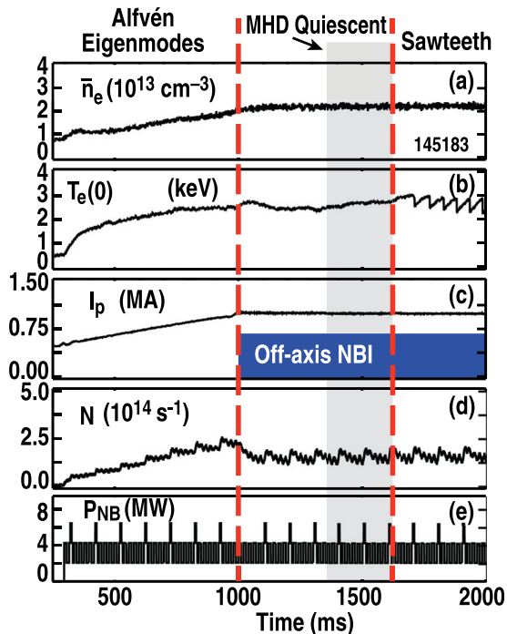
FIG. 1. Time evolution of plasma parameters from shot 145183 indicating the regions of energetic ion transport mechanisms and the presence of off-axis NBI. (a) Line-averaged density, (b) central electron temperature, (c) plasma current, (d) neutron rate, and (e) neutral beam power.
