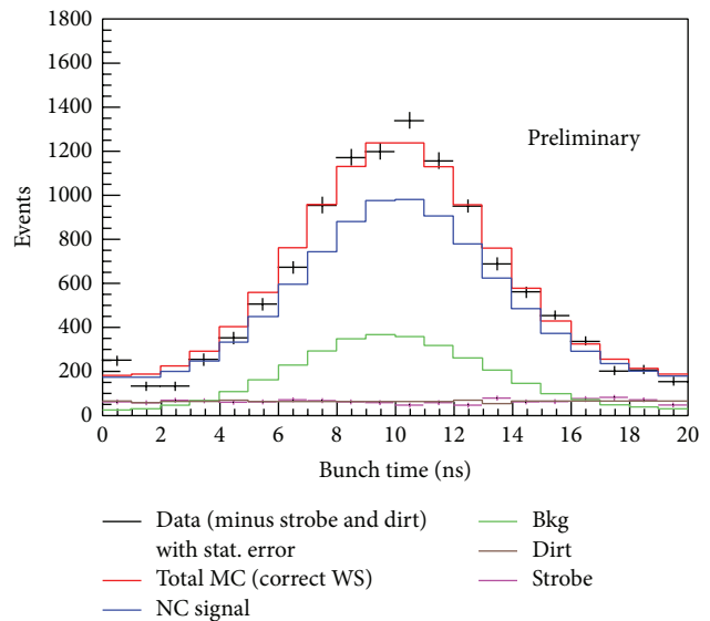
FIGURE 18: (Color online) The reconstructed NCE event time profile for the antineutrino mode beam. The events are overlaid relative to the bunch center. As expected, the data peaks in the bunch center, which means these are dominated with antineutrino interactions and there is no delay of events.
