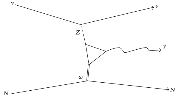
FIGURE 8: The triangular anomaly mediated photon production. The neutrino neutral current couples via Z-boson, and the target nucleon or nucleus couples with a strong force mediated vector meson, such as an omega meson.
