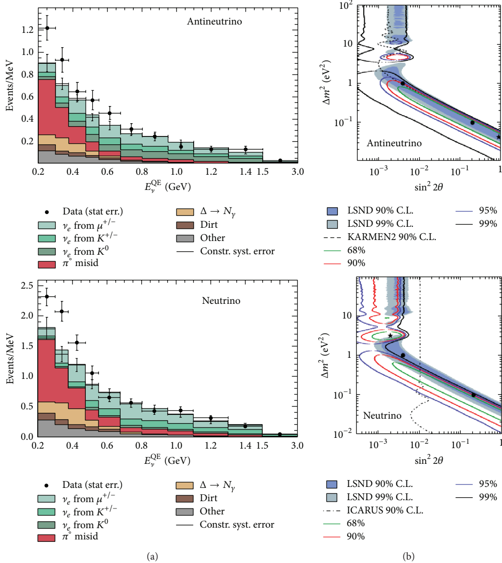
FIGURE 7: (Color online) The final MiniBooNE oscillation results [58]. (a) shows the reconstructed neutrino energy distribution of oscillation candidate events. The top is for antineutrino mode and the bottom is for neutrino mode. (b) shows the allowed region in \Delta m^2 - \sin^2 2\theta , where the best fit points are shown in black stars.
