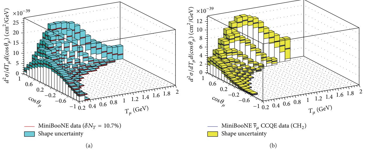
FIGURE 3: (Color online) MiniBooNE CCQE cross sections. (a) shows the muon neutrino flux-integrated CCQE double differential cross section on a neutron target. (b) shows muon antineutrino flux integrated CCQE double differential cross section on a \text{CH}_2 molecule.
