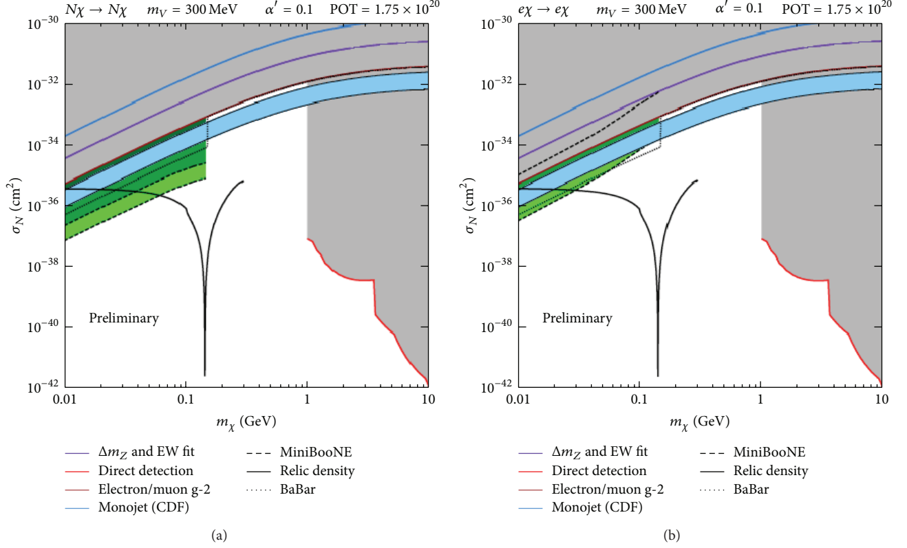
FIGURE 15: (color online) The MiniBooNE dark matter particles search phase space [116]. Here, the x -axis is the dark matter mass m_\chi , and the y -axis is either the dark matter-nucleon or dark matter-electron cross section, assuming the vector mediator mass and the gauge coupling ( m_V = 300 MeV and \alpha' = 0.1 ). The MiniBooNE exclusion region can be seen in green.
