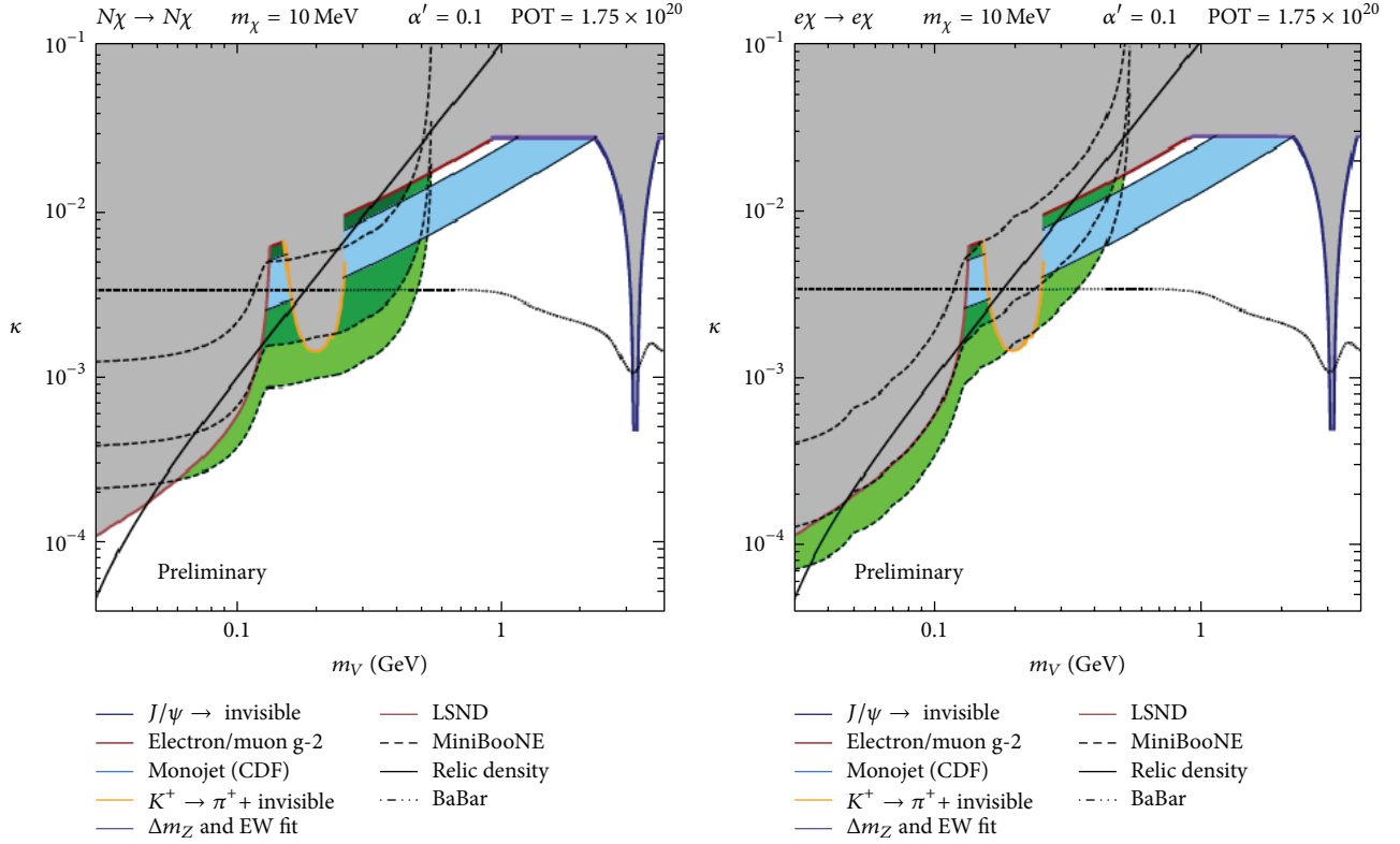
FIGURE 16: (Color online) The MiniBooNE dark matter search phase space [116]. Here, x -axis is the vector mediator mass m_V , and the y -axis is the kinetic mixing parameter \kappa , assuming the dark matter mass and the gauge coupling ( m_\chi = 10 MeV and \alpha = 0.1 ). MiniBooNE exclusion region can be seen in green.
