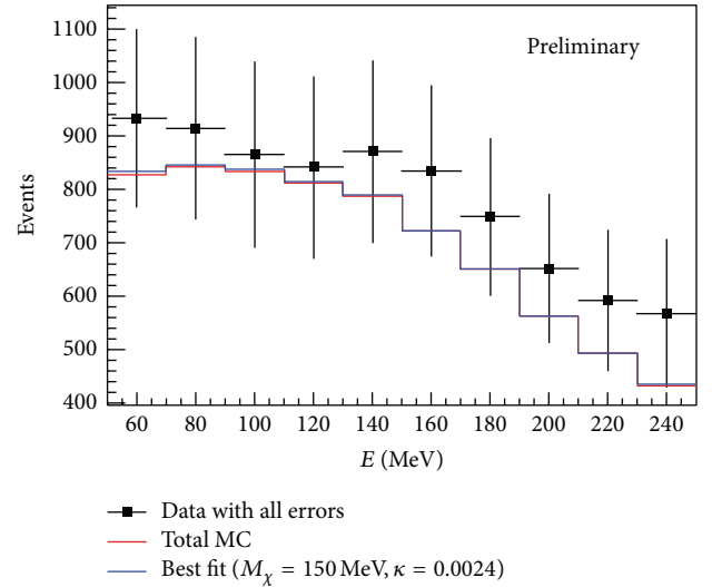
FIGURE 13: (Color online) The dark matter fit result to the NCE data [116].
