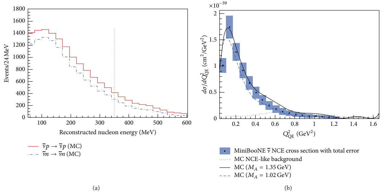
FIGURE 5: (Color online) MiniBooNE NCE results [45]. (a) shows simulated kinetic energy of protons and neutrons from NCE in MiniBooNE. The line denotes the Cherenkov threshold, that is, only protons which have higher energy from this line emit Cherenkov radiation. (b) shows the antineutrino NCE differential cross section. As you see, the data shows a “roll-over” in the low Q^2 region.
