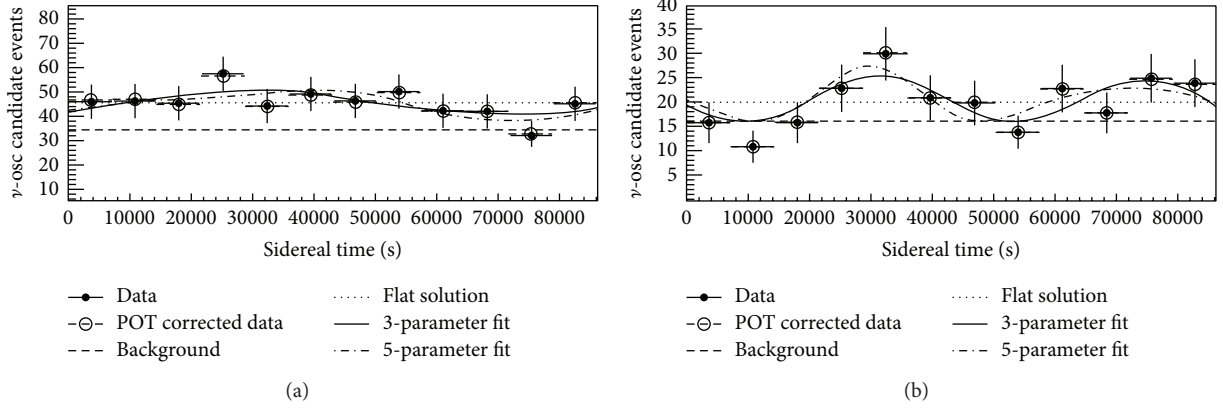
FIGURE 12: The MiniBooNE Lorentz violation results [103]. (a) shows the neutrino mode electron-like low energy excess sidereal time distribution, and (b) shows the antineutrino mode sidereal time distribution. Here, the data with a POT correction (open circle) show the size of the beam day-night variation. There are three fit curves based on different assumptions, a flat solution (dotted), a three-parameter fit (solid curve), and a full five-parameter fit (dash-dotted curve).
