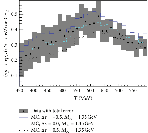
FIGURE 6: (Color online) The ratio of \nu p \rightarrow \nu p to \nu N \rightarrow \nu N as a function of the reconstructed total kinetic energy of nucleons [10].
