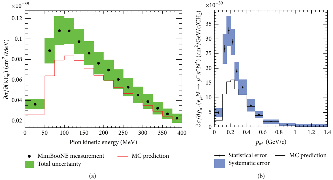
FIGURE 4: (Color online) MiniBooNE single pion production results. (a) is \pi^+ kinetic energy differential cross section from \text{CCl}\pi^+ interaction on \text{CH}_2 [8]. (b) is \pi^0 momentum differential cross section from \text{CCl}\pi^0 interaction in \text{CH}_2 [9]. As you see, predictions underestimate data for both channels and the shapes do not agree as well.
