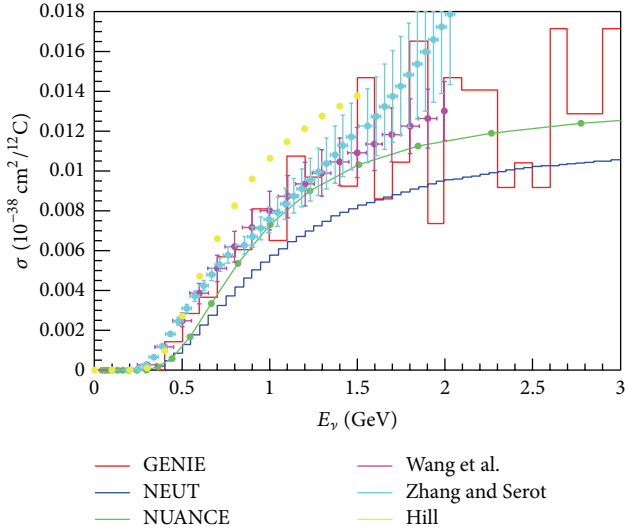
FIGURE 9: (Color online) A comparison of the total cross section of NC photon production per ^{12}\text{C} nucleus [68]. The neutrino interaction generators used by experimentalists (GENIE [13], NEUT [14], and NUANCE [11]) tend to predict lower cross sections than state-of-the-art theoretical models (Wang et al. [65], Zhang and Serot [69], Hill [64]).
