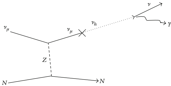
FIGURE 10: The concept of a heavy neutrino decay signal in the MiniBooNE detector [73]. The mixing of a neutrino with a hypothetical heavy neutrino and its short life time allows for it to decay in the MiniBooNE detector to leave a photon signal.
