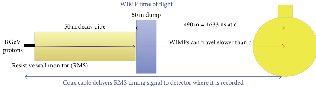
FIGURE 17: (Color online) The concept of dark matter particles TOF. Because of the localization of the dark matter particle production in time and in space, the dark matter beam has well-defined timing structure.
