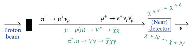
FIGURE 14: (Color online) The concept of the dark matter beam in MiniBooNE [116]. The dominant production mode of dark matter particles is decays of the mediator particles created by decays of neutral mesons. The dark matter particles can be also made through the direct collisions of protons on the beam dump.
