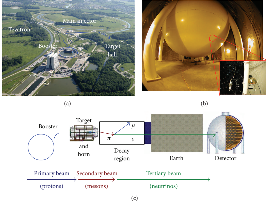
FIGURE 1: The MiniBooNE experiment layout [4]. (a) The Fermilab accelerator complex. (b) The MiniBooNE detector, with inset showing the black inner volume and the white outer volume. (c) Schematic layout of the beam and detector [18].
