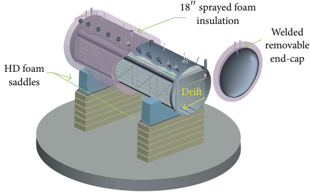
FIGURE 11: (Color online) A drawing of MicroBooNE cryostat [53]. The 170 ton cryostat contains the 89 ton TPC.
