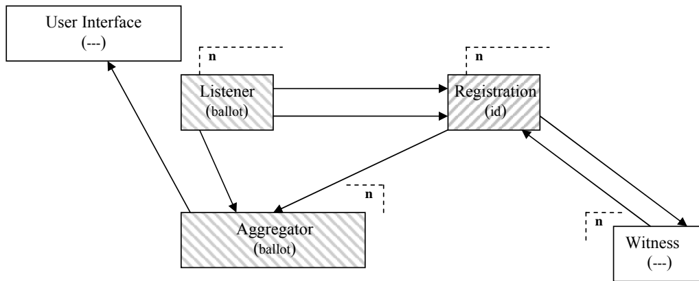
Figure 3.3: Knowledge Separation
