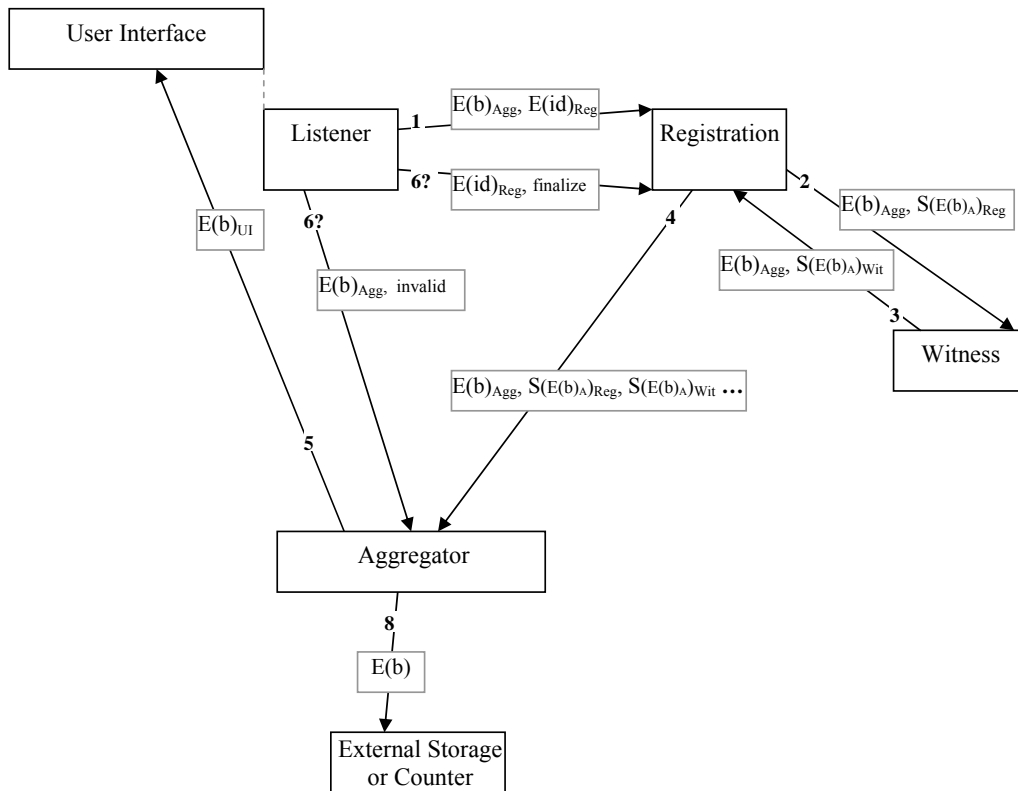
Figure 3.2: Voting Process
