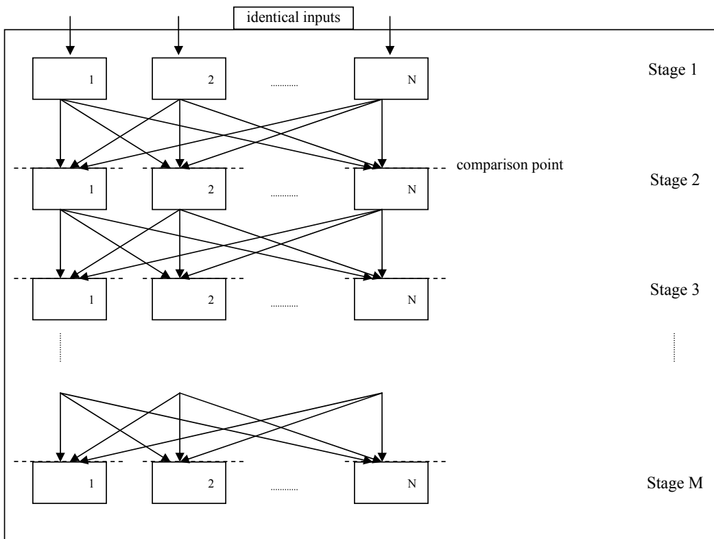
Figure 2.1: Generalization of SAVE communication network
