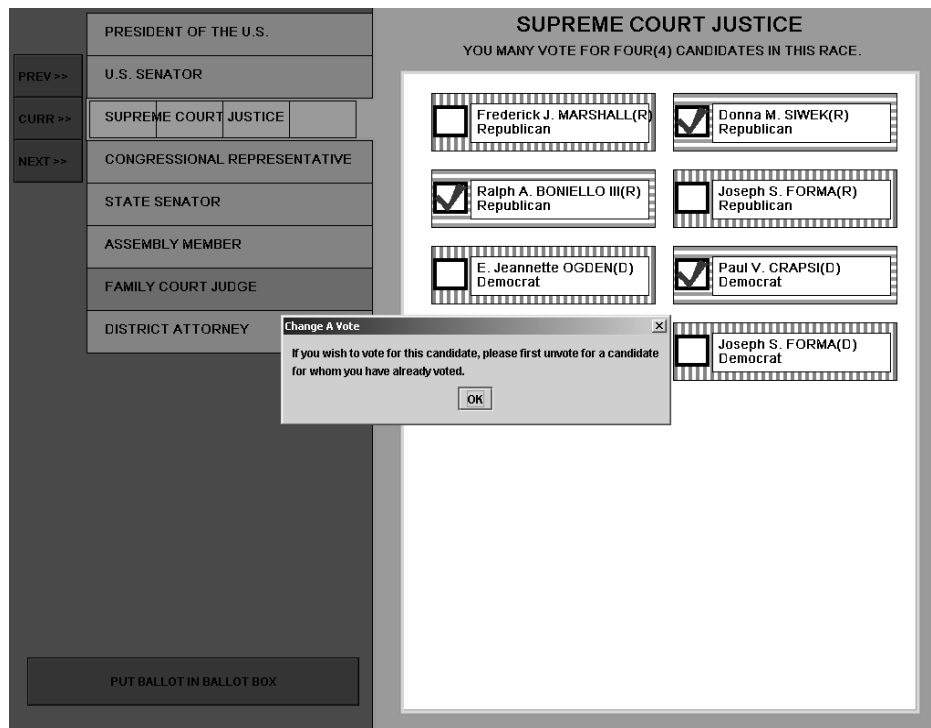
Figure 5.3: Overvoting prevented
