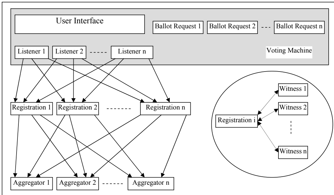
Figure 3.1: SAVE System
