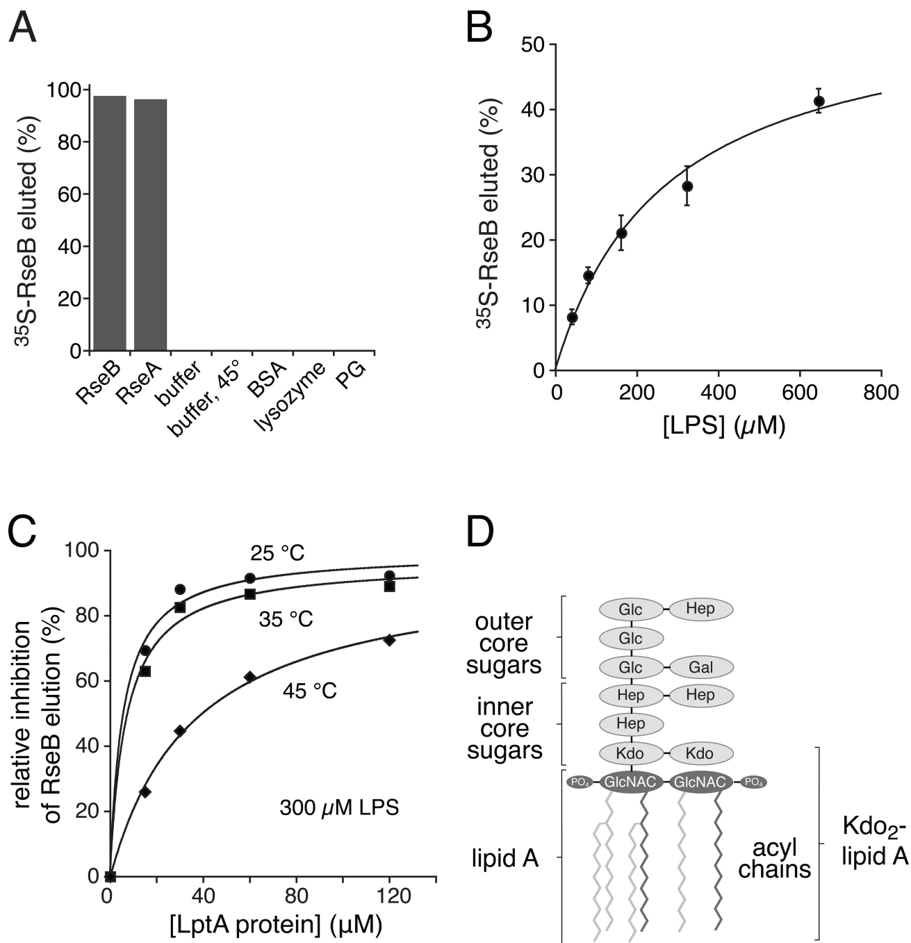
Fig. 1. LPS displaces RseA from RseB. (A) RseB (35 \mu\text{M} ) and RseA P (100 \mu\text{M} ) eluted ^{35}\text{S} -RseB (~1 \mu\text{M} ) from RseA P -agarose, whereas buffer controls, albumin (BSA; 125 \mu\text{M} ), lysozyme (125 \mu\text{M} ), or phosphatidylglycerol (PG; 13 mM) did not. (B) LPS from E. coli K12 eluted ^{35}\text{S} -RseB from RseA P -agarose (25 °C). Data (mean \pm SD; N=3 ) were fit to a hyperbolic function ( K_{\text{app}} = 270 \mu\text{M} ). (C) LptA inhibition of RseB elution by LPS (300 \mu\text{M} ) was more efficient at lower temperatures. (D) Structure of E. coli K12 LPS (GlcNAC, N-acetylglucosamine; Kdo, keto-deoxyoctulosonate; Hep, heptose; Gal, galactose; Glc, glucose). We show that the dark gray elements mediate RseB binding.
