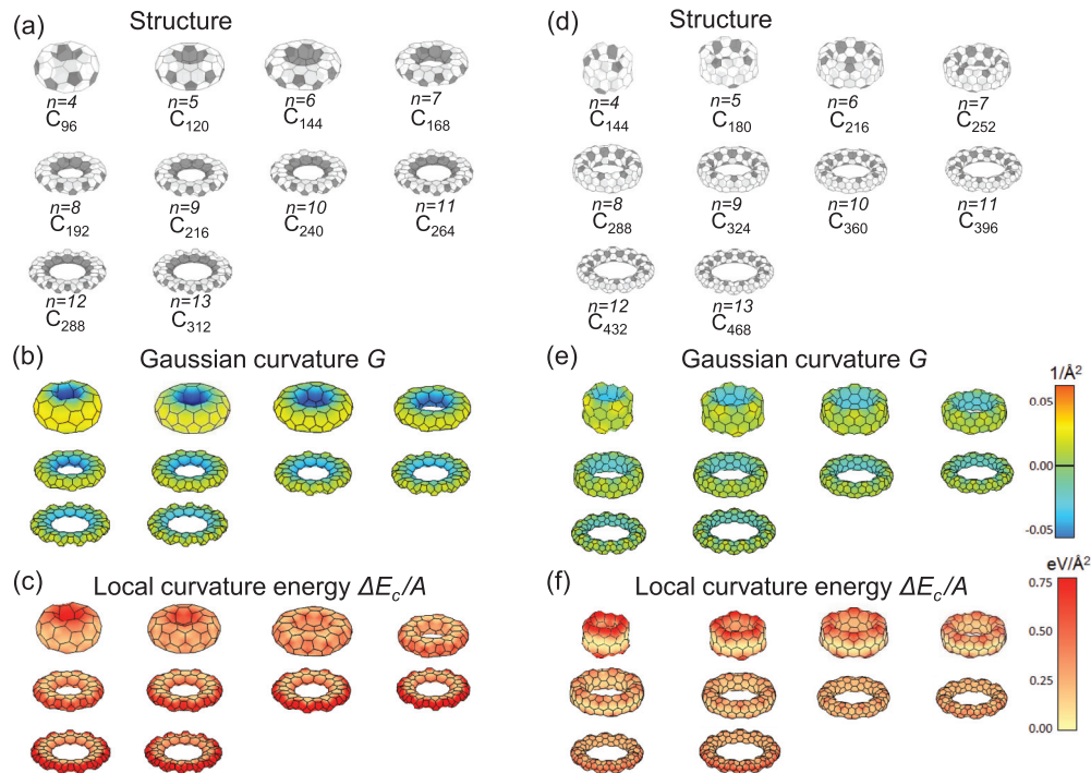
FIG. 9. (Color online) [(a) and (d)] Structural models, [(b) and (e)] local Gaussian curvature G , and [(c) and (f)] local curvature energy \Delta E_c/A across the surface of torus isomers with different rotational symmetry numbers n , defined in Fig. 6(a). Structures in [(a) and (c)] and [(d) and (f)] represent two distinct torus families. The nonhexagonal rings in (a) and (d) are shaded. The values of G and \Delta E_c/A have been interpolated from their values at the atomic sites.
