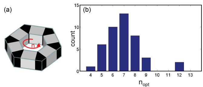
FIG. 10. (Color online) (a) A schematic model of a polygonal nanotorus with an n -fold ( n = 6 in this case) symmetry. (b) Distribution of the optimal rotational symmetry numbers n_{opt} in the 43 families of polygonal nanotori covered in this study.
