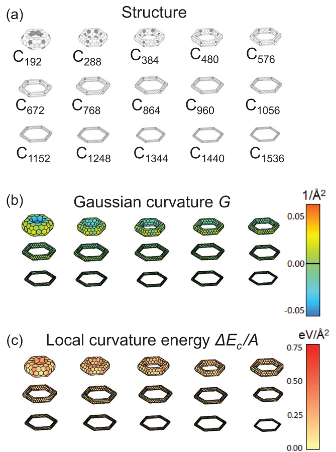
FIG. 7. (Color online) (a) Structural models, (b) local Gaussian curvature G , and (c) local curvature energy \Delta E_c/A across the surface of torus isomers with different lengths of the nanotube segments L , defined in Fig. 6(a). The nonhexagonal rings in (a) are shaded. The values of G and \Delta E_c/A have been interpolated from their values at the atomic sites.
