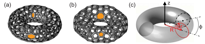
FIG. 1. (Color online) Atomic structure of (a) a polyhex nanotorus with only hexagons and (b) a polygonal nanotorus containing nonhexagonal rings. (c) A model of a perfect torus with major radius R and minor radius r . \theta is the longitudinal angle and \phi is the azimuthal angle. The yellow shading in (a) and (b) indicates specific polygons in the nanotori.
