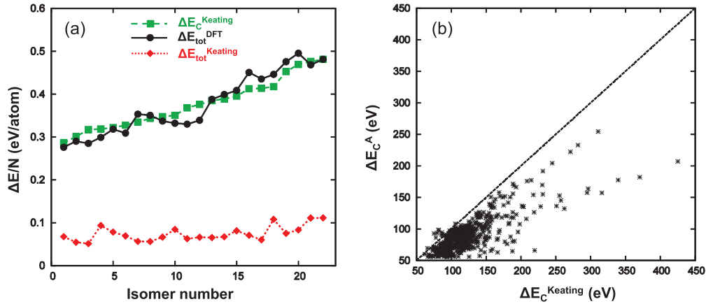
FIG. 4. (Color online) Strain energy \Delta E in different polygonal nanotori. (a) Energy differences per atom \Delta E_{\text{tot}}^{\text{DFT}} based on DFT and \Delta E_{\text{tot}}^{\text{Keating}} based on the Keating potential are presented next to curvature energies \Delta E_c^{\text{Keating}} based on Eq. (2) for Keating-optimized geometries, described in more detail in the text. (b) Comparison between the analytical expression in Eq. (11) for the curvature energy \Delta E_c^A based on the elastic description of a parametric torus and the curvature energy \Delta E_c^{\text{Keating}} obtained using Eq. (2) for Keating-optimized discrete torus geometries.
