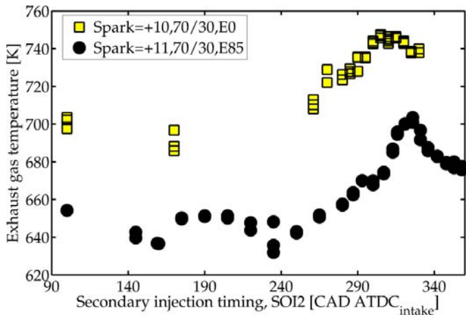
Figure 17: Exhaust temperature as a function of SOI2 for E0 and E85 fuels at NIMEP = 2 bar.
