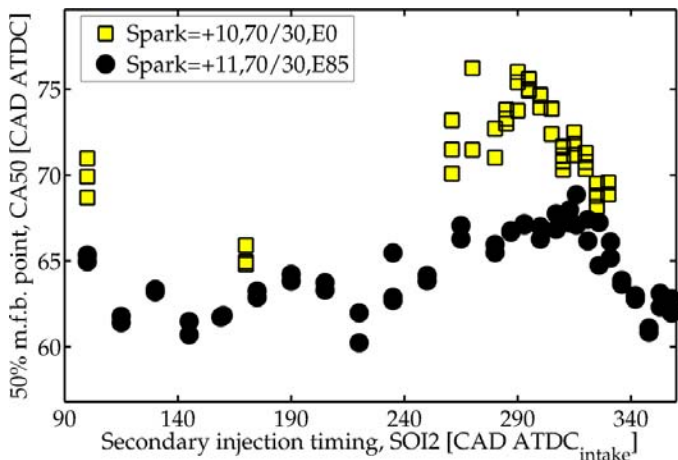
Figure 18: CA50 versus SOI2 for E0 and E85 fuels at NIMEP = 2 bar.
