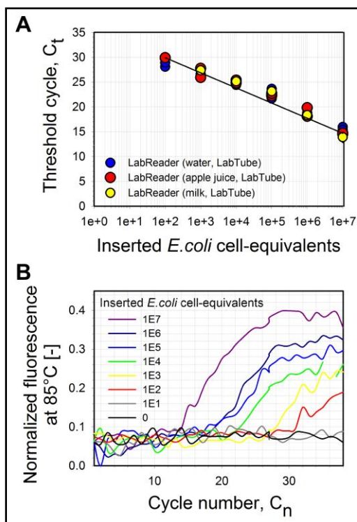
Fig. 4 E. coli PCR in the LabReader using the intercalating dye SYTOX Orange with readout at 85°C above the melting point of nonspecific products (A) The calibration curve no longer shows false positive signals below 100 cell-equivalents. (B) Reaction curves for different copy numbers of genomic E. coli DNA in water (effective fluorescence vs. cycle number). Normalized fluorescence is the difference in fluorescence signal between 85°C and 95°C divided by the difference in fluorescence signal between 62°C and 95°C at each cycle number.
