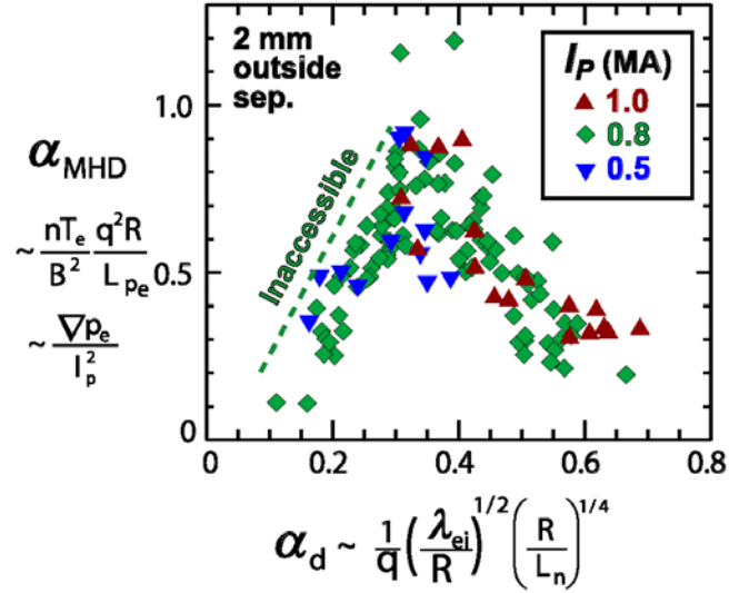
Fig. 14. The normalized pressure gradient ( \alpha_{\text{MHD}} ) in the near-SOL depends strongly on collisionality. \alpha_d is the inverse normalized collisionality as defined in Rogers 1998 PRL.
