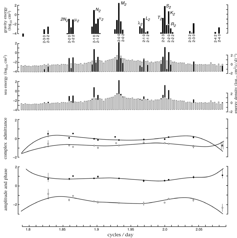
FIGURE 7. Same as Fig. 6 except for the semi-diurnal band (notice the different frequency scales in the two figures). See the text for explanation of the panels.
