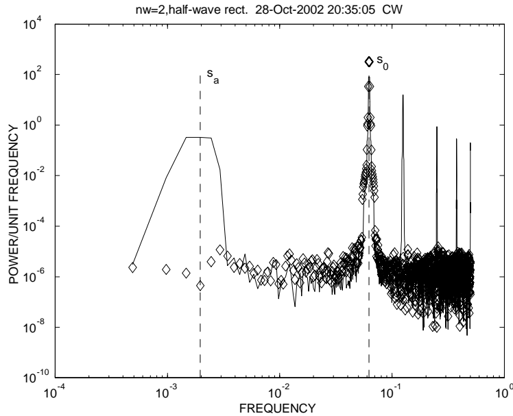
FIGURE 8. Diamonds are the power density spectrum of the original modulated carrier wave Eq. (7.3) plus a small amount of white noise. There is no excess energy at the modulation period 1/s_a . Solid line is a power density spectral estimate of the signal, from the half-wave rectifier. Now excess energy appears at period 1/s_a as well as at the periods of all the harmonics of s_0 .
