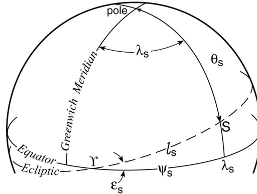
FIGURE 3. Latitude and longitude of the subsolar point in Greenwich coordinates (\lambda_s, \theta_s) . Angles l_s, \psi_s are measured from the vernal equinox \Upsilon . (Adapted from Munk and Cartwright, 1966).
