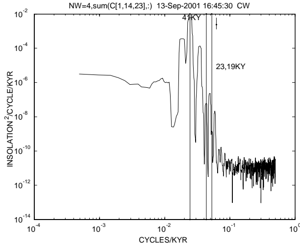
FIGURE 5. Power density spectrum of the long period terms in insolation, Eq. (6.2) from a calculation of duration 2 MY sampled at intervals of 1KY. Vertical lines show the dominant obliquity period of 41KY and the two main precessional terms at 23 and 19KYR. The latter are essentially absent in a year-long average. The eccentricity term at 100KY is very small. (From a time series of B. Bills, 2001)
