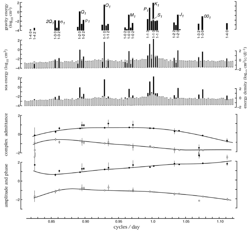
FIGURE 6. From Munk and Cartwright (1966) showing the diurnal band frequencies separable at one cycle/year as well as an analysis of the behavior of the tides at Honolulu (see the text). None of the frequencies lies very far from 1 cycle/lunar or solar day.
