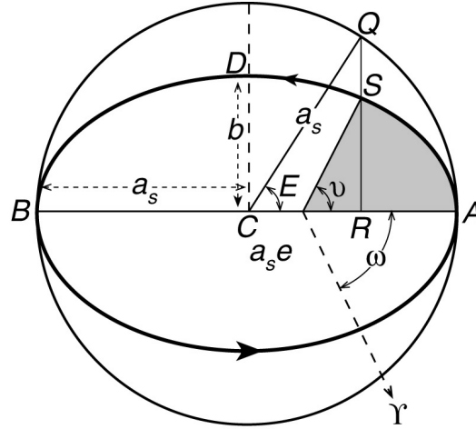
FIGURE 4. Geometry of a body at S moving in an exaggerated ellipse about the earth at a focus. \nu is the true anomaly of the body (the sun), E measured relative to the center of the ellipse is the eccentric anomaly. \omega defines the angle between the vernal equinox \Upsilon and perihelion. a_s , b are the semi-major and minor axes of the ellipse, and a_s is also the radius of the bounding circle. \nu , E , M (the solar anomalies) are all measured from perigee. M is the angle of the position of the fictitious mean sun moving uniformly along the circle.
