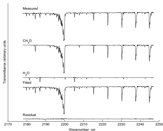
Figure 2. A typical spectral fit in the region where ^{12}\text{CH}_3\text{D} is obtained (Experiment 5). Experimental data are shown by the topmost line, followed by the fitted (synthetic) partial spectra of the most dominant absorbers ( \text{CH}_3\text{D} and \text{H}_2\text{O} ), the resulting fitted (synthetic) spectrum (also including \text{CO}_2 and \text{CO} ), and the residual between the measured and fitted spectra.
