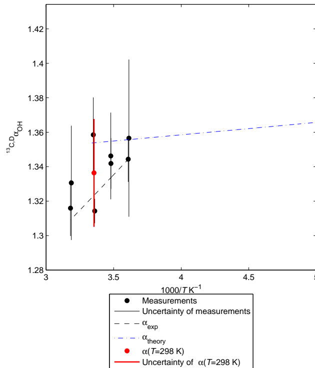
Figure 6. The individual measurements of ^{13}\text{C}_3\text{H}_3\text{D}\alpha are represented by black points, the accompanying individual error bars are represented by thin black solid lines, the experimental Arrhenius curve fit is represented by a black dashed line, the theoretical Arrhenius curve fit is represented by a blue dashed-dotted line, the mean of the room temperature measurements is represented by a red solid circle, and the uncertainty of the room temperature measurements is represented by a thick red solid line. All uncertainties are given as 1 standard deviation ( \sigma ).
