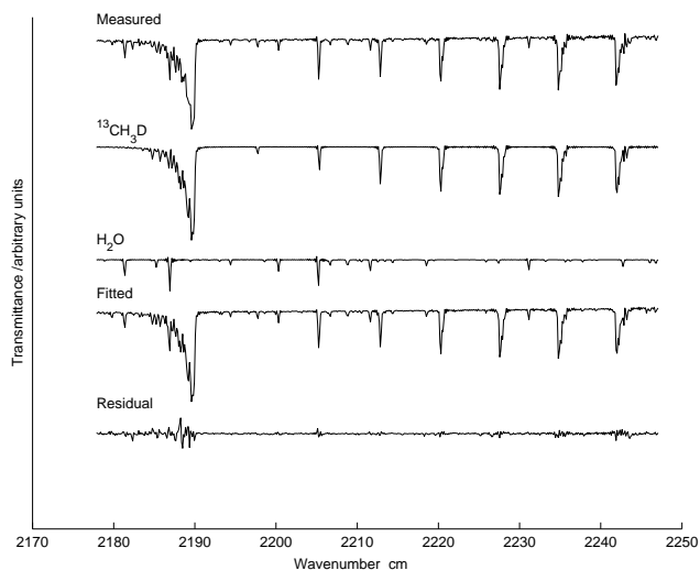
Figure 1. A typical spectral fit in the region where ^{13}\text{CH}_3\text{D} is obtained (Experiment 10). Experimental data are shown by the topmost line, followed by the fitted (synthetic) partial spectra of the most dominant absorbers ( ^{13}\text{CH}_3\text{D} and \text{H}_2\text{O} ), the resulting fitted (synthetic) spectrum (also including \text{CO}_2 and \text{CO} ), and the residual between the measured and fitted spectra.
