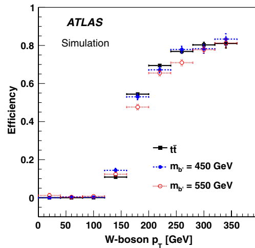
FIG. 3 (color online). The efficiency for jet pairs from a simulated W boson decay to have \Delta R < 1.0 and a dijet mass within 70–100 GeV, for simulated t\bar{t} and signal events. Events are required to have exactly six jets.
