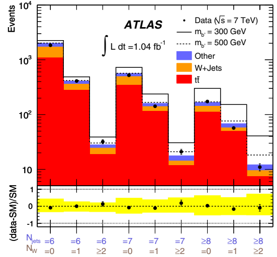
FIG. 4 (color online). Distribution of the numbers of events observed in the data and expected from SM processes for jet multiplicity N_{\text{jets}} = 6, 7, \geq 8 with hadronic W multiplicity N_W = 0, 1, \geq 2 . The expected b' signals for two masses are also shown, stacked on top of the backgrounds.
