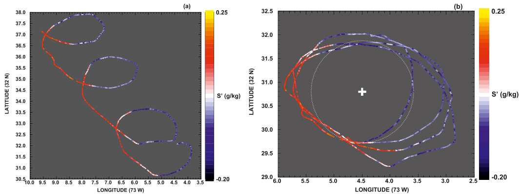
FIG. 6. Representative site 2 transformation from (left) Eulerian to (right) Lagrangian coordinates using the drogue Gateway buoy to center the Lagrangian coordinates ( U = -0.25 \text{ m s}^{-1} and V = 0.45 \text{ m s}^{-1} ). This example shows the Hammerhead tow-yo path for its 14 Jun deployment.
