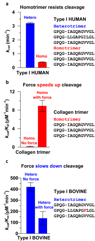
Figure 1. Comparisons of the cleavage rates between the heterotrimer and the homotrimer without and with applying forces
