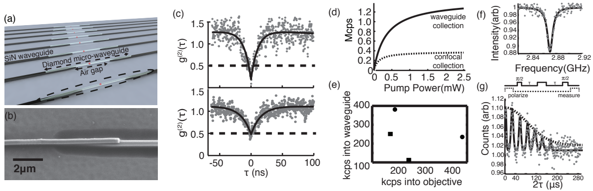
Fig. 1. Demonstration of a PIC with NV emission efficiently collected into a SiN waveguide a) Schematic of a PIC with multiple integrated quantum memory nodes. b) Scanning electron micrograph of a diamond waveguide placed over a gap in a SiN waveguide. c) normalized auto-correlation via confocal collection (top) and normalized cross-correlation (bottom) measurements of one integrated quantum node confirming single photon emission into the waveguide. d) Saturation measurements corrected for background and collection losses. e) Counts collected into a free space objective vs. counts collected into the single mode SiN waveguide for 4 integrated NV centers at 125uW of excitation. Circles are calculated from saturation curves, and squares are measured. f) ODMR of an integrated NV under no magnetic field with waveguide collection. g) A Hahn-Echo measurement to decouple the NV from the surrounding spin bath and measure T_2 > 120 \mu\text{s} .
