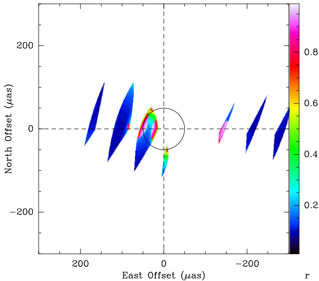
Figure 4. Offsets between two point sources that would produce closure phases between +0.9^\circ and +14.9^\circ at all triangles of (u,v) coordinates sampled by our data. For a unit point source centered at the origin, the colored regions indicate the allowed offset of a second point source, with color indicating the maximum value of r within the range 0 < r < 1 . The circle shows an offset of 50 \mu\text{as} , which is approximately the diameter of the predicted shadow in Sgr A*. For two components separated by the shadow diameter, a roughly east-west alignment with the brighter component to the west is required to be consistent with our data.
