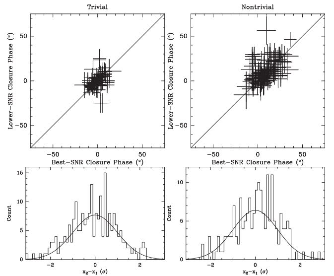
Figure 1. Consistency checks. Top: multiple processings of the same trivial (left) and nontrivial (right) closure phases are consistent with much less than the thermal noise. Bottom: pairwise differences of similar data points (as defined in Section 3.2) are consistent with being drawn from a Gaussian random distribution characterized by their error bars, confirming that the error estimates are not biased.
