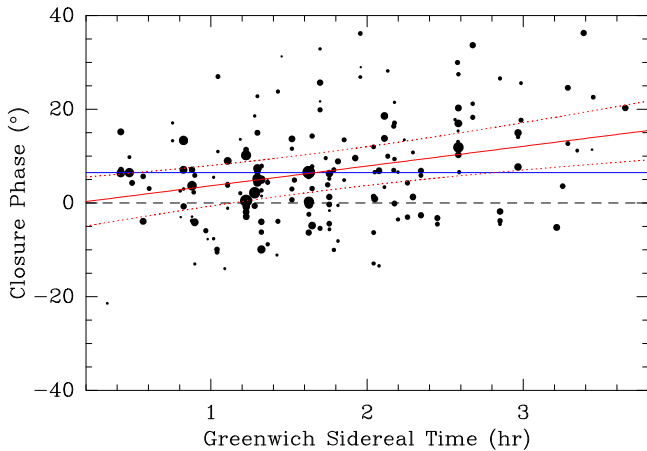
Figure 3. Measured closure phases (dot diameter proportional to S/N) plotted against GST. The solid red line shows the best-fit line, with the dashed red lines showing the \pm 3\sigma range. The solid blue line shows the best-fit line with zero slope. Despite the large scatter, the data suggest that the California–Hawaii–Arizona closure phase may be increasing with GST.
