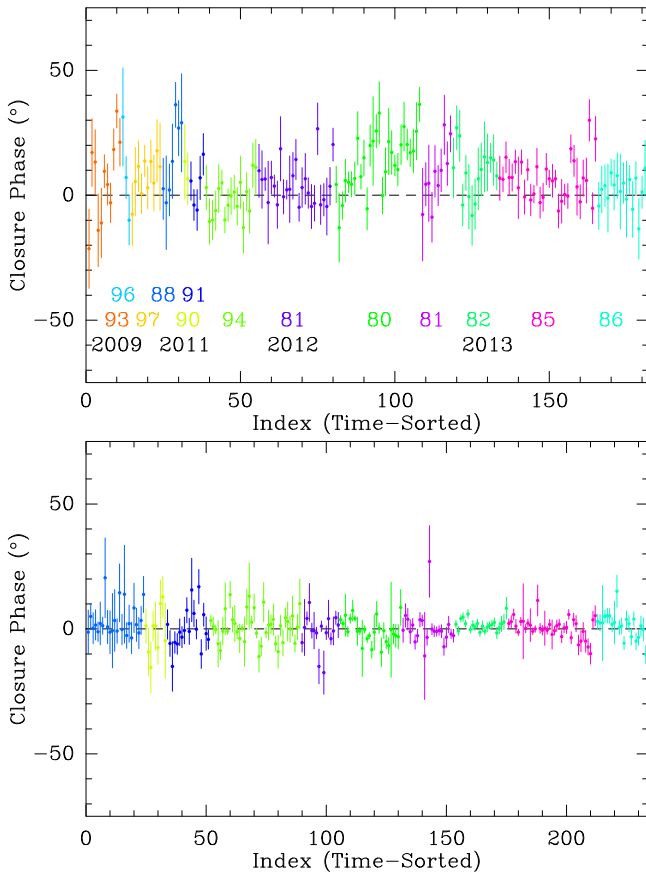
Figure 2. Top: all 181 nontrivial California–Hawaii–Arizona closure phases measured on Sgr A*. Data are presented in time order and are color-coded by day and year. The median nontrivial closure phase is +6^{\circ}.3 . Bottom: the 233 trivivial closure phases for Sgr A*, excluding data from 2009 (Section 2.1.1). The median trivivial closure phase is consistent with zero, as expected.
