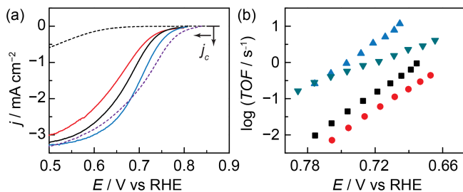
Figure 3. (a) Linear sweep voltammograms (5 mV/s scan rate) of 1 (black), 2 (red), 3 (blue), 3'-treated Monarch 1300 (dotted purple) and unmodified GC (dotted black) recorded in O 2 saturated 0.1 M KOH electrolyte. Data were recorded at 2000 RPM and current densities are normalized to the geometric electrode area. (b) Tafel plots of per site activity versus applied potential for 1 (black), 2 (red), 3 (blue) and Ag (green).
