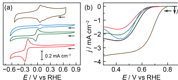
Figure 4. (a) Cyclic voltammograms of pyrazine (red), quinoxaline-6-carboxylic acid (green), dibenzo[a,c]phenazine-2-carboxylic acid (blue) and 4 (brown) recorded in N 2 -saturated 0.1 M KOH. (b) Linear sweep voltammograms of a freshly polished GC disk electrode rotated at 2000 RPM and recorded in O 2 -saturated 0.1 M KOH electrolyte containing 5 mM pyrazine (red), 5 mM quinoxaline-6-carboxylic acid (green), 1 mM dibenzo[a,c]phenazine-2-carboxylic acid (blue),
