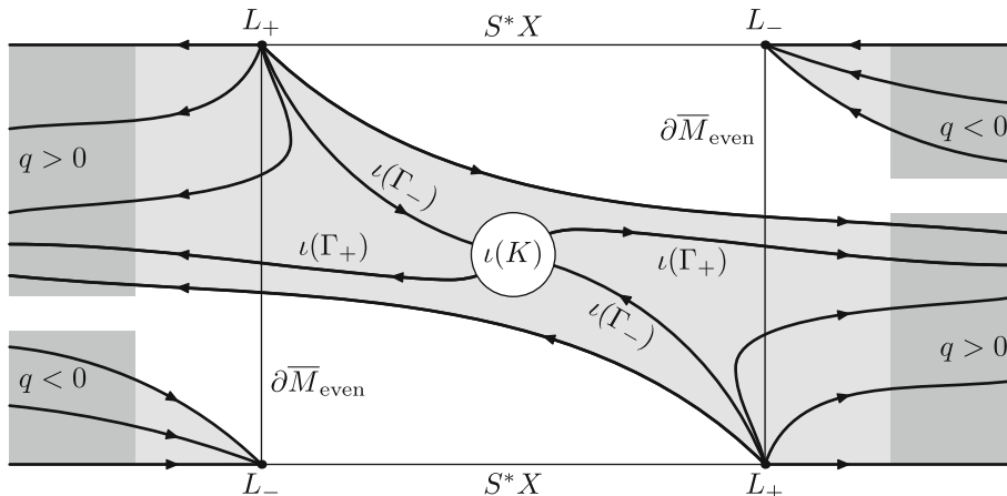
Figure 2: A schematic presentation of the dynamical complexity for the hyperbolic cylinder M = (-1, 1)_r \times \mathbb{S}^1_{\tilde{y}} . Here \iota(K) denotes the trapped set, which connects to infinity through the incoming and outgoing tails \iota(\Gamma_{\pm}) . The vertical lines \partial\bar{M}_{\text{even}} correspond to the two funnel ends \{r = \pm 1\} ; the horizontal variable is r and the vertical variable is the compactification \zeta/\langle\zeta\rangle of the momentum \zeta dual to r . The lighter shaded regions are the components \Sigma_{\pm} of the energy surface, with \Sigma_+ the bigger region and \Sigma_- the union of two small ones. The darker shaded regions are the sets where the complex absorbing operator Q is elliptic. See Appendix B for more details
