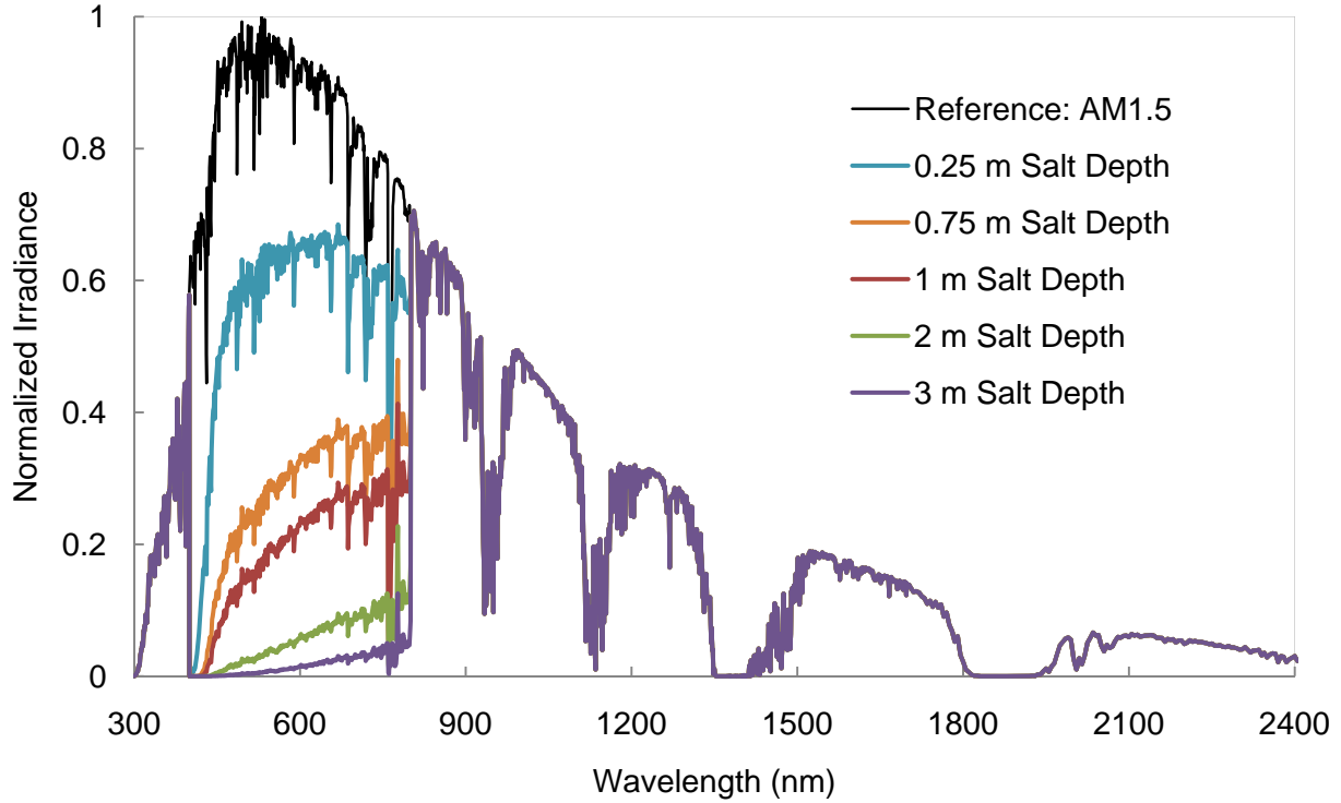
Fig. 6. Solar irradiance attenuation for different molten salt depths. This figure was produced using experimentally measured attenuation coefficients for a 60/40 wt% sodium-potassium nitrate mixture at 350°C in the wavelength range of 400-800 nm, the range where experimental measurements are possible.
