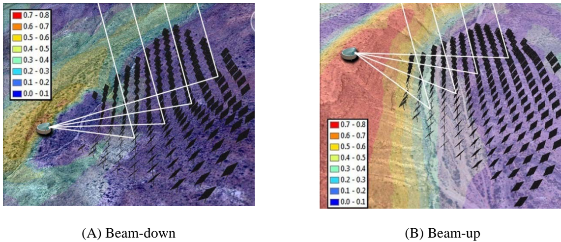
Fig. 1. Representative CSPonD sites in White Sands, NM for pond receiver without (A) and with (B) secondary reflector. The CSPonD system simultaneously collects sunlight while also acting as the beam-down optic thereby reducing overall system complexity and cost. Icons illustrate receiver location and discretized terrain sampling locations from elevation data, not an actual heliostat layout. See Noone et al. (2011).
