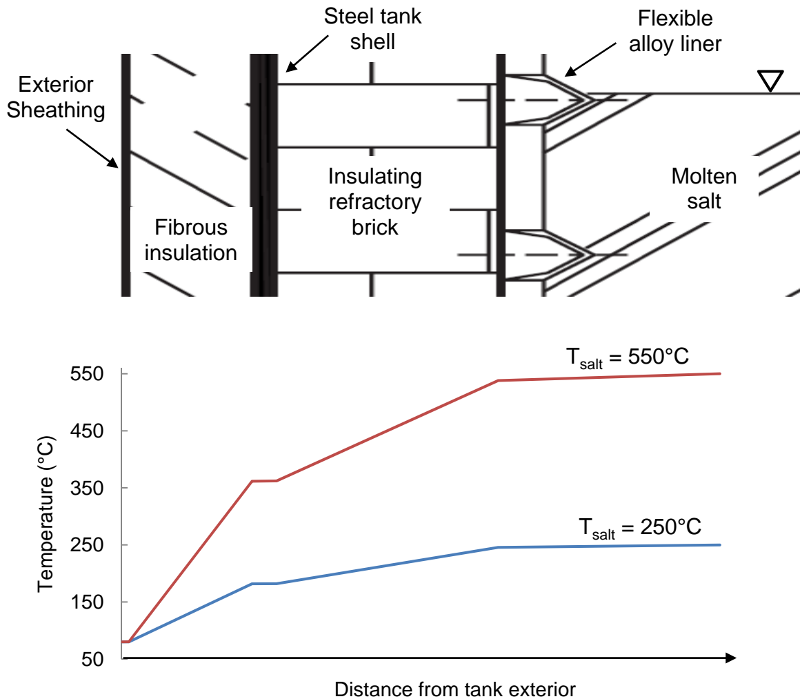
Fig. 4. Tank wall insulation schematic. Internal insulating refractory brick is used to reduce temperature fluctuations at the tank shell. A thin, thermally conductive alloy liner can be employed to reduce axial thermal gradients and shock. Cross-section adapted from Kolb (1993) and Gabbrielli and Zamparelli (2009).
