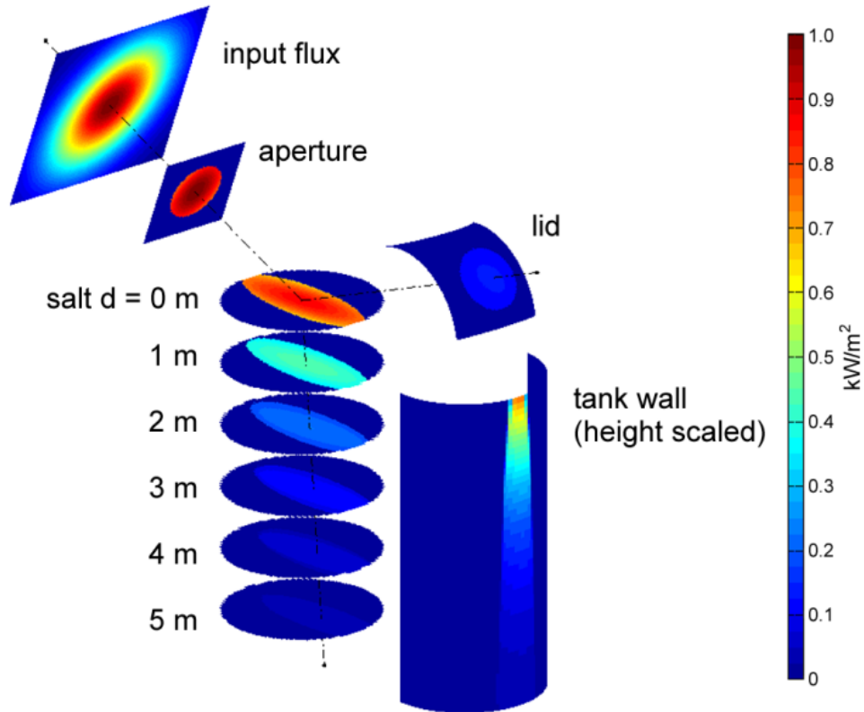
Fig. 7. Representative solar irradiance distribution for a single heliostat aimed at a CSPonD receiver. A complete heliostat field can be aimed to create a circular illumination distribution on the salt surface.
