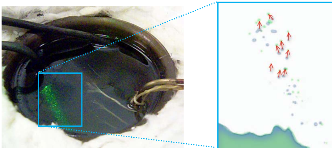
Fig. 9. Molten salt convection cell monitoring using PIV. Notice that there are particles in the molten salt that reflect light which can be used to determine fluid movement within the receiver. The inset on the right is composed of two consecutive time frames (blue and green). The arrows show particles that have shifted from frame-to-frame; these can be used to characterize fluid movement.
