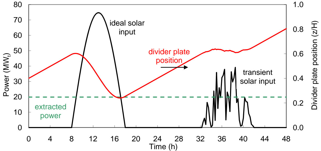
Fig. 3. Simplified divider plate position example for two day/night cycles: Ideal solar input (left) and transient, or cloudy, solar input (right) for a constant 20\text{MW}_t extraction system.
