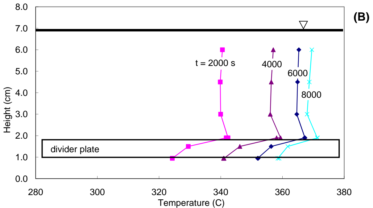
Fig. 8. Temperature distribution of CSPonD receiver optically heated by the 10.5 kW MIT CSP Solar Simulator; inset depicts stainless steel (type 316L, 28 cm inner diameter x 8 cm high, 7 L solar salt capacity) test receiver. The movable divider plate (3.2 mm thick stainless steel disc with a 6.4 mm thick layer of rigid silica insulation board affixed to the underside) and is denoted by the shaded grey box located near the salt surface (A) and tank bottom (B) of the test receiver.
