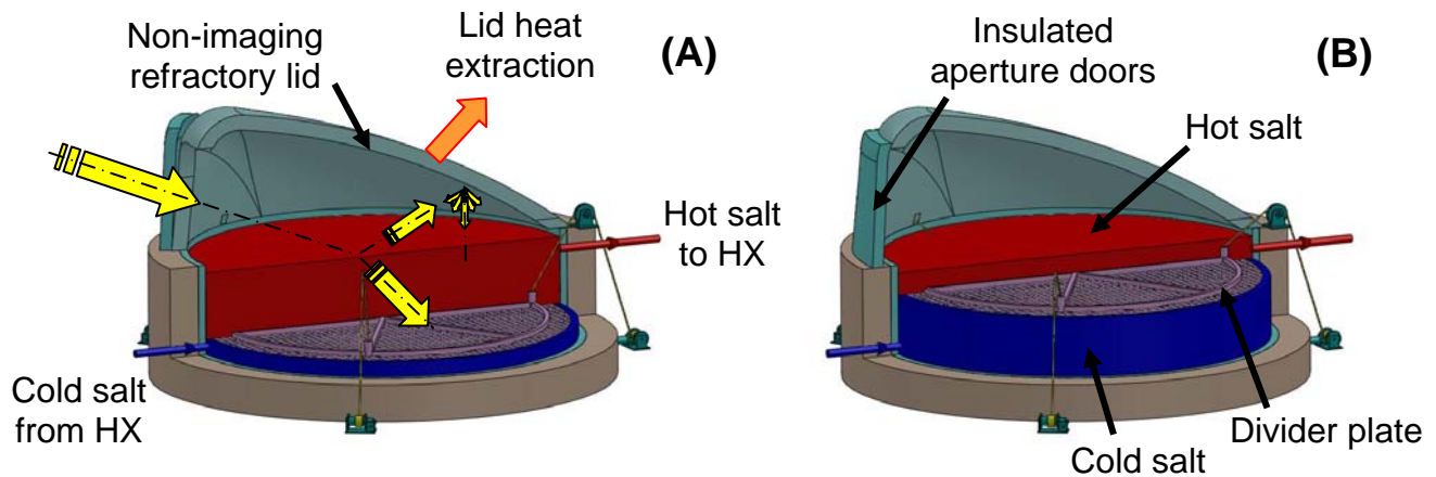
Fig. 2. Cross sections of a CSPonD volumetric absorption molten salt receiver/storage system: (A) Yellow arrows denote light path within receiver. At end of a sunny day the divider plate has moved down and the hot salt region is fully charged. (B) Whereas after prolonged heat extraction without solar input, the divider plate has moved up and the cold side is full. Hot molten salt is pumped as needed from the top of the tank to provide reasonably constant power and temperature input to a steam generator or other power cycle. Colder, yet still liquid salt from the steam generator is returned to the bottom of the tank.
