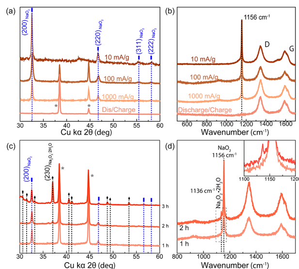
Figure 2. (a) XRD patterns and (b) Raman spectra for the CNT electrodes discharged at 10, 100, and 1000 \text{mA g}^{-1} to 1000 \text{mAh g}^{-1} (corresponding discharge profiles shown in Figure 1a) and after being discharged and fully charged at 1000 \text{mA g}^{-1} to 1000 \text{mAh g}^{-1} in 0.1 M \text{NaClO}_4 in DME. D and G bands of the CNTs and the \text{NaO}_2 peak at 1156 \text{ cm}^{-1} are indicated in the Raman spectra. (c) XRD patterns of a CNT electrode discharged at 1000 \text{mA g}^{-1} to 2000 \text{mAh g}^{-1} in 0.1 M \text{NaClO}_4 in DME, showing the conversion to \text{Na}_2\text{O}_2 \cdot 2\text{H}_2\text{O} (black dashed lines) from \text{NaO}_2 (blue dashed lines) in the XRD holder after 1, 2, and 3 h at ambient. The CNT electrodes were extracted from the \text{Na}-\text{O}_2 cell immediately after discharge in an argon-filled glovebox and sealed in an airtight XRD sample holder (Anton Paar, Graz, Austria). The first diffractogram (labeled 1 h) was collected immediately after 1 h of cell discharge. Subsequent diffractograms (2 h and 3 h) were collected sequentially, each with a collection time of 1 h. (d) Raman spectra of a CNT electrode discharged at 1000 \text{mA g}^{-1} to 2000 \text{mAh g}^{-1} in 0.1 M \text{NaClO}_4 in DME taken immediately after discharge (labeled 1 h) and after 1 h of exposure to air (labeled 2 h), showing evolution of \text{Na}_2\text{O}_2 \cdot 2\text{H}_2\text{O} ( 1136 \text{ cm}^{-1} ) from \text{NaO}_2 ( 1156 \text{ cm}^{-1} ).
