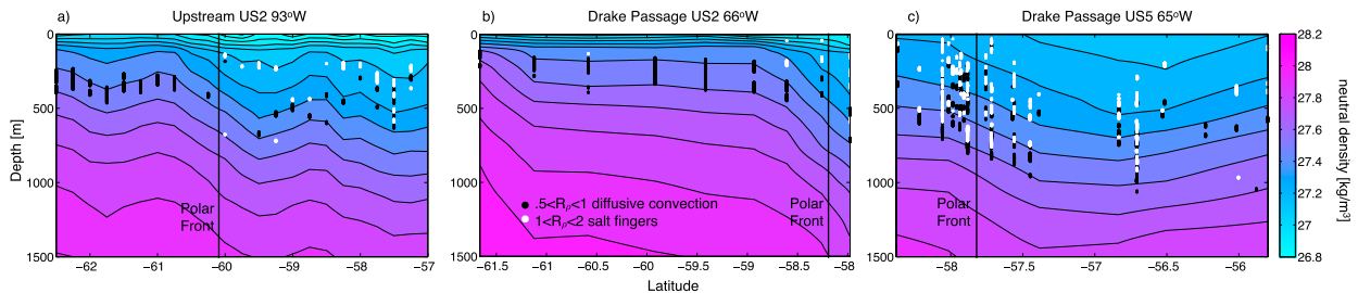
FIG. 6. Three meridional transects of neutral density (colors) at (a) 93°W, (b) 66°W, and (c) 65°W. The circles represent regions in the water column where the density ratio R_\rho is between 0.5 and 1 (black) and 1 and 2 (white). These ranges represent potential for double-diffusive instabilities with growth rates comparable to the buoyancy frequency ( N ), the time scale associated with internal-wave-driven turbulence. The density ratio is preferable to double-diffusive instability in neutral density classes between 27.2 and 27.7 \text{kg m}^{-3} . The PF in each panel is defined by the hydrographic measurements made during the respective cruises, (a),(b) US2 and (c)US5.
