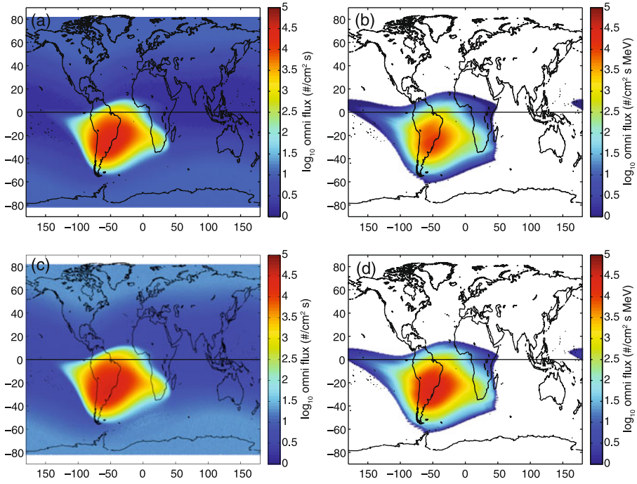
Fig. 11 Median (a) and 95th percentile (c) >36 MeV flux maps constructed from 13 years of POES N15/SEM data. Similar median (b) and 95th percentile maps (d) determined from 40 MC AP9 scenarios of 3.5 years duration each
