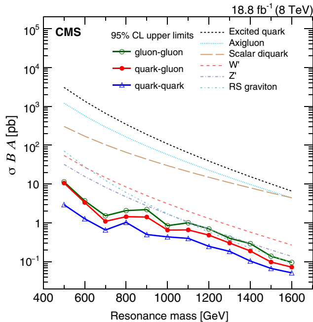
FIG. 3. Observed 95% CL upper limits on \sigma\mathcal{B}A for a narrow resonance decaying to gluon-gluon final states (open circles), quark-gluon final states (solid circles), and quark-quark final states (open triangles) compared with theoretical predictions for various resonance models.
