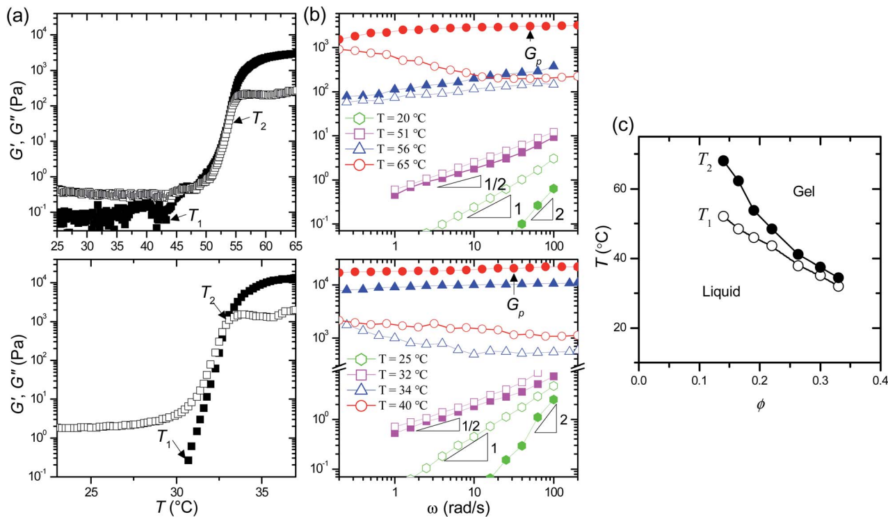
Fig. 1 Rheological characterization of nanoemulsions with (a) = 18 nm containing (top) \phi = 0.22 and (bottom) \phi = 0.33 . (a) Thermal scans of elastic modulus G' (closed symbols) and viscous modulus G'' (open symbols) versus temperature, indicating the apparent gel temperatures T_1 and T_2 . (b) Frequency sweeps of G' and G'' versus oscillatory frequency for the temperatures indicated in the linear viscoelastic regime ( \gamma_0 = 0.05\% ). (c) Colloidal phase diagram for nanoemulsions containing droplets with (a) = 18 nm. Points give the apparent gel temperatures corresponding to panel (a).
