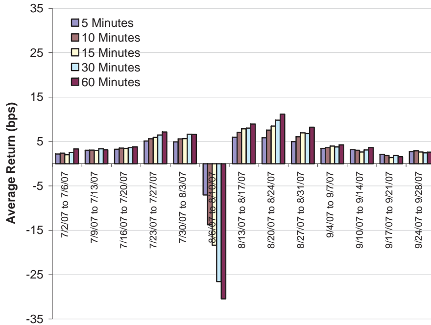
Figure 10: The average return for the contrarian strategy applied to 5-minute returns from July 2, 2007 to September 28, 2007. Each day is divided into non-overlapping 5-minute intervals, and positions are established based on lagged 5-minute returns and then held for 5, 10, 15, 30, or 60 minutes. The average return for each holding period is calculated for each week during this sample. No overnight positions are allowed, initial positions are established at 9:40am each day and all positions are closed at 4:00pm. Components of the S&P 1500 are based on memberships as of the last day of the previous month.
