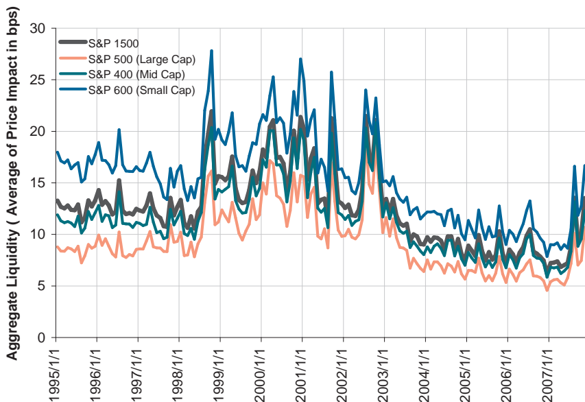
Figure 7: Monthly cross-sectional averages of price impact coefficients \hat{\lambda}_i of stocks in the S&P 1500 and sub-components between January 1995 and December 2007, based on daily time-series regressions for each stock i within each month: R_{i,t} = \hat{c}_i + \hat{\lambda}_i \cdot \text{Sgn}(t) \log(v_{i,t}p_{i,t}) + \epsilon_{i,t} where \text{Sgn}(t) \log(v_{i,t}p_{i,t}) is the signed volume of security i on date t and the sign is determined by “tick test” applied to daily returns. Components of these indexes are based on the memberships on the last day of the previous month.
