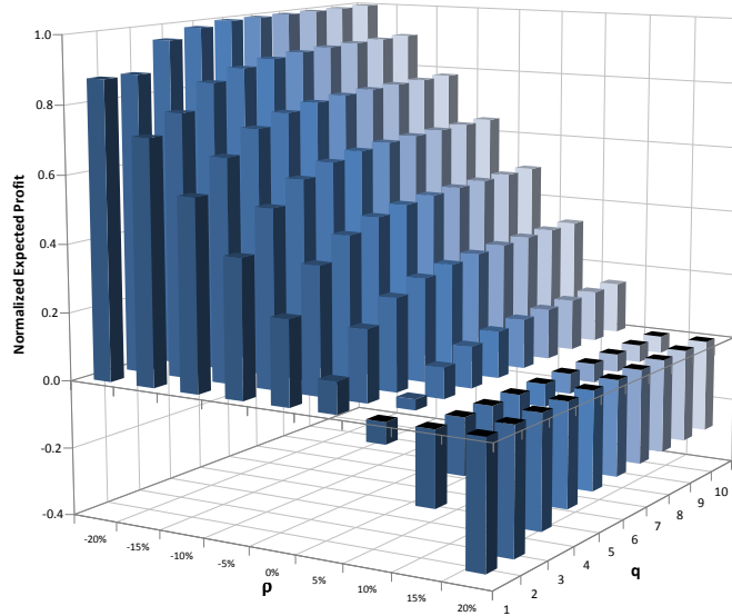
Figure 5: Plot of the normalized expected profit of the contrarian strategy, \frac{1-\theta^q}{2} - \rho \frac{1-\rho^q}{1-\rho} \frac{\sigma_\beta^2}{\sigma_\lambda^2} \sigma^2(\boldsymbol{\beta}) , for parameter values \frac{\sigma_\beta^2}{\sigma_\lambda^2} = 50 , \sigma^2(\boldsymbol{\beta}) = 1/16 , and \theta = 1/2 , as a function of the serial correlation coefficient of the common factor, \rho , and the holding period q .
