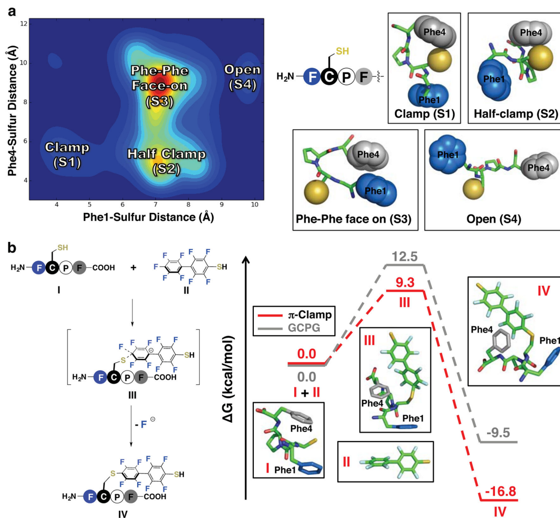
Figure 6. Structure and mechanism of the \pi -clamp
