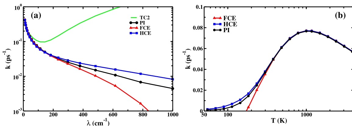
FIG. 3. (a) Energy transfer rates between two symmetric two level systems as a function of the reorganization energy. The cutoff frequency is \gamma = 53 \text{ cm}^{-1} and the temperature is T = 300 K. The black dots, green lines, red triangles, and blue squares denote the results from the present stochastic path integral approach, the TC2 master equation, 13 the FCE, 5,7 and the HCE, 6 respectively. (b) The energy transfer rates as a function of the temperature. The reorganization energy is \lambda = 200 \text{ cm}^{-1} and the cutoff frequency is \gamma = 53 \text{ cm}^{-1} . The results from the TC2 approach lie outside the scale of the graph for all temperatures shown.
