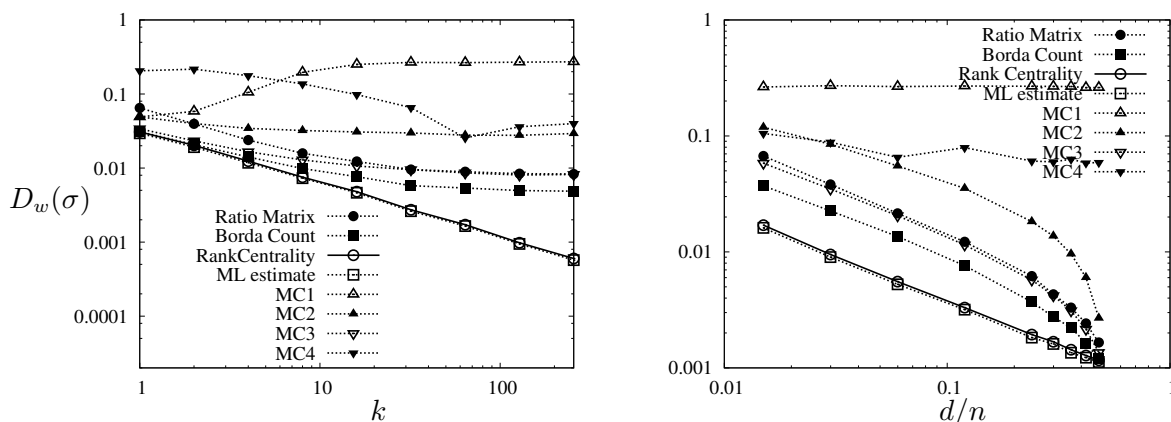
Figure 1 Average error D_w(\sigma) of various rank aggregation algorithms averaged over 20 instances. In the figure on the left, d and n are fixed while k is increased. The figure on the right, keeps k = 32 fixed, and lets d increase.
