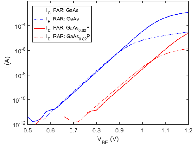
Figure 7: Collector current in the forward-active regime (FAR) and emitter current in the reverse-active regime (RAR) for GaAs/InGaP and GaAs 0.82 P/InGaP HBTs. The emitter-base junction diameter is 60 \mu\text{m} .
