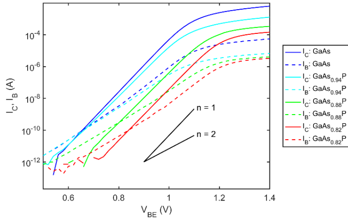
Figure 5: Gummel plots (collector current and base current vs emitter-base voltage) for GaAsP/InGaP HBTs of four different compositions. Measurement was taken with V_{BC} = 0 V.
