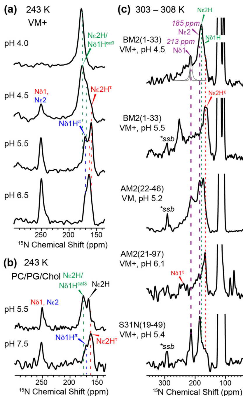
Figure 7. 1D ^{15}\text{N} CP spectra of BM2(1–33) as a function of pH, membrane composition and temperature. (a) Spectra of the VM+ bound BM2 from pH 4.0 to pH 6.5 at 243 K. (b) Spectra of PC/PG/Chol-bound BM2 at pH 5.5 and pH 7.5 at 243 K. (c) Comparison of high-temperature (303 – 308 K) ^{15}\text{N} spectra of BM2 and AM2 at acidic pH. An ^{15}\text{N} exchange peak is detected at \sim 213 ppm at pH 4.5 for BM2, at pH 5.2 for AM2-TM, and at pH 5.4 in the S31N mutant of AM2-TM. The exchange-averaged chemical shifts are the same in all
