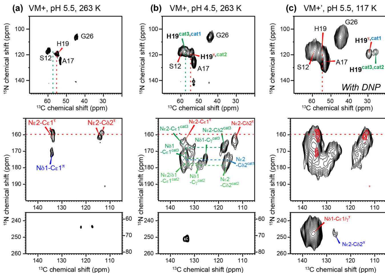
Figure 5. 2D ^{15}\text{N} - ^{13}\text{C} correlation spectra of His19 in BM2(1-33). (a, b) BM2 in the VM+ membrane, measured on an 800 MHz spectrometer with 14.5 kHz MAS at 263 K. (a) pH 5.5. (b) pH 4.5. (c) BM2 at pH 5.5 in the d_{31} -VM+ membrane, measured on a 400 MHz/263 GHz DNP spectrometer under 9 kHz MAS at 117 K. Note the different neutral and cationic histidine distribution between high and low temperatures at pH 5.5, indicating temperature-induced \text{pK}_a shifts.
