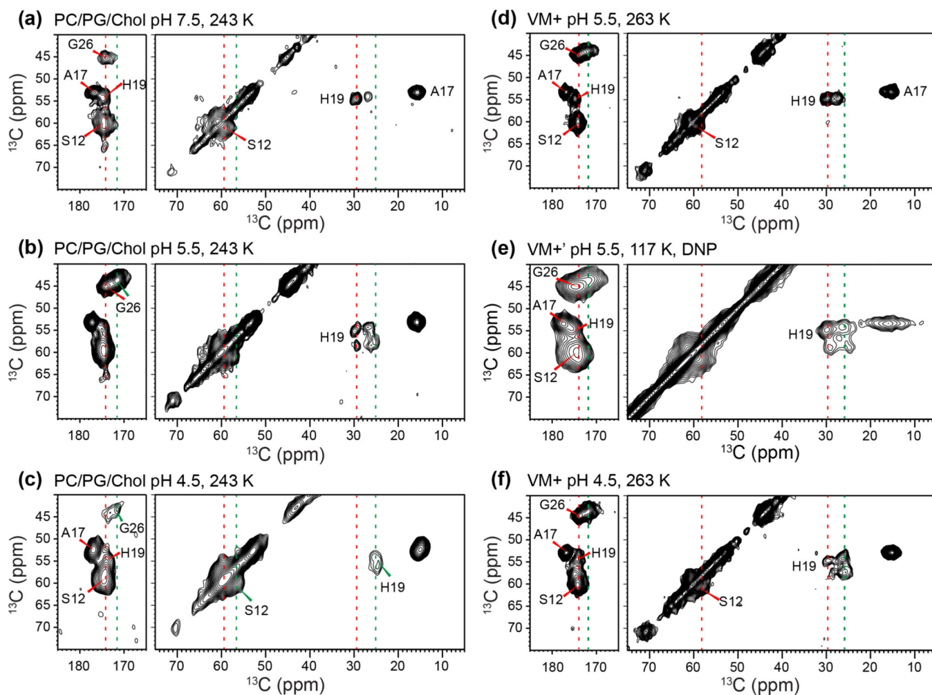
Figure 3. 2D ^{13}\text{C} - ^{13}\text{C} correlation spectra of site-specifically labeled BM2(1–33) in different membranes and at different pH. (a) PC/PG/Chol at pH 7.5. (b) PC/PG/Chol at pH 5.5. (c) PC/PG/Chol at pH 4.5. (d) VM+ membrane at pH 5.5. (e) VM+' membrane at pH 5.5 with DNP. (f) VM+ membrane at pH 4.5.
