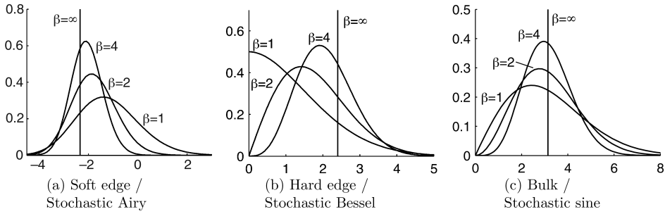
FIGURE 2. Local eigenvalue behavior
