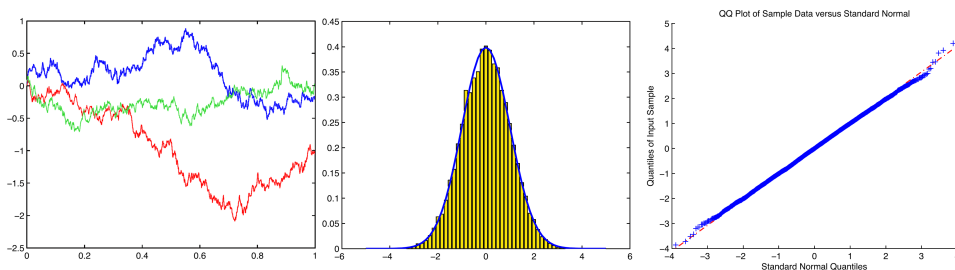
FIGURE 1. Left: Sample paths for standard Brownian motion; Center: histogram of W(1) vs. the pdf of the standard normal; Right: quantile-quantile plot of W(1) .
