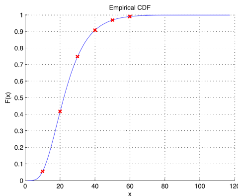
FIGURE 3. The empirical (solid line) and analytic (x's) cdf's of the largest eigenvalue of the general \beta -Wishart Ensemble.
